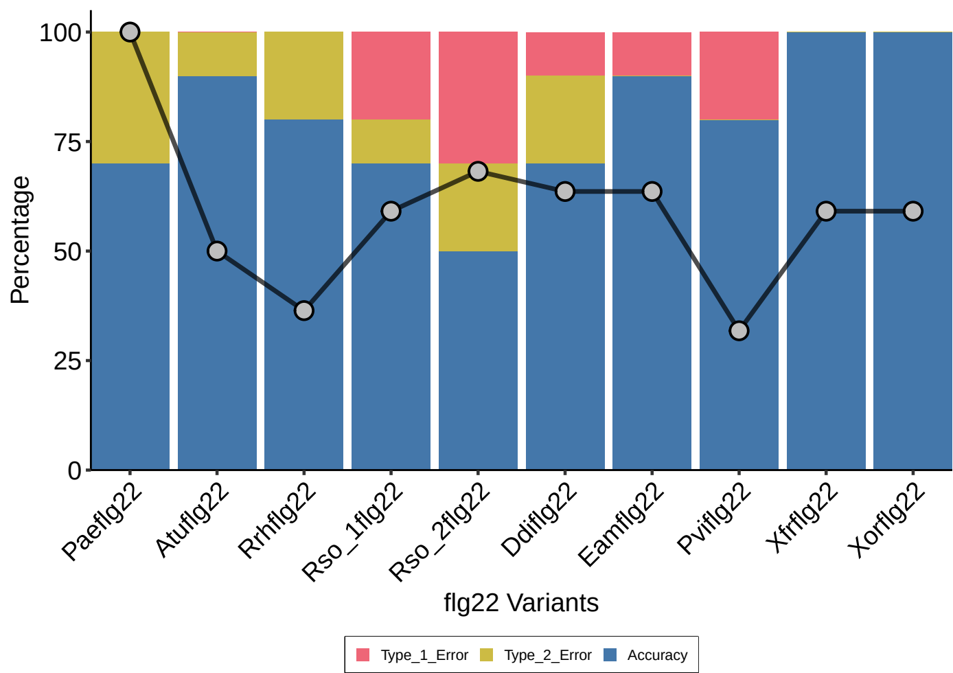
Metric at ipTM Cutoff 0.82
