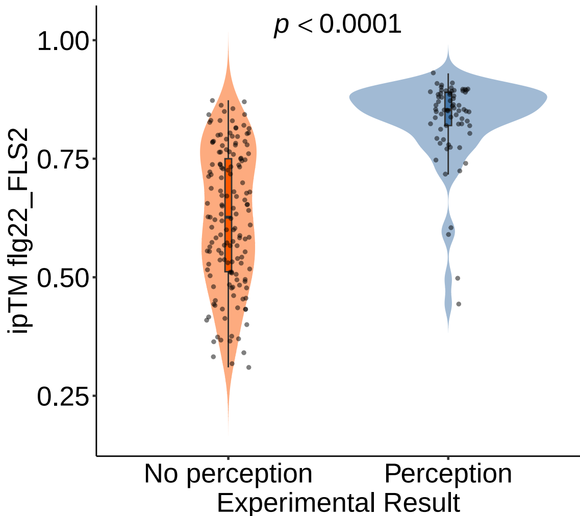
Raincloud Plot of ipTM flg22_FLS2 by Experimental Result
