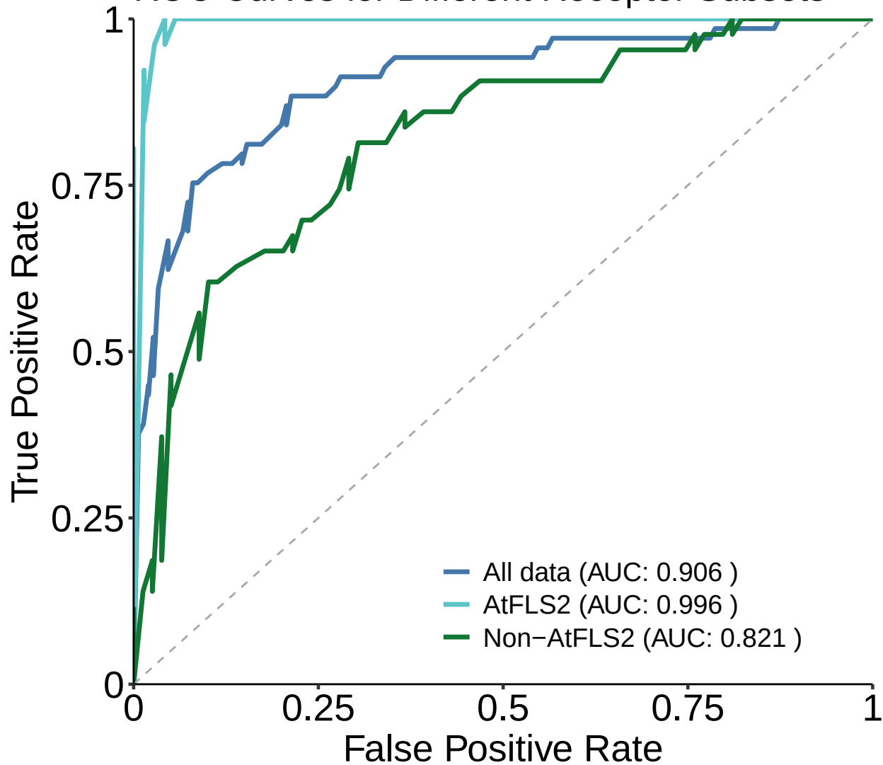
ROC Curves for Different Receptor Subsets
