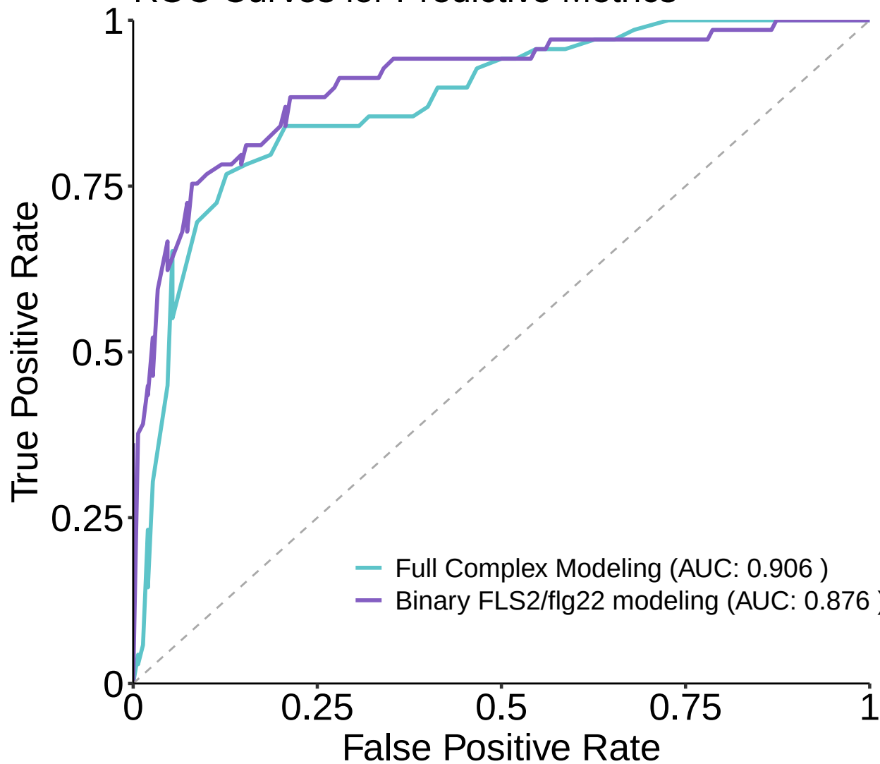
ROC Curves for Predictive Metrics
