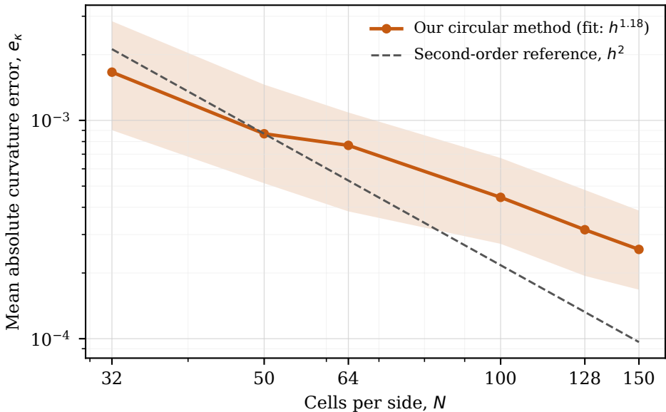
Ellipse curvature-estimate convergence (Cartesian mesh)
