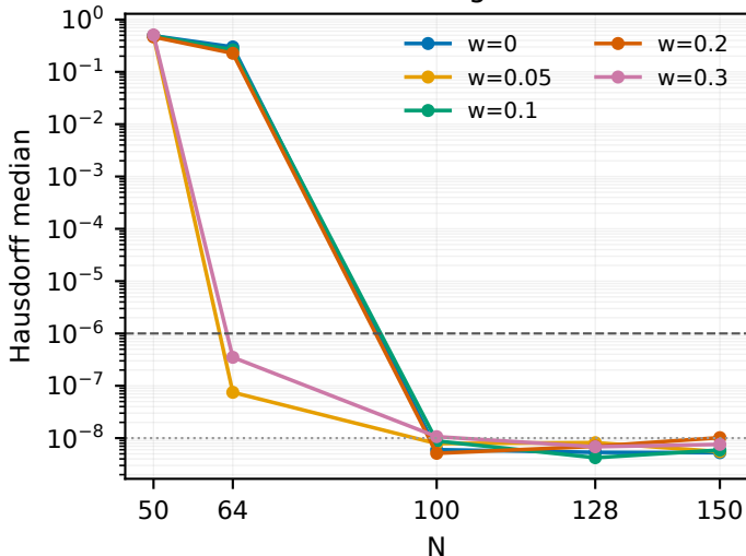
Zalesak: threshold sensitivity
