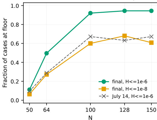
Zalesak: threshold sensitivity
