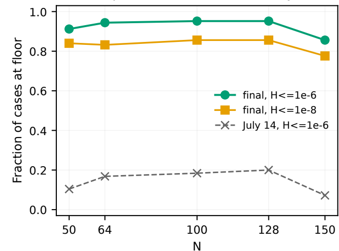
Squares: threshold sensitivity
