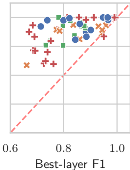
gpt-oss-20b | Ministral-3-3B
