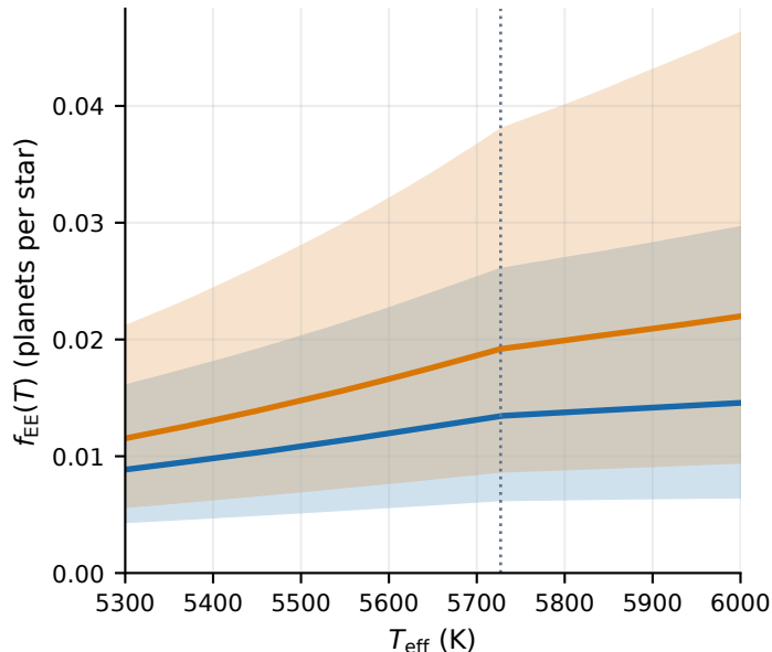
Narrow-domain occurrence
