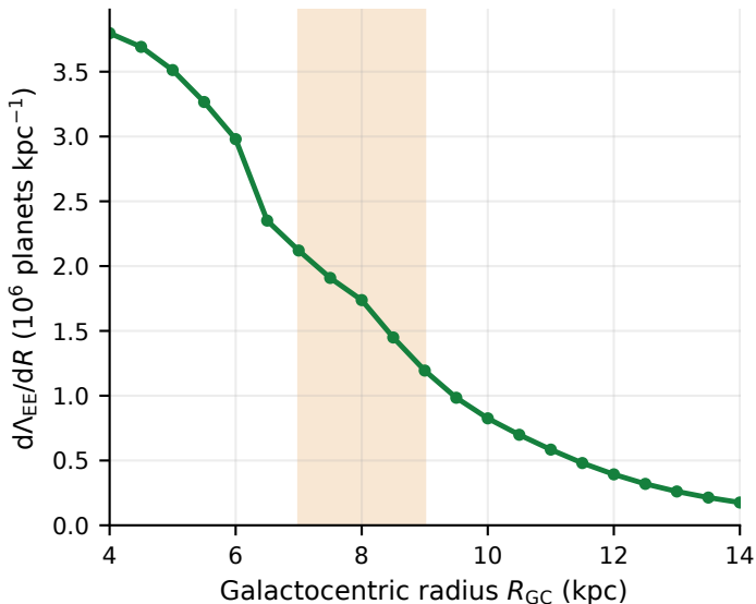
Point-vector ExoEarth intensity
