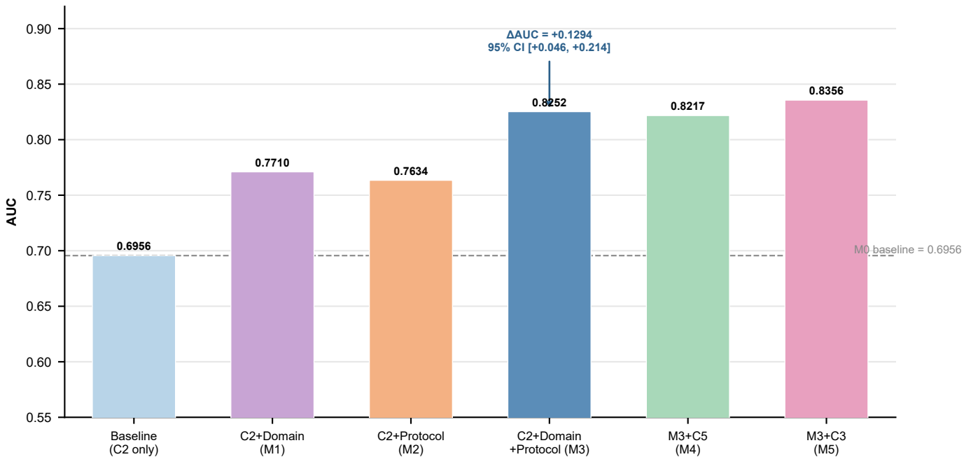
Incremental Model AUC Comparison
