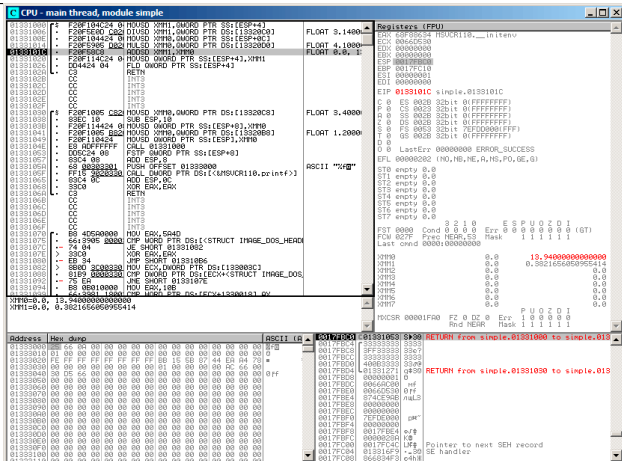
Figura 27.3: OllyDbg: MULSD product XMM0
