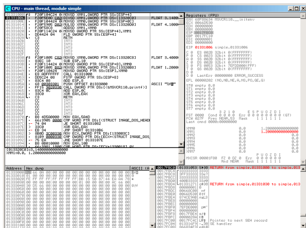
Figura 27.1: OllyDbg: MOVSD a XMM1
