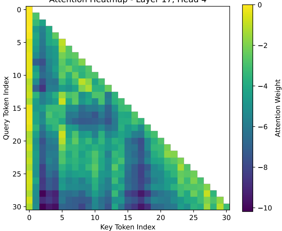
Attention Heatmap - Layer 17, Head 4
