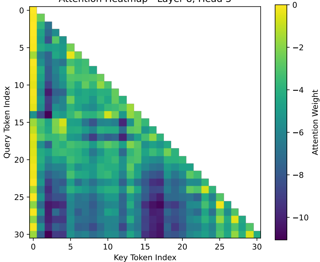
Attention Heatmap - Layer 8, Head 3
