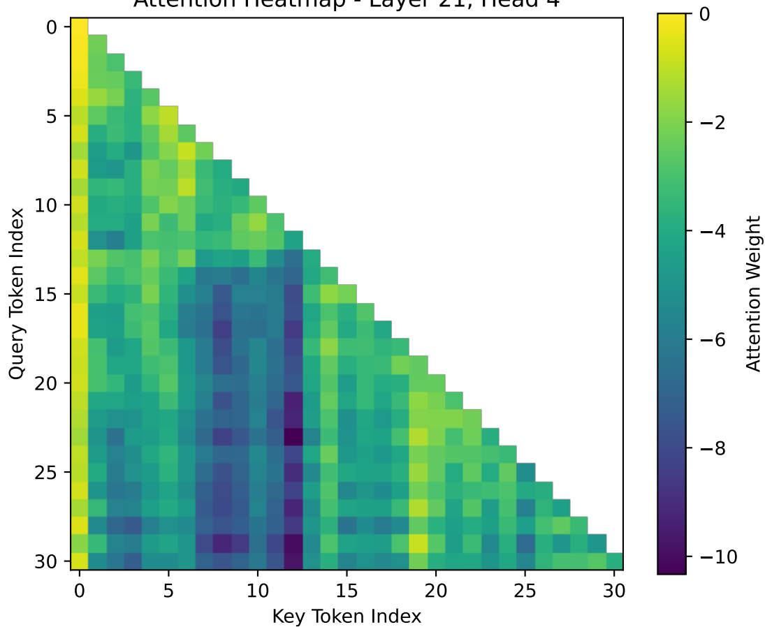
Attention Heatmap - Layer 21, Head 4
