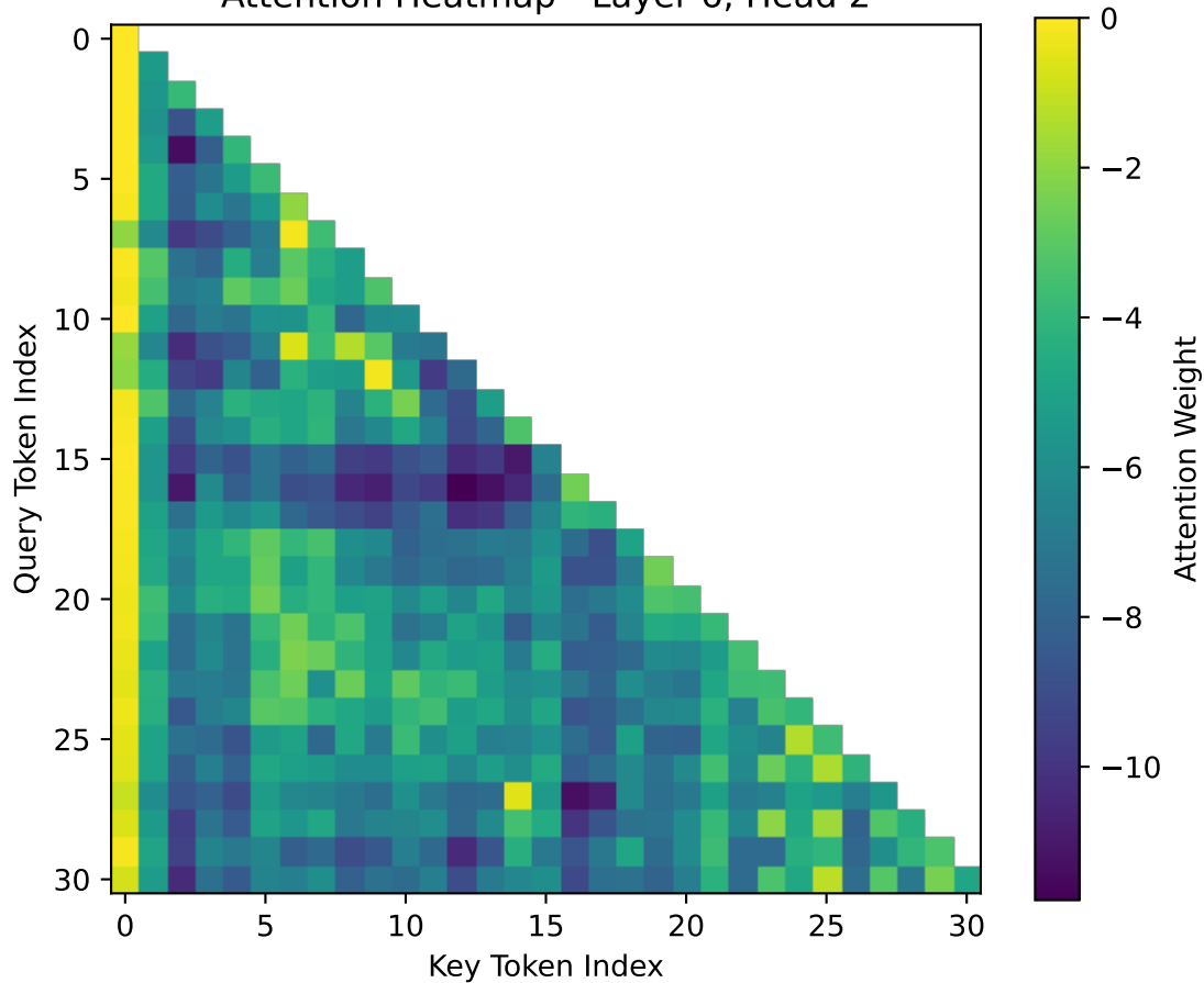
Attention Heatmap - Layer 6, Head 2
