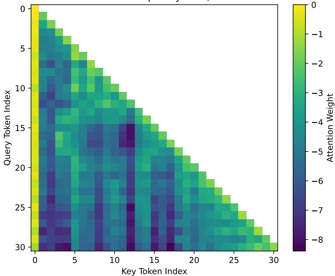
Attention Heatmap - Layer 20, Head 2
