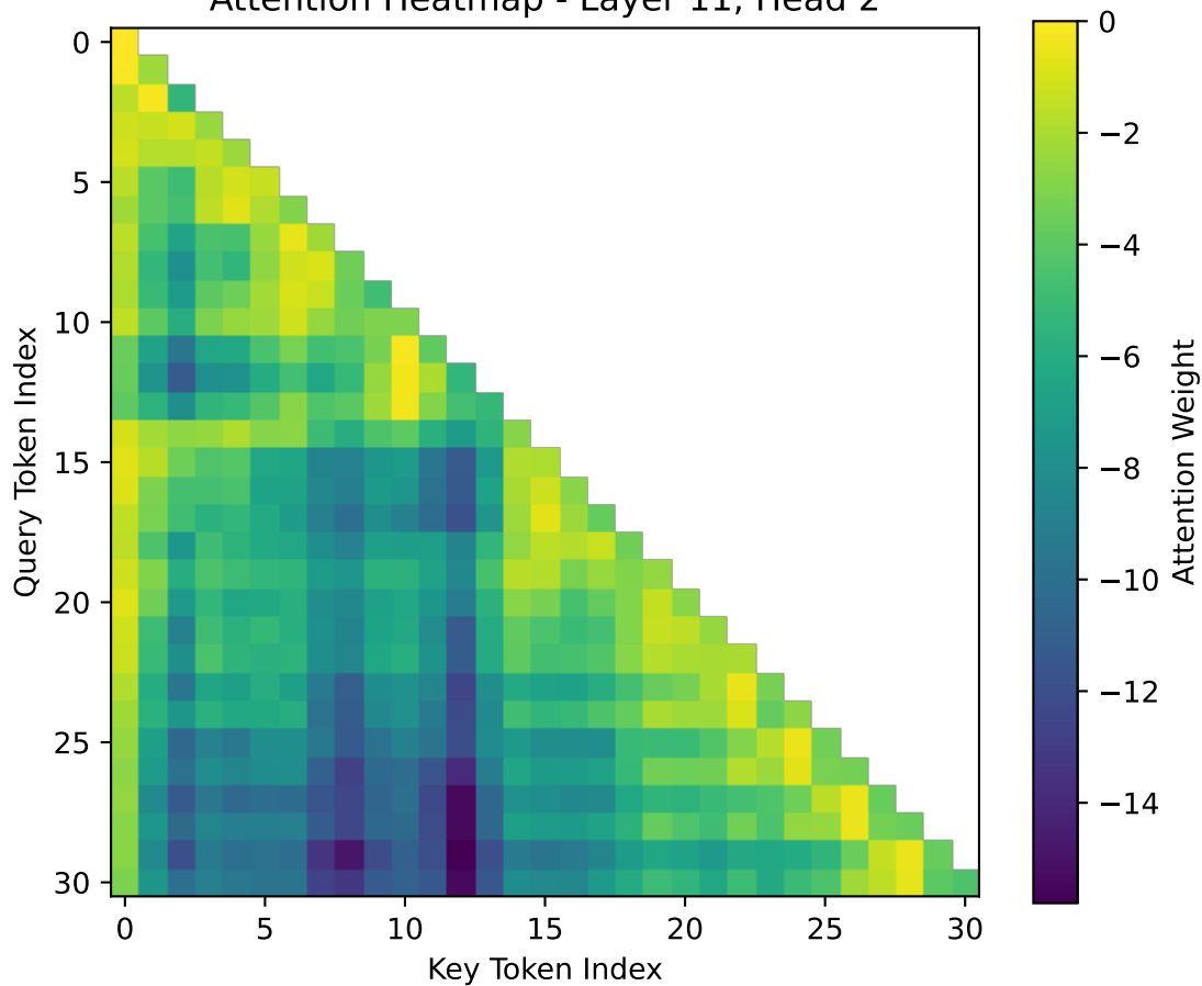
Attention Heatmap - Layer 11, Head 2
