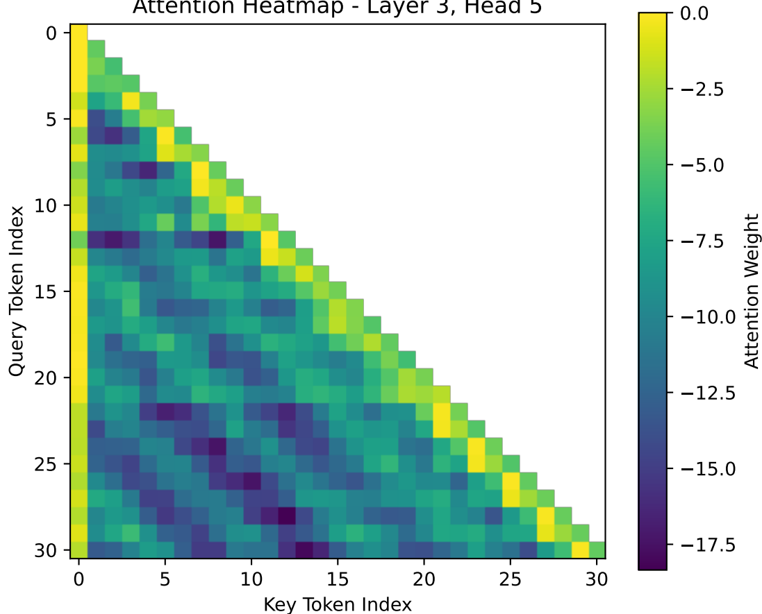
Attention Heatmap - Layer 3, Head 5
