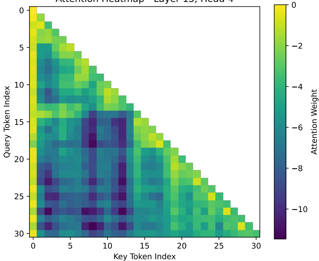
Attention Heatmap - Layer 15, Head 4
