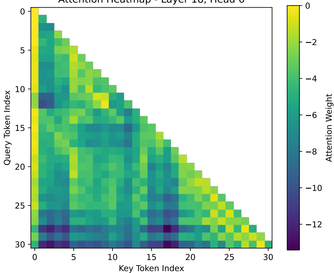
Attention Heatmap - Layer 18, Head 6
