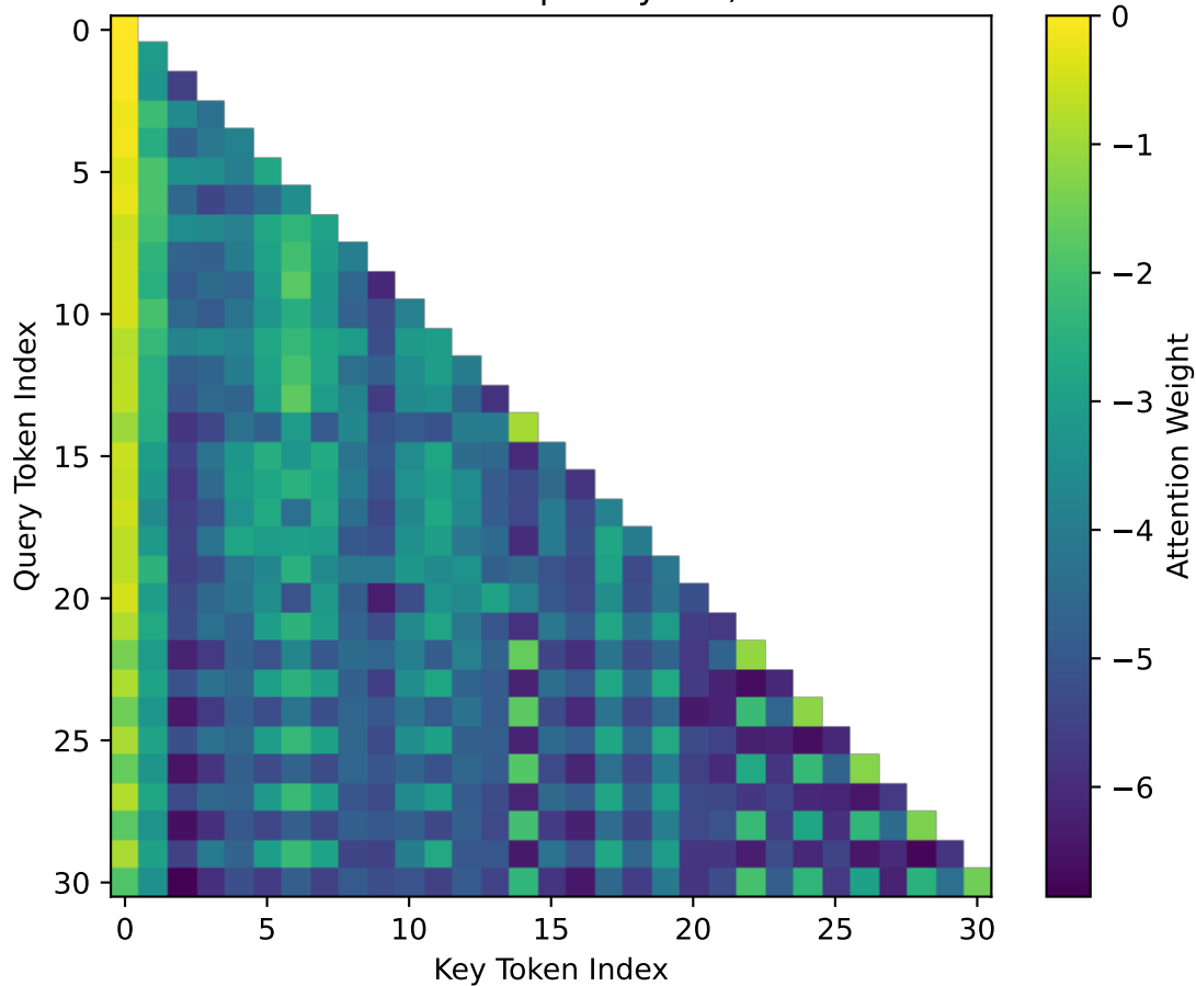
Attention Heatmap - Layer 0, Head 6
