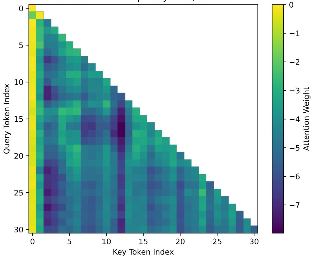
Attention Heatmap - Layer 13, Head 5
