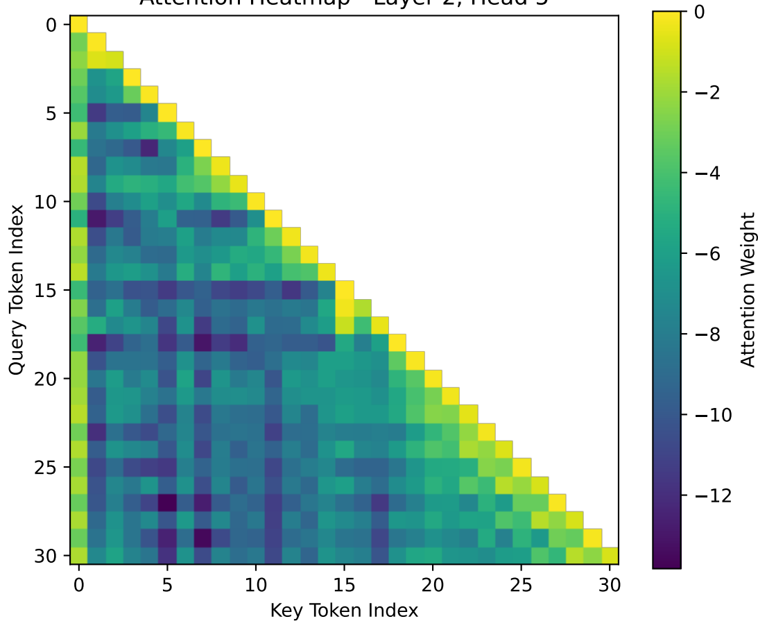
Attention Heatmap - Layer 2, Head 5
