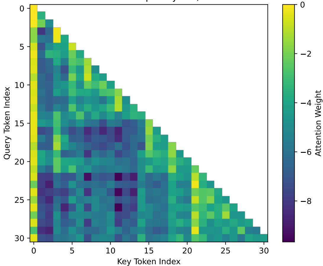
Attention Heatmap - Layer 3, Head 3
