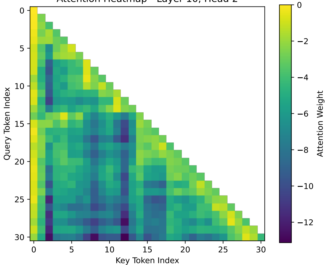
Attention Heatmap - Layer 10, Head 2
