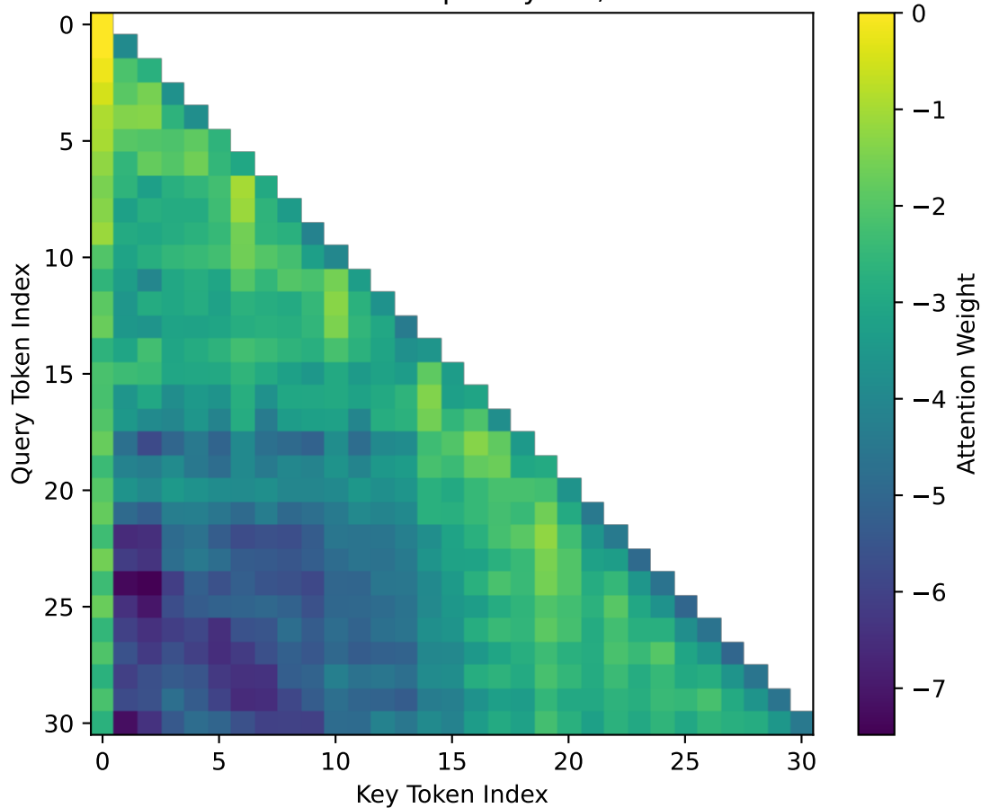
Attention Heatmap - Layer 2, Head 7
