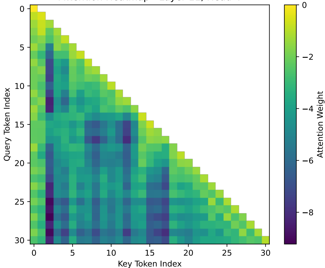
Attention Heatmap - Layer 11, Head 4
