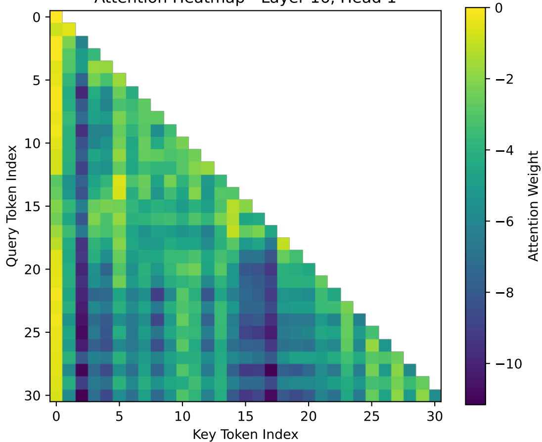
Attention Heatmap - Layer 16, Head 1
