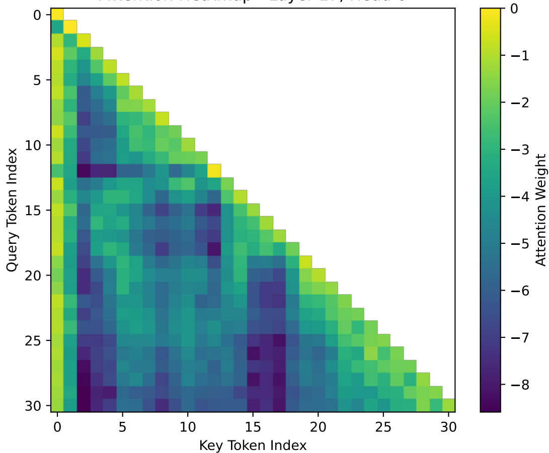
Attention Heatmap - Layer 17, Head 6
