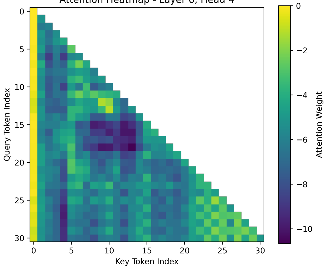
Attention Heatmap - Layer 6, Head 4
