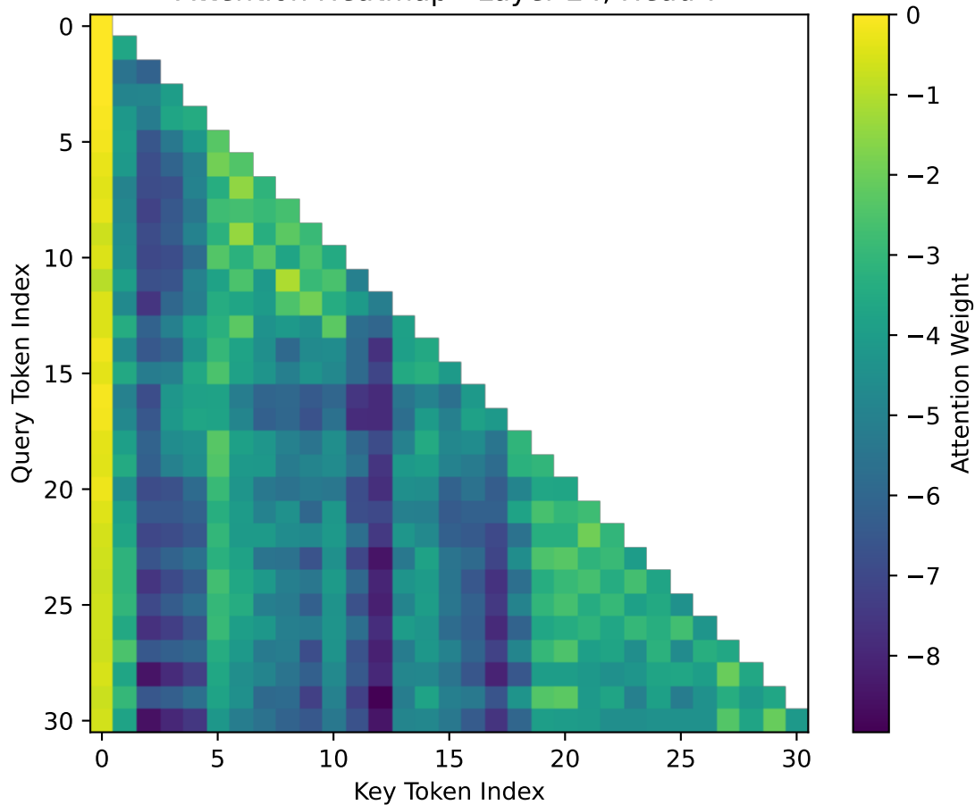
Attention Heatmap - Layer 24, Head 7
