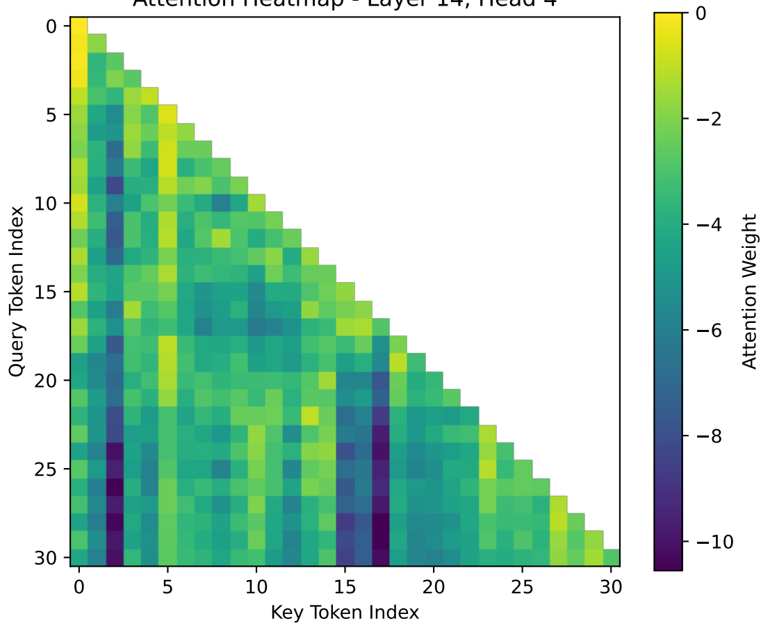
Attention Heatmap - Layer 14, Head 4
