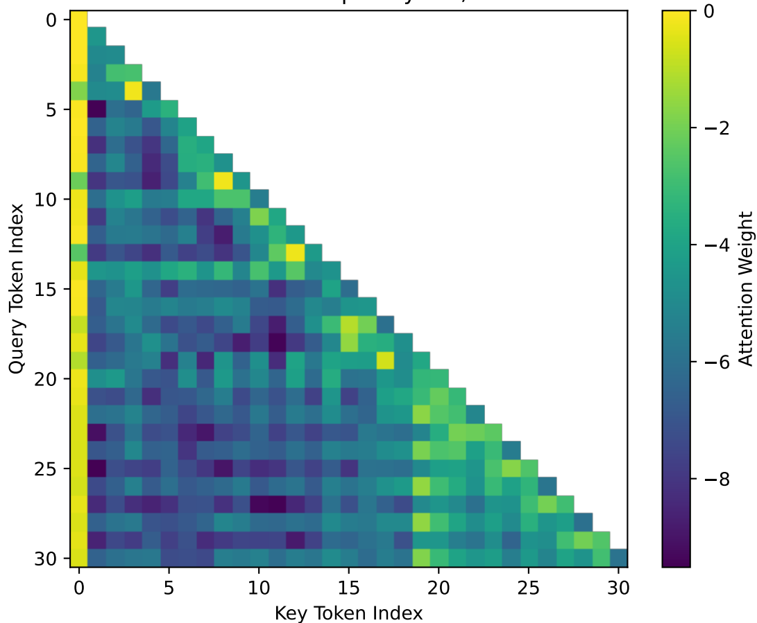
Attention Heatmap - Layer 2, Head 1
