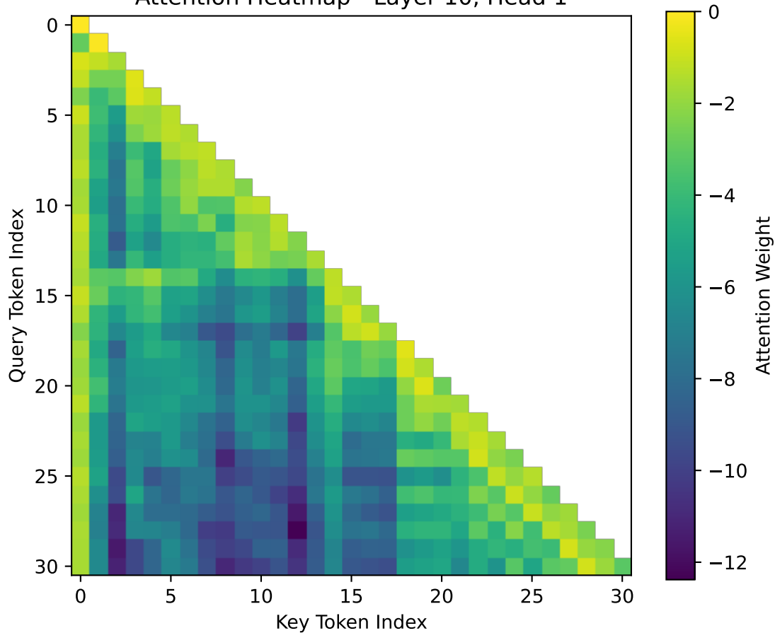
Attention Heatmap - Layer 10, Head 1
