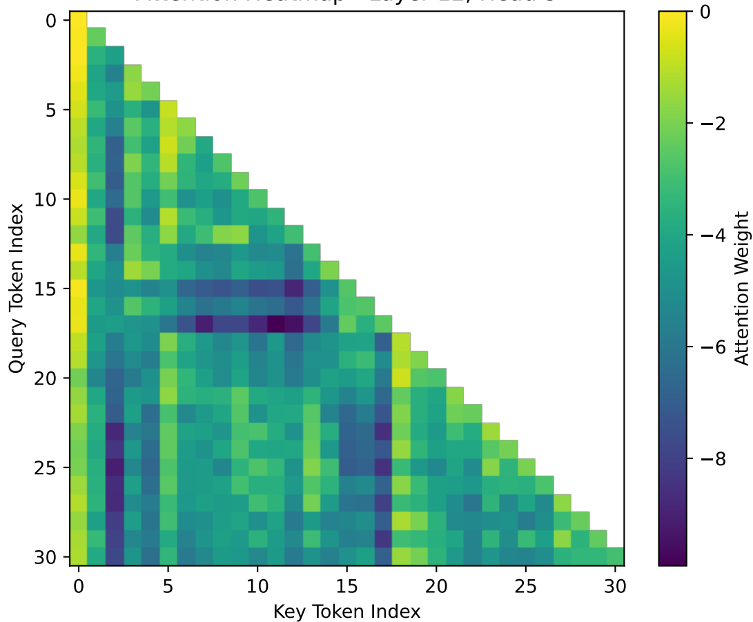
Attention Heatmap - Layer 12, Head 3
