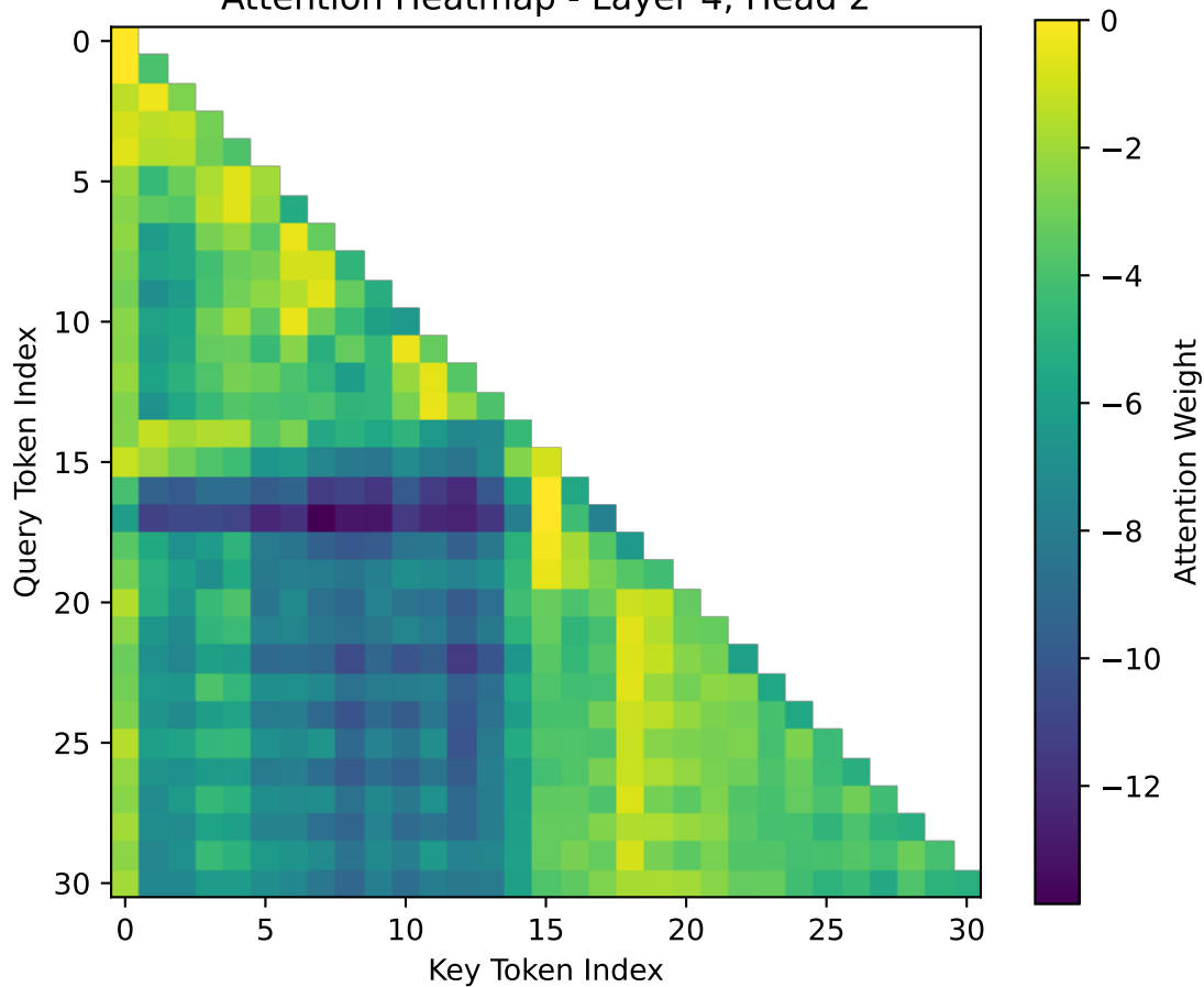
Attention Heatmap - Layer 4, Head 2
