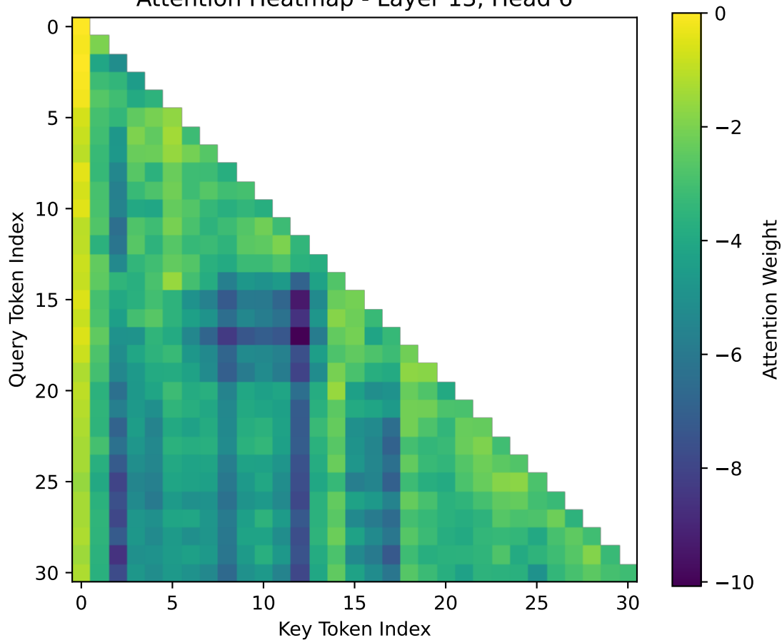
Attention Heatmap - Layer 13, Head 6
