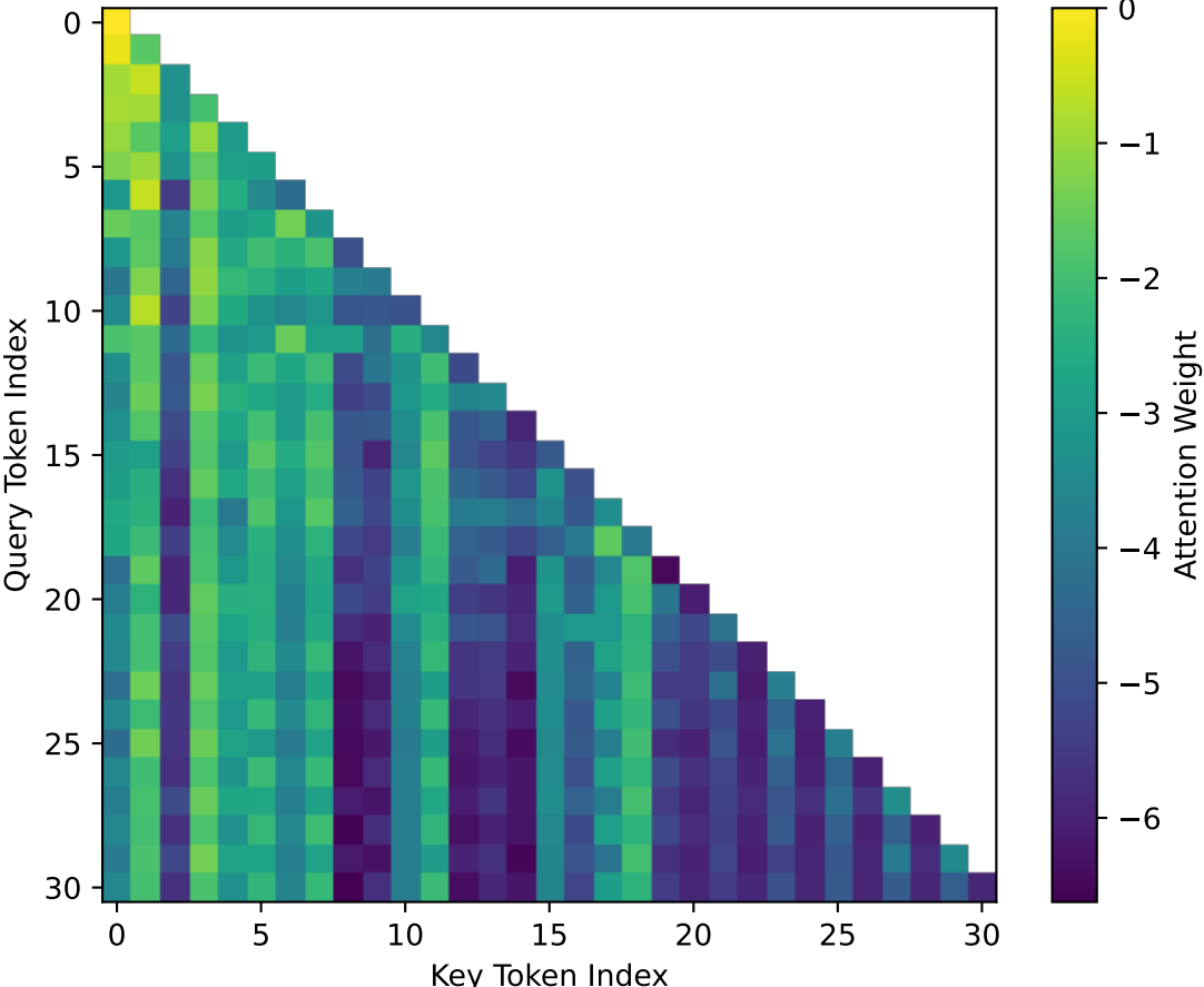
Attention Heatmap - Layer 0, Head 3
