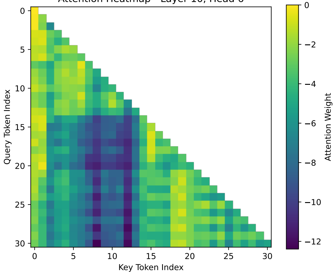
Attention Heatmap - Layer 10, Head 6
