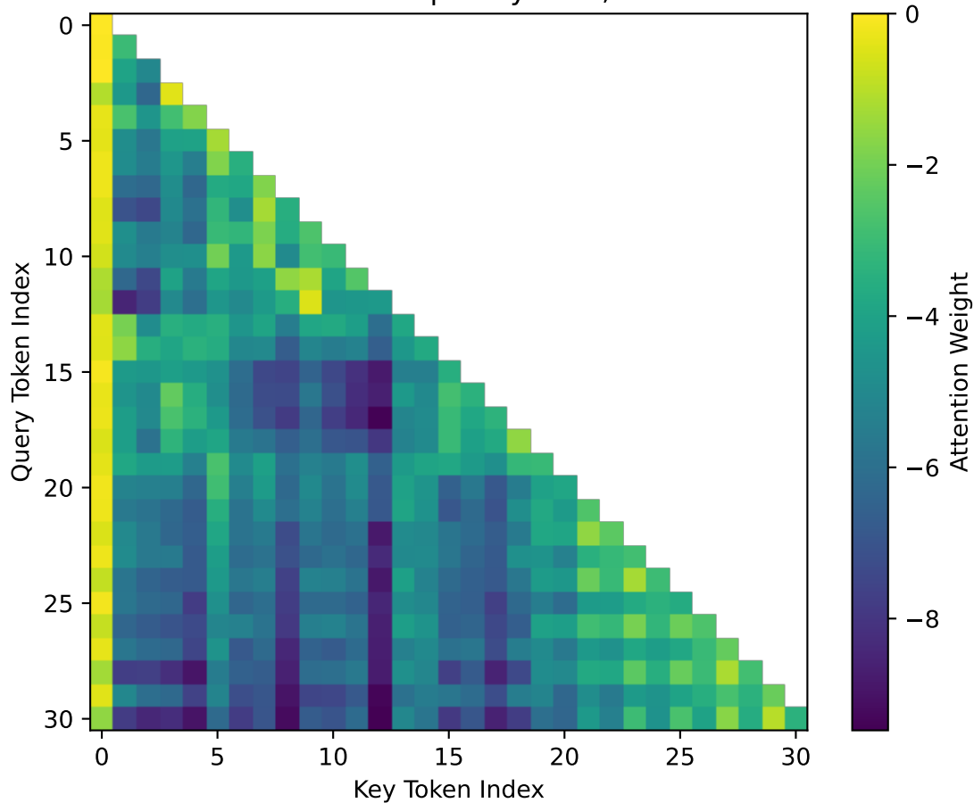
Attention Heatmap - Layer 20, Head 6
