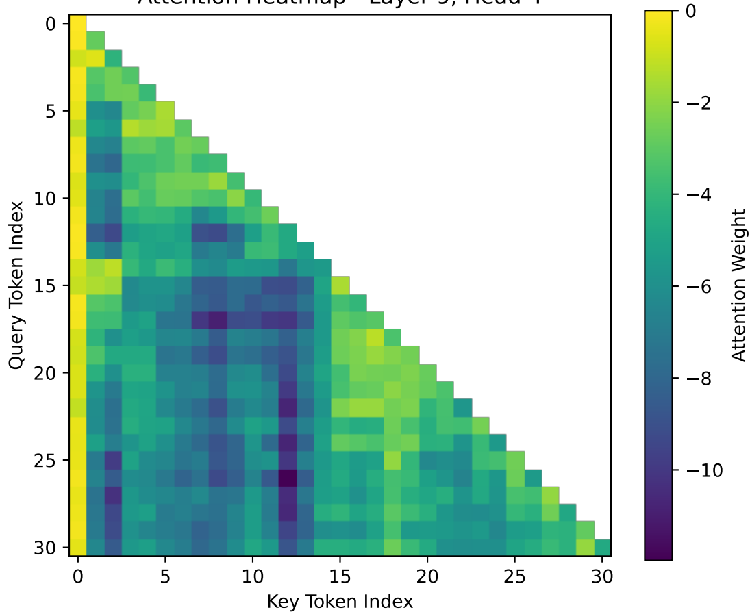
Attention Heatmap - Layer 9, Head 4
