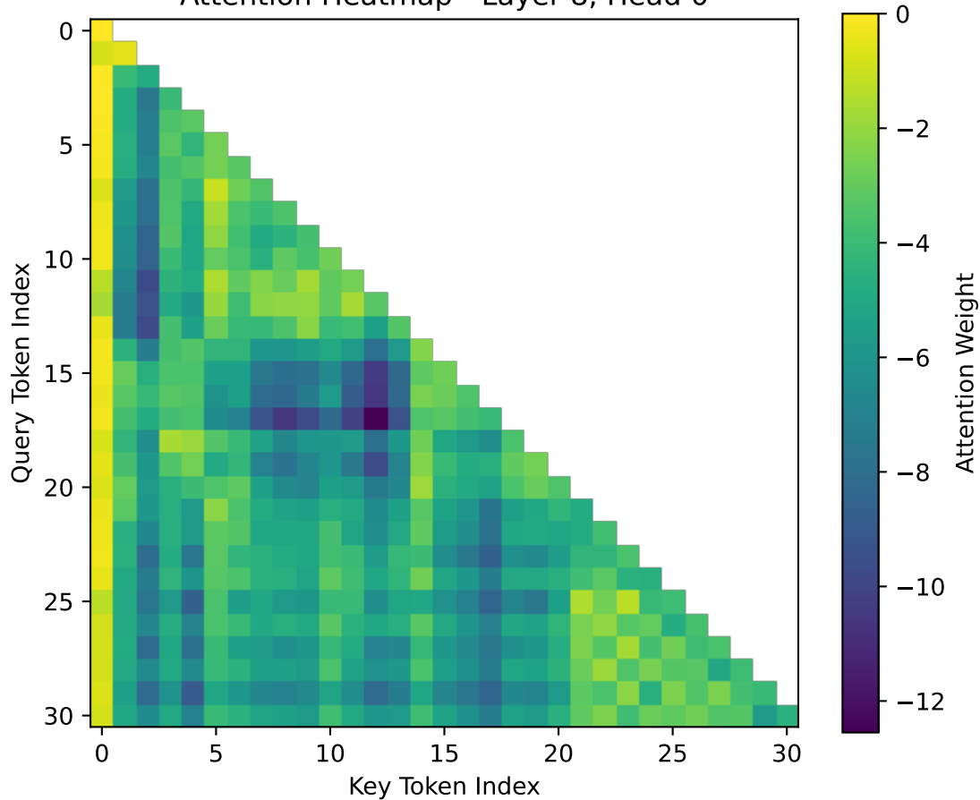
Attention Heatmap - Layer 8, Head 0
