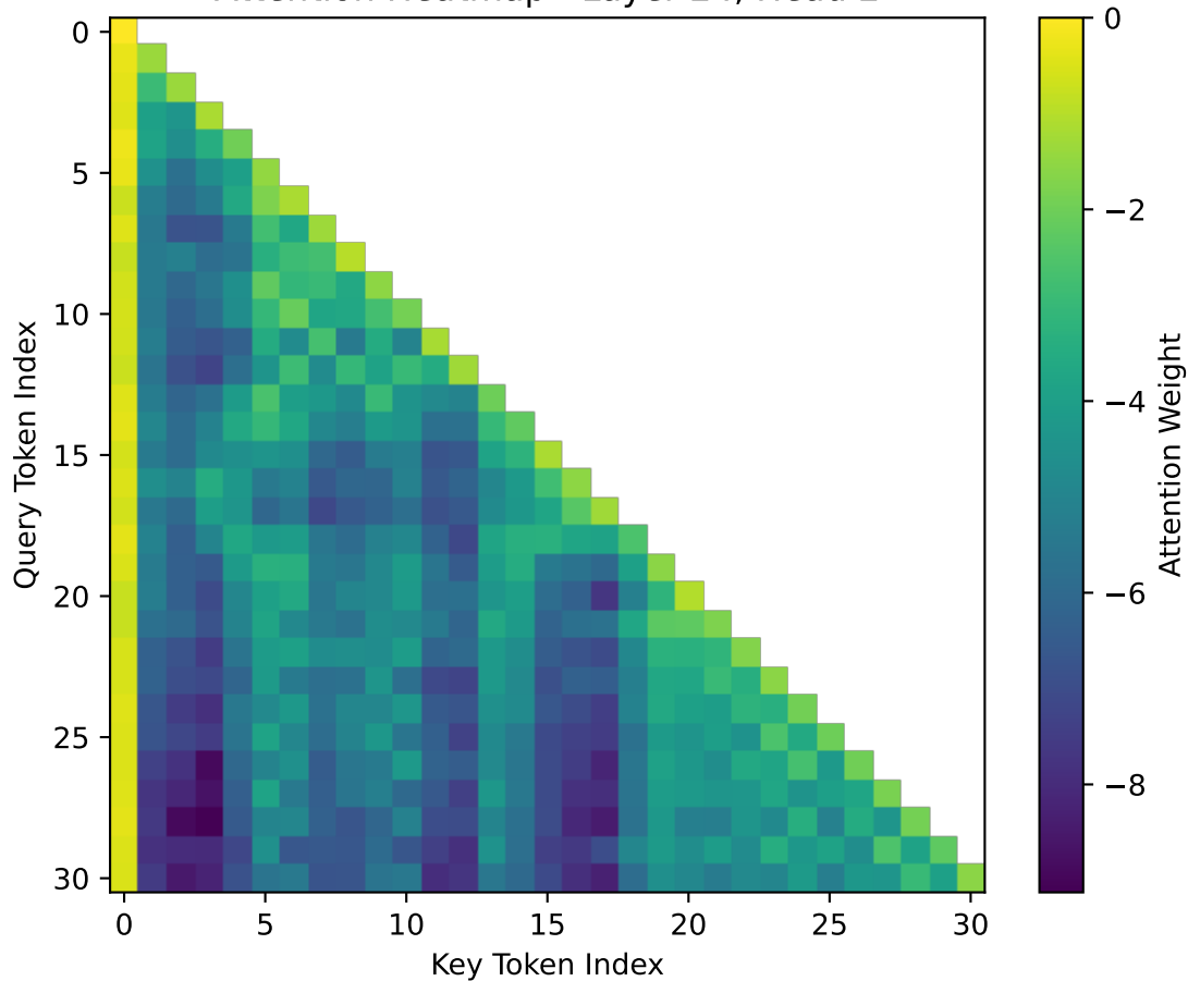
Attention Heatmap - Layer 24, Head 2
