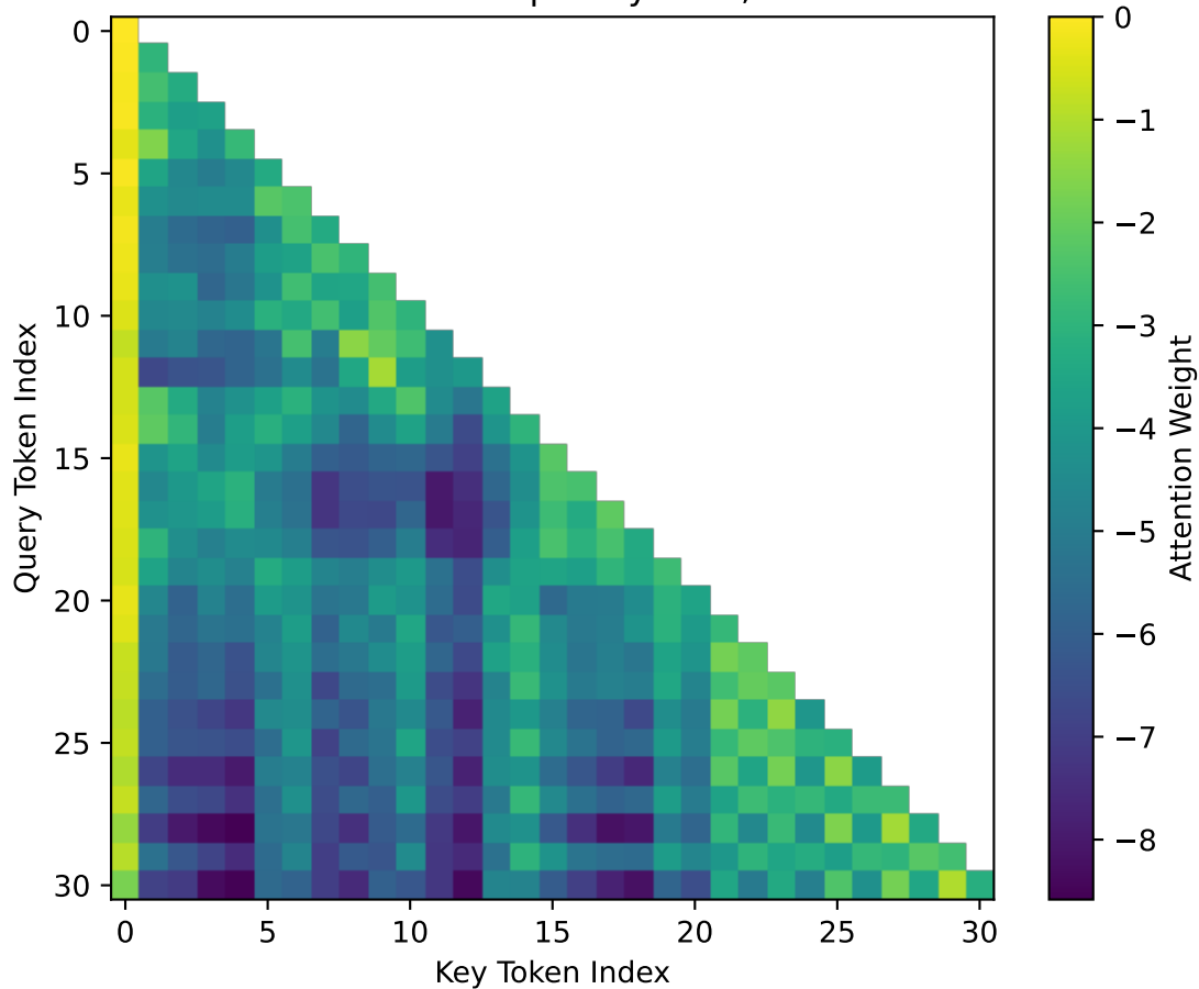
Attention Heatmap - Layer 22, Head 6
