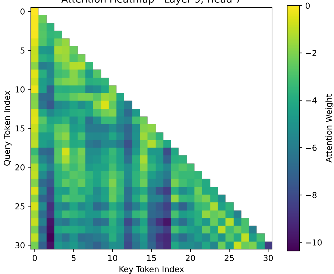
Attention Heatmap - Layer 9, Head 7
