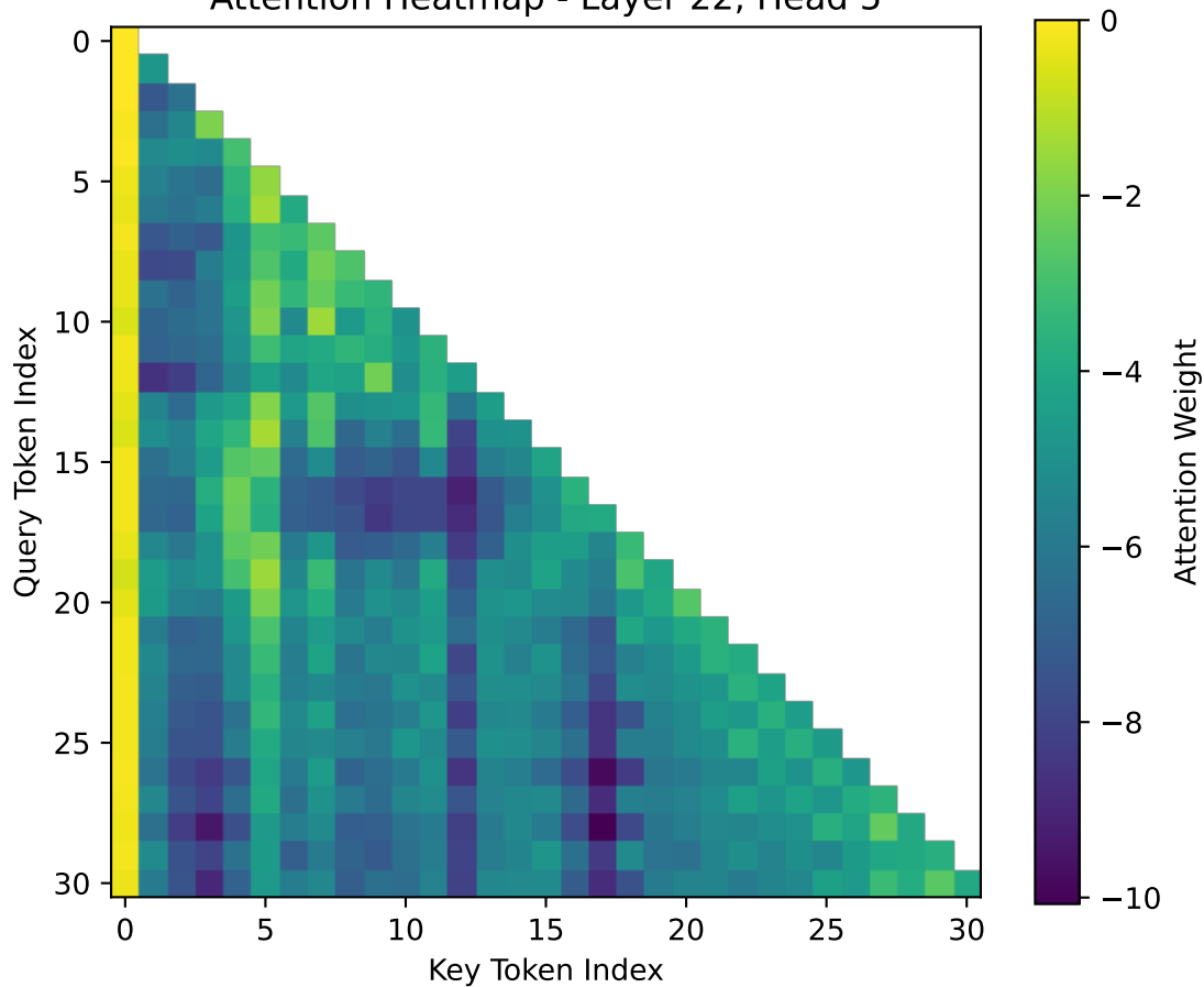
Attention Heatmap - Layer 22, Head 5
