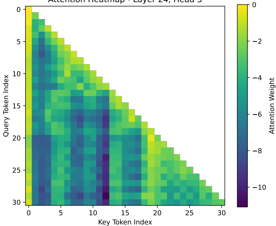
Attention Heatmap - Layer 24, Head 3
