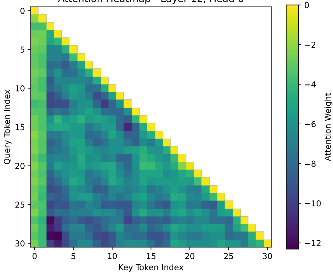
Attention Heatmap - Layer 12, Head 6
