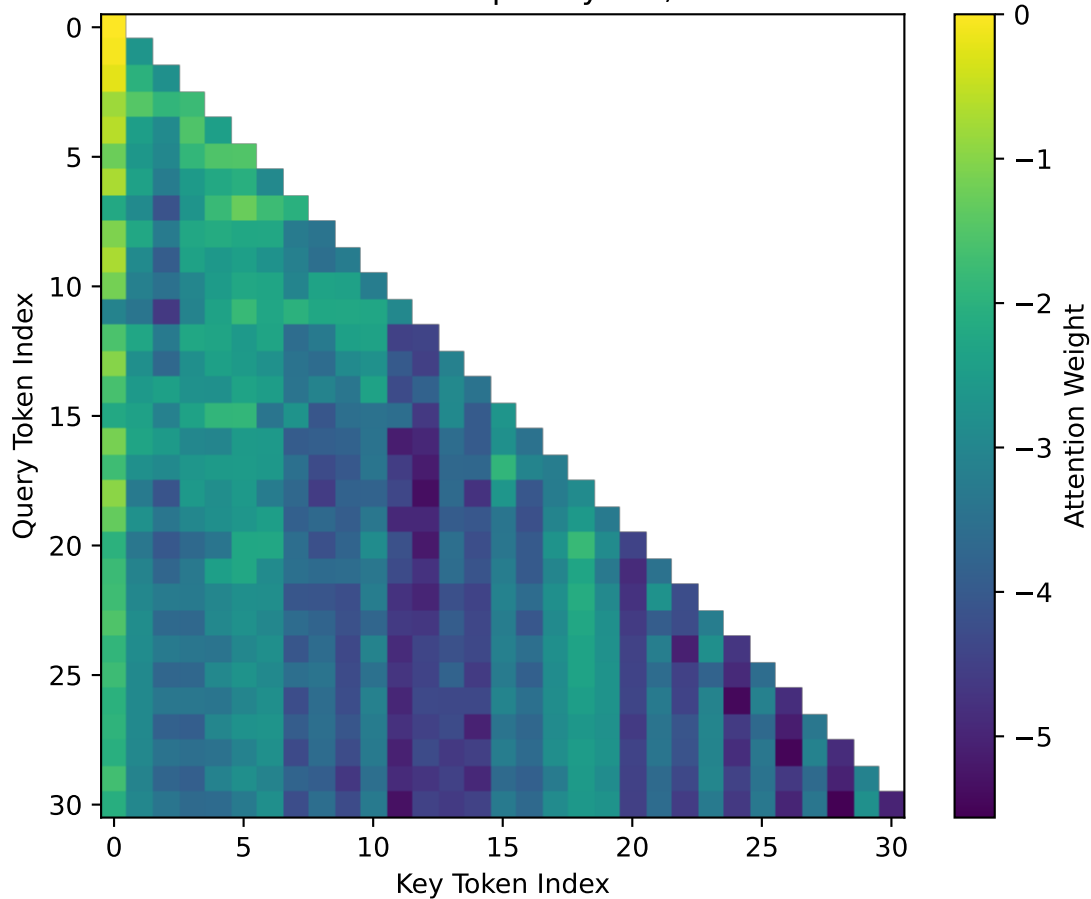
Attention Heatmap - Layer 1, Head 1
