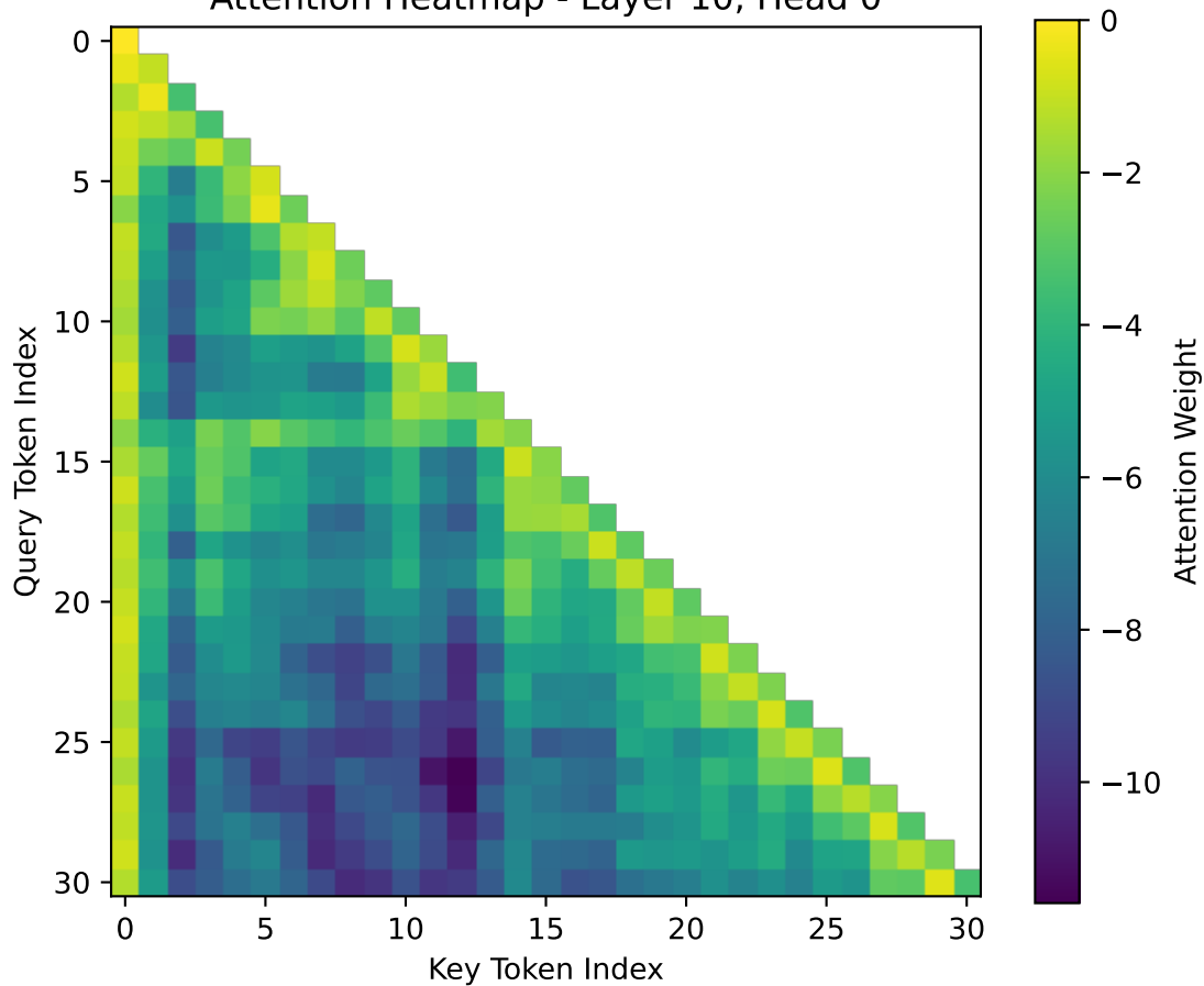
Attention Heatmap - Layer 10, Head 0
