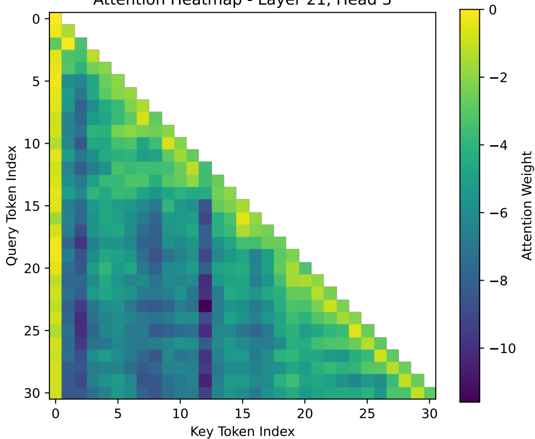
Attention Heatmap - Layer 21, Head 3
