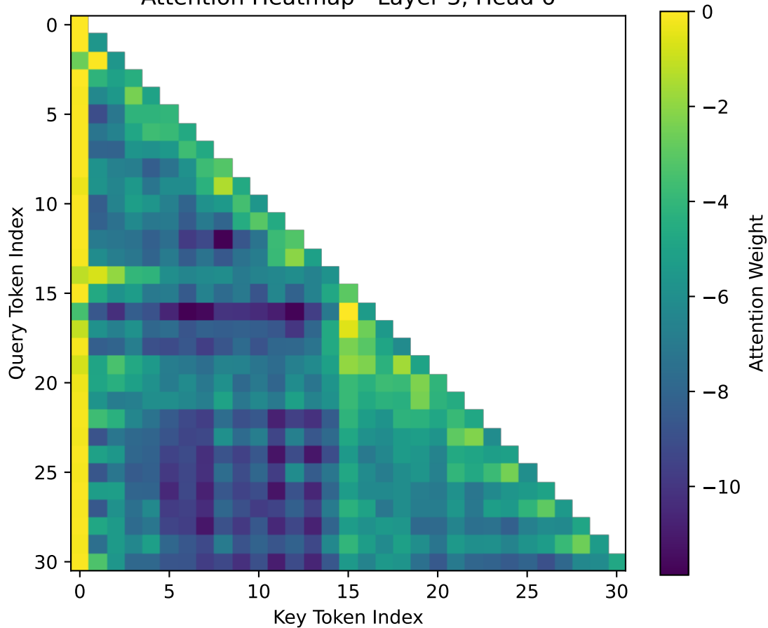
Attention Heatmap - Layer 3, Head 6
