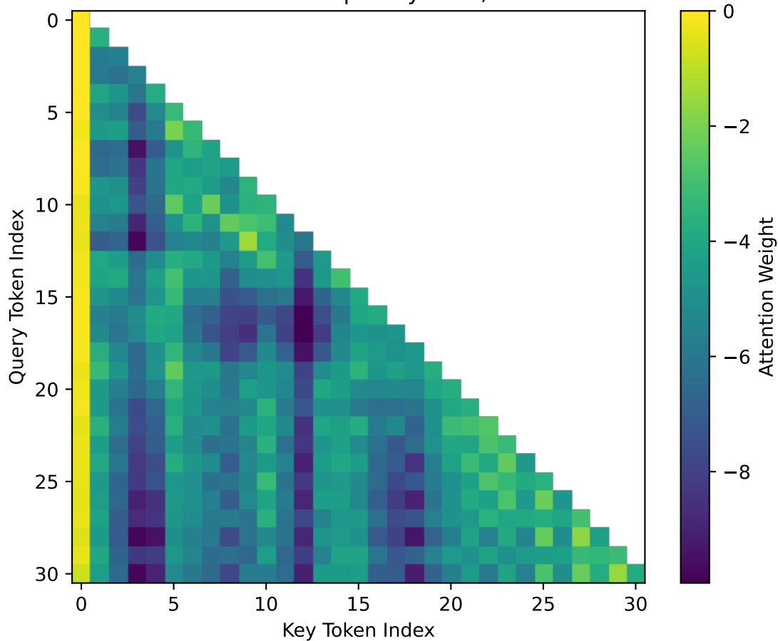
Attention Heatmap - Layer 22, Head 7
