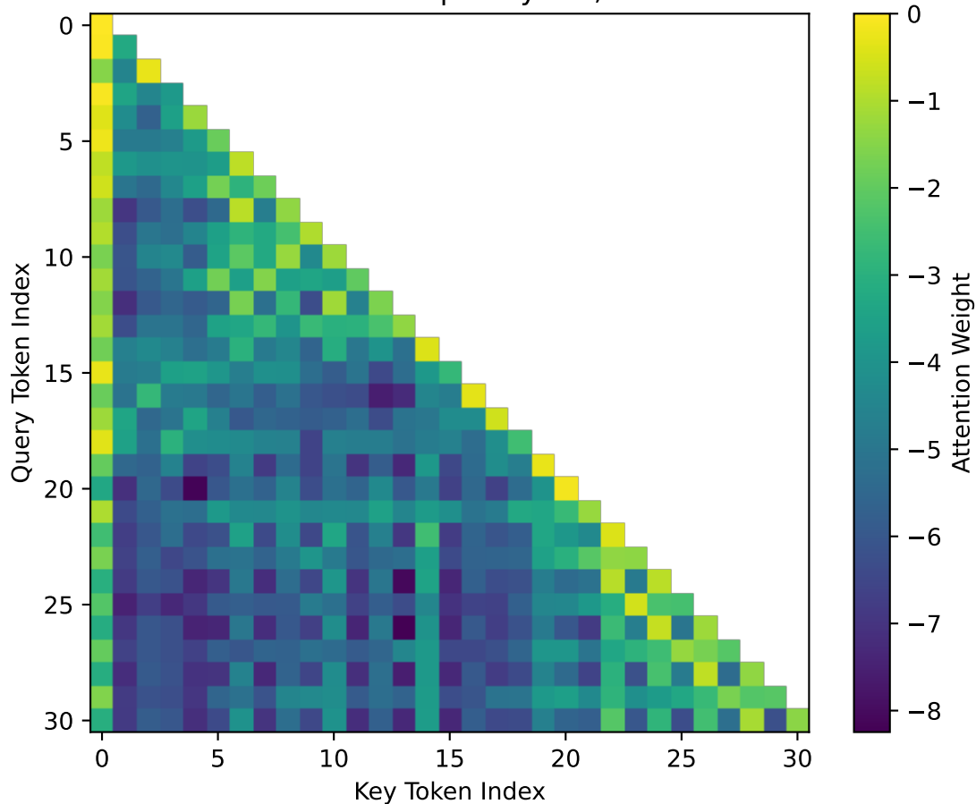
Attention Heatmap - Layer 2, Head 3
