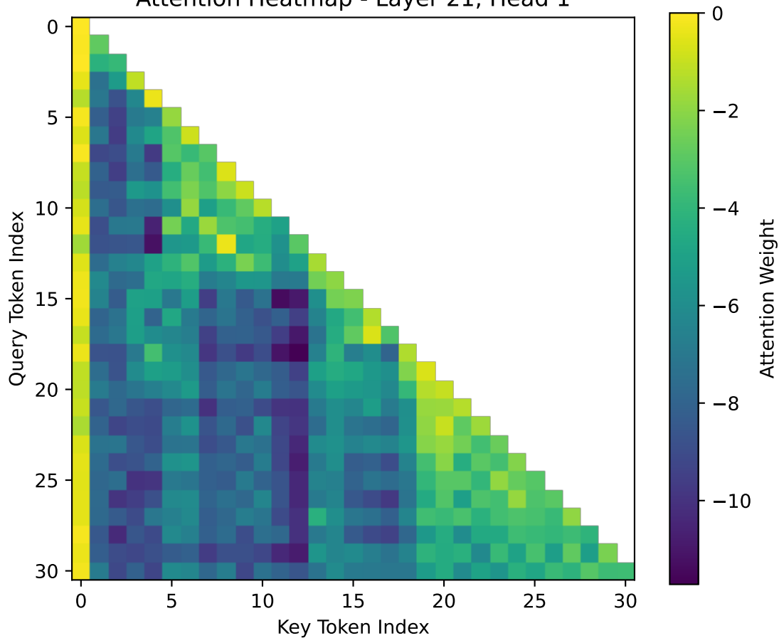
Attention Heatmap - Layer 21, Head 1
