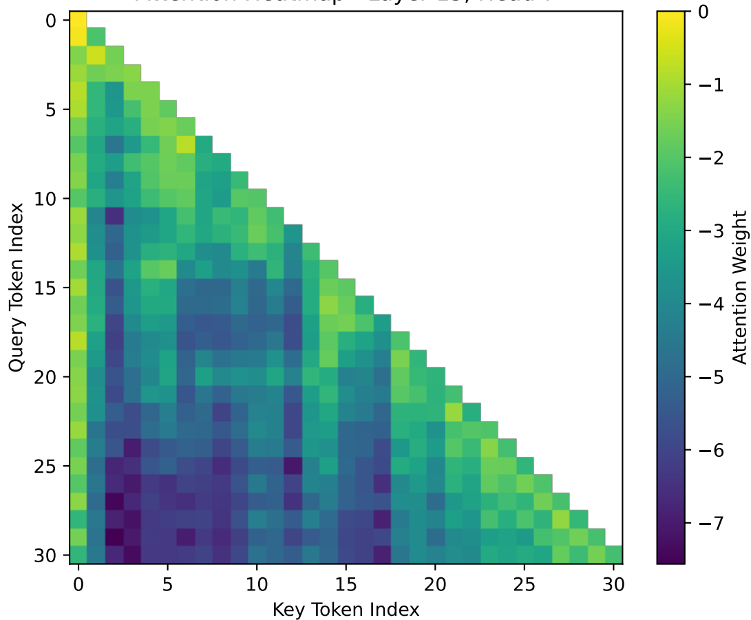
Attention Heatmap - Layer 15, Head 7
