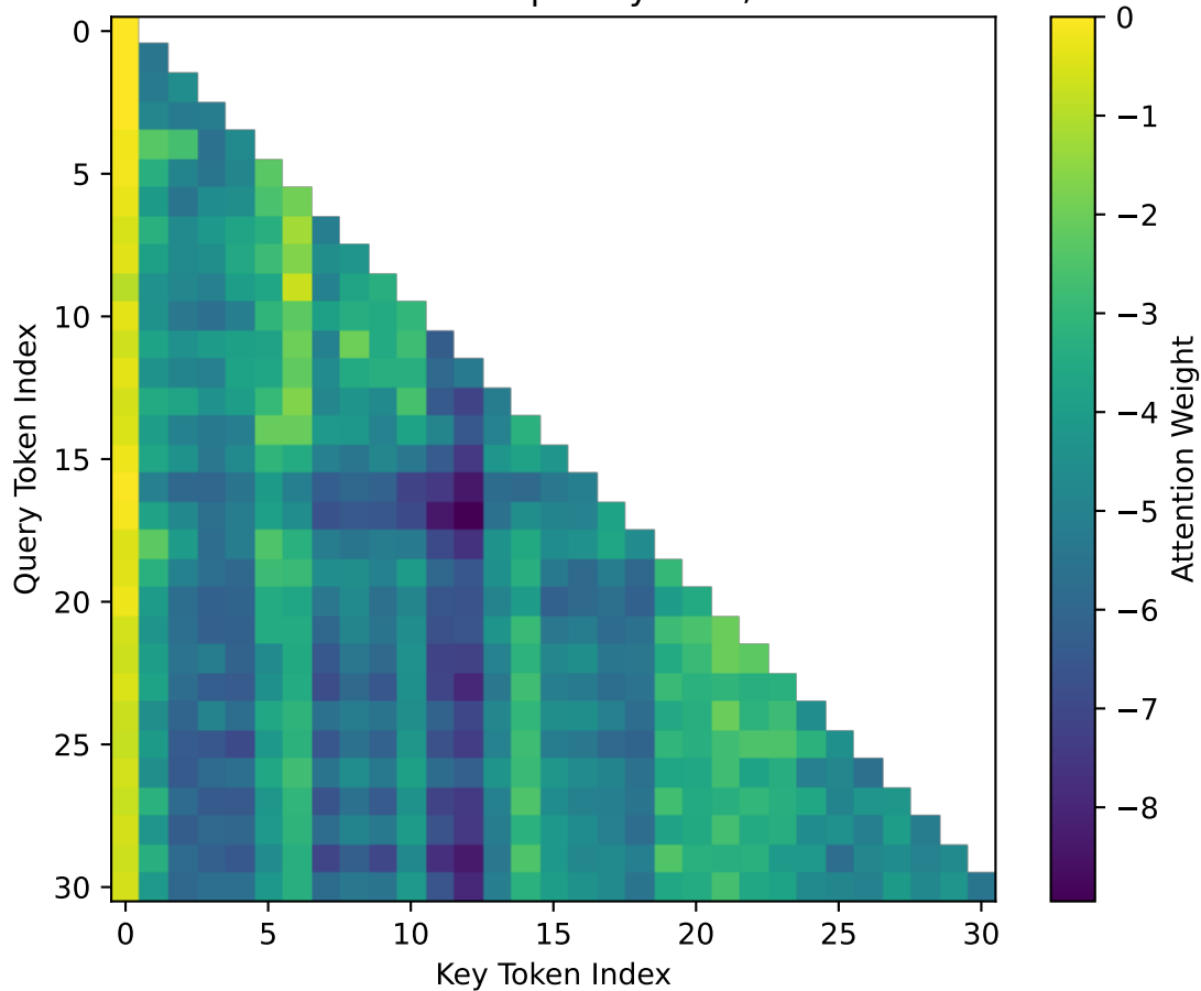
Attention Heatmap - Layer 20, Head 4
