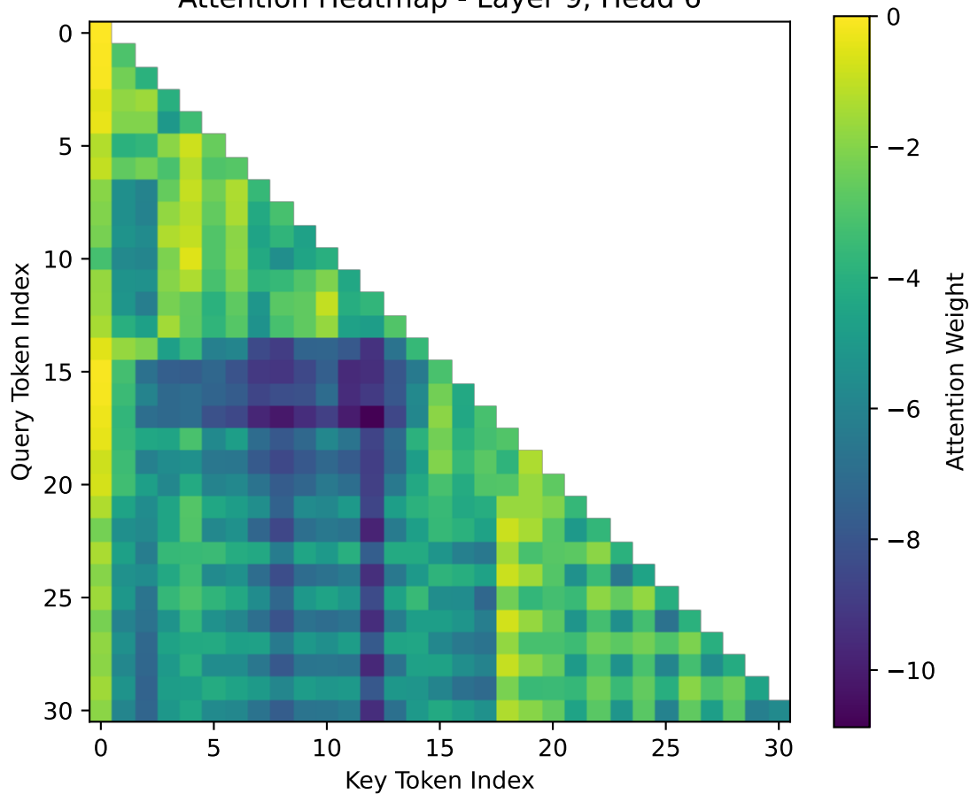
Attention Heatmap - Layer 9, Head 6
