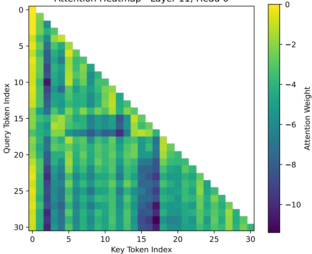
Attention Heatmap - Layer 11, Head 6
