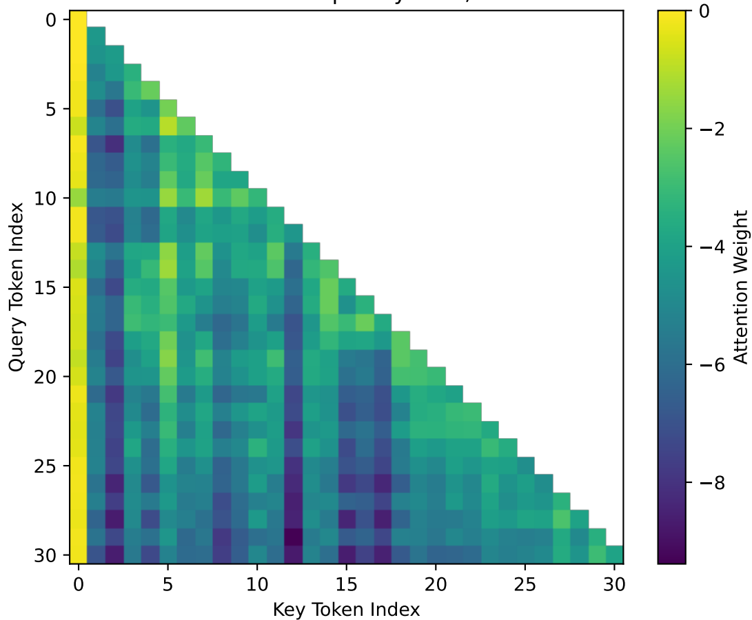
Attention Heatmap - Layer 20, Head 3
