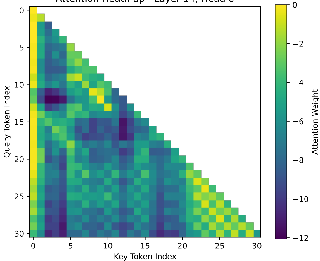
Attention Heatmap - Layer 14, Head 0
