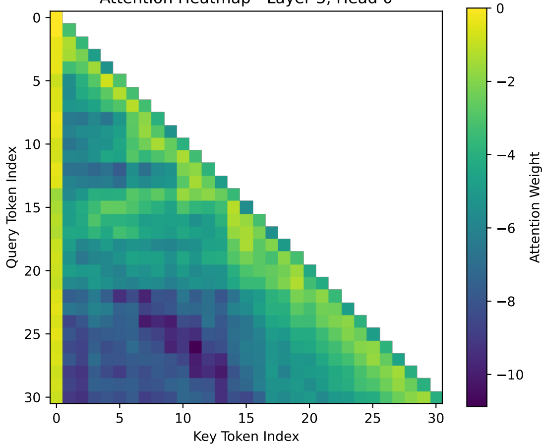
Attention Heatmap - Layer 3, Head 0
