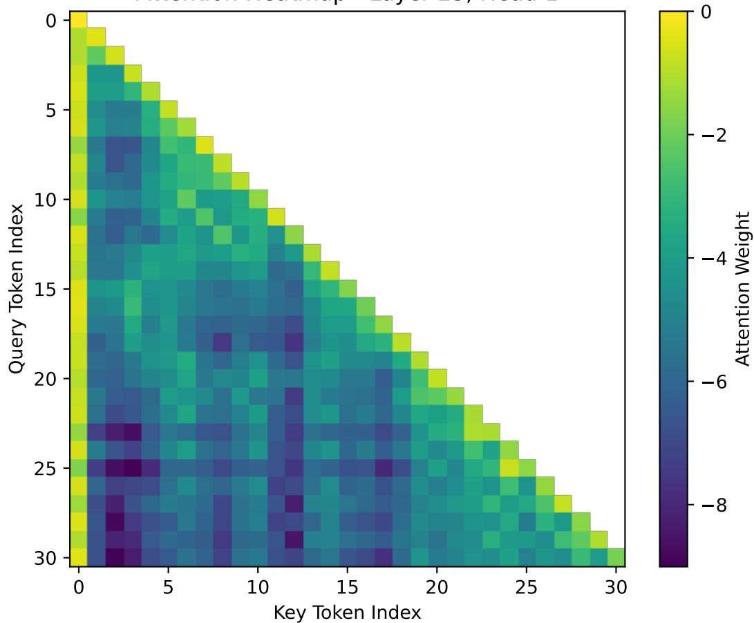
Attention Heatmap - Layer 23, Head 1
