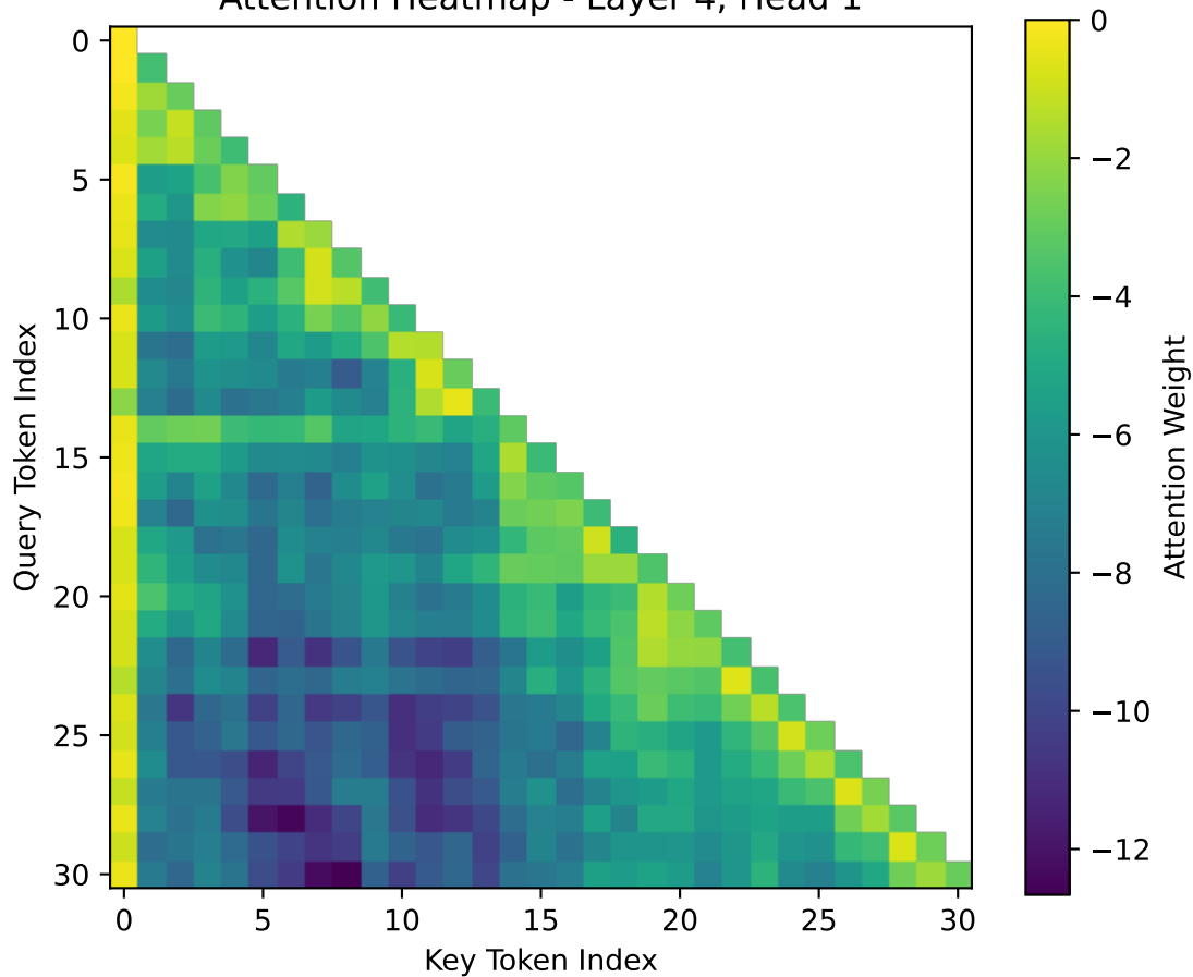
Attention Heatmap - Layer 4, Head 1
