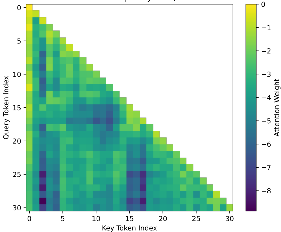
Attention Heatmap - Layer 14, Head 5
