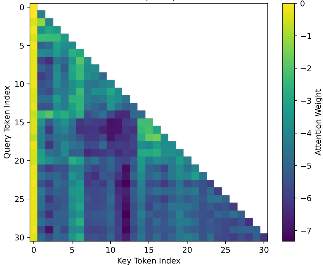
Attention Heatmap - Layer 5, Head 5
