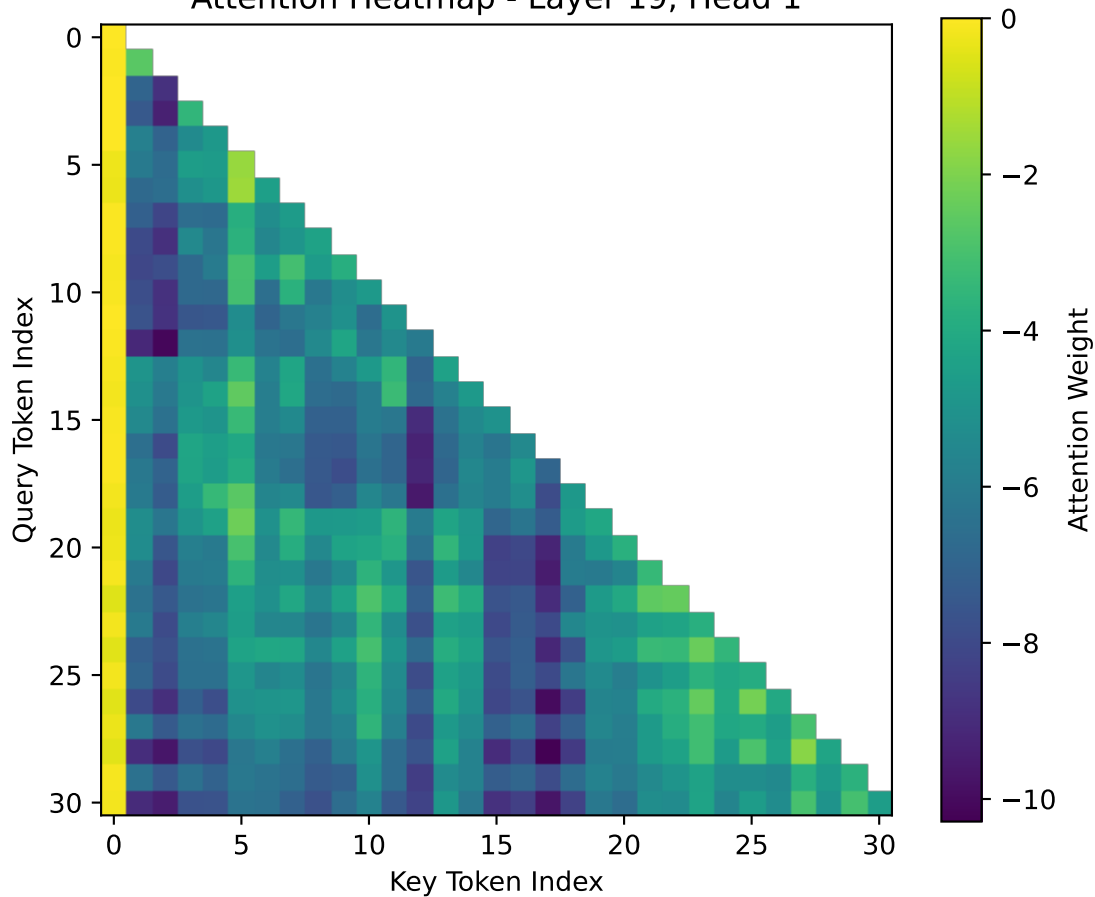
Attention Heatmap - Layer 19, Head 1
