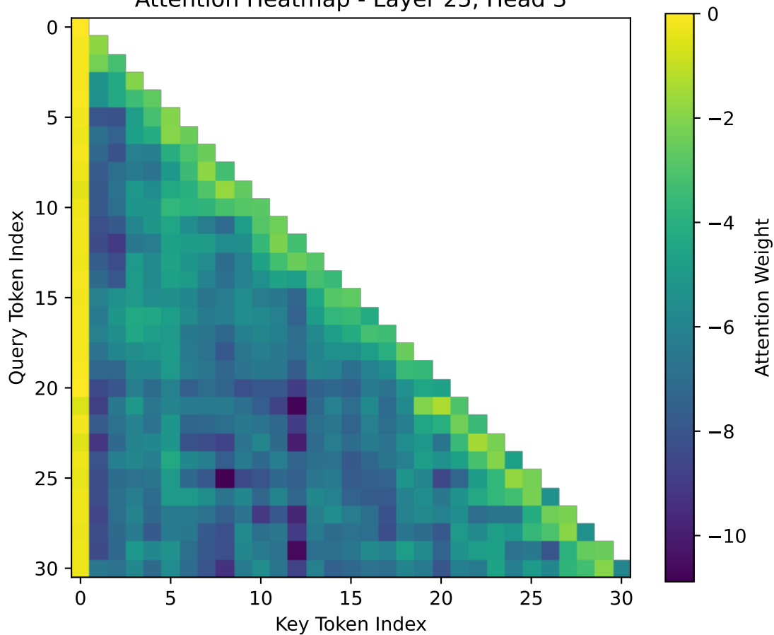
Attention Heatmap - Layer 25, Head 3
