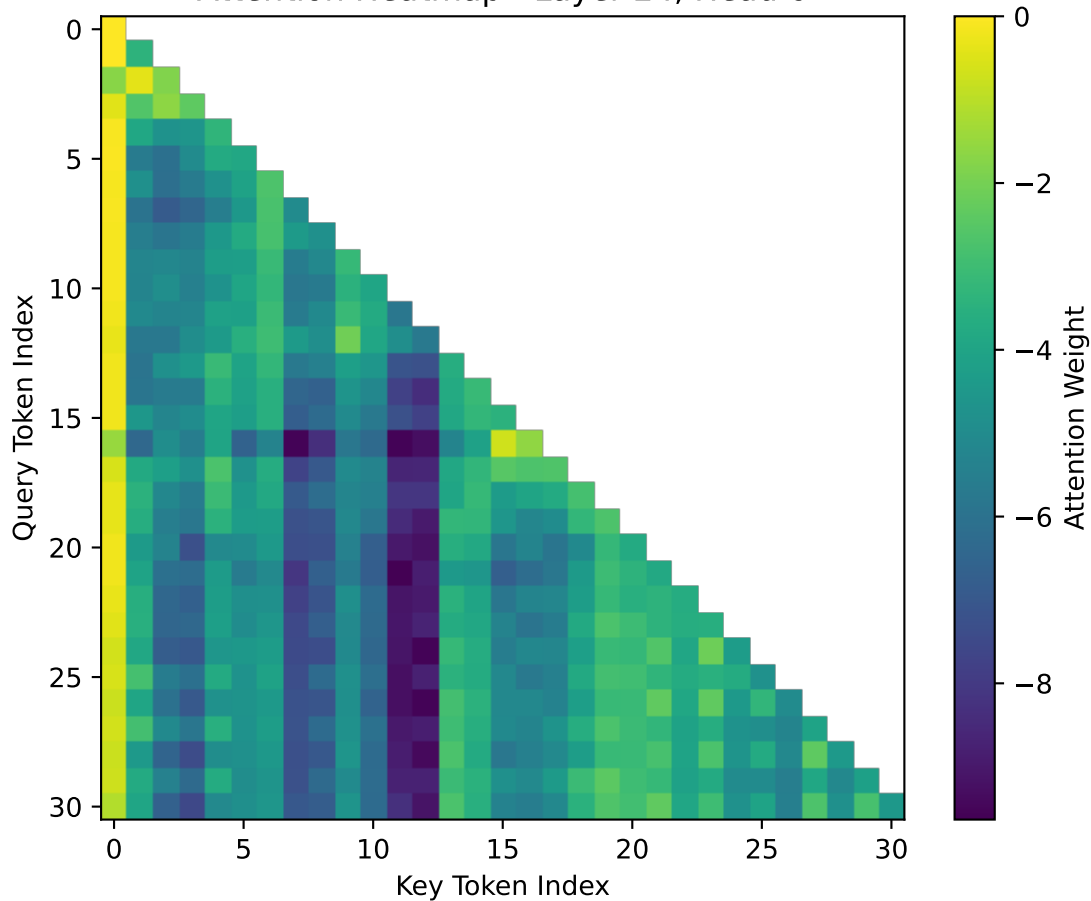
Attention Heatmap - Layer 24, Head 6
