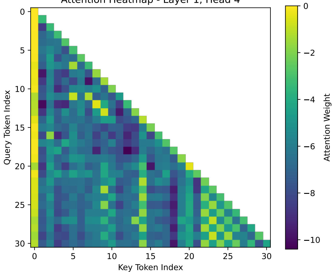
Attention Heatmap - Layer 1, Head 4
