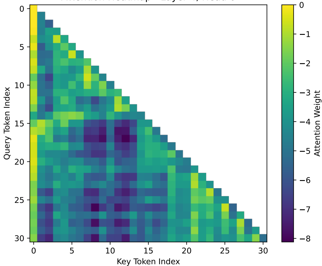
Attention Heatmap - Layer 4, Head 6
