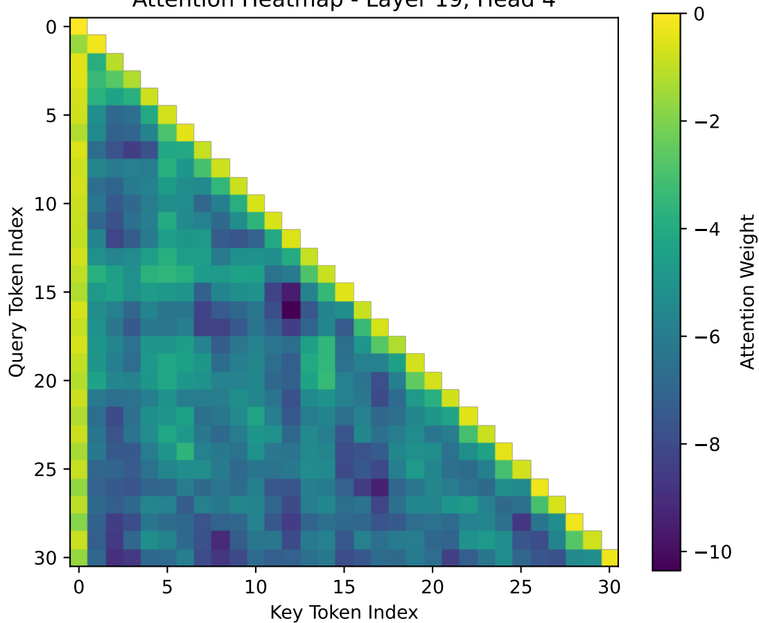
Attention Heatmap - Layer 19, Head 4
