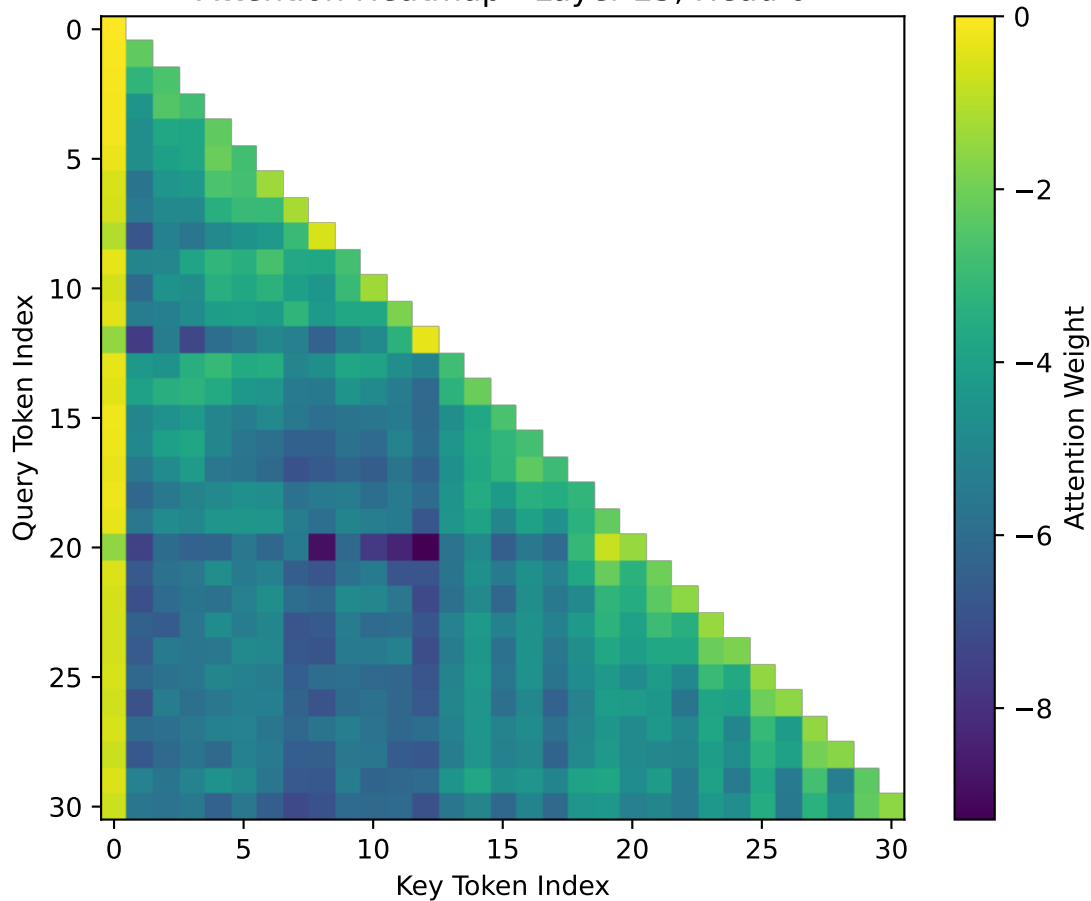
Attention Heatmap - Layer 25, Head 0
