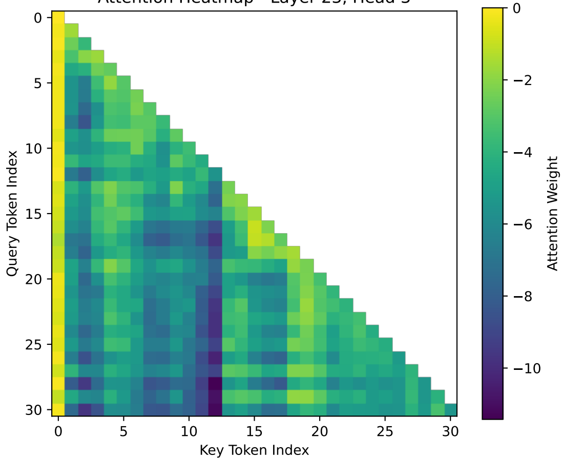
Attention Heatmap - Layer 23, Head 3
