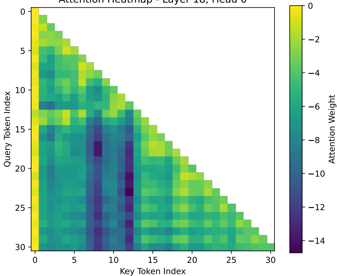
Attention Heatmap - Layer 18, Head 0
