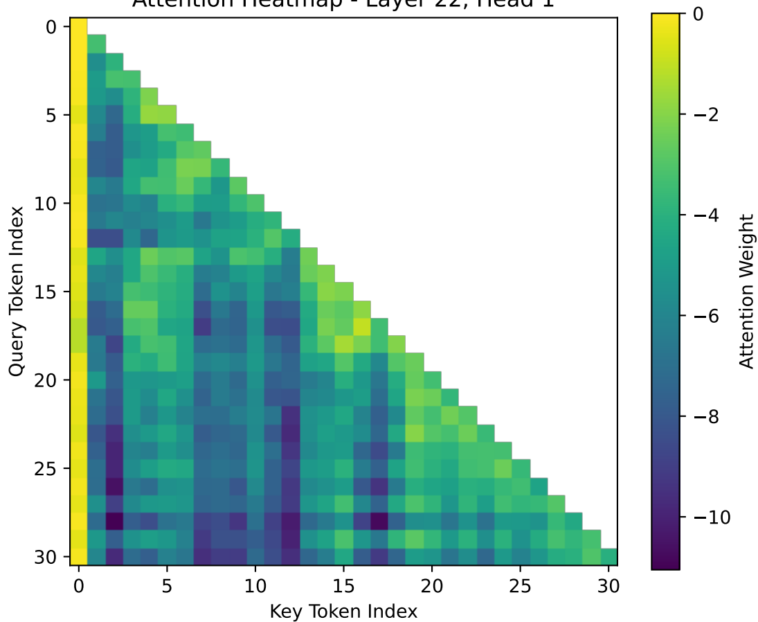
Attention Heatmap - Layer 22, Head 1
