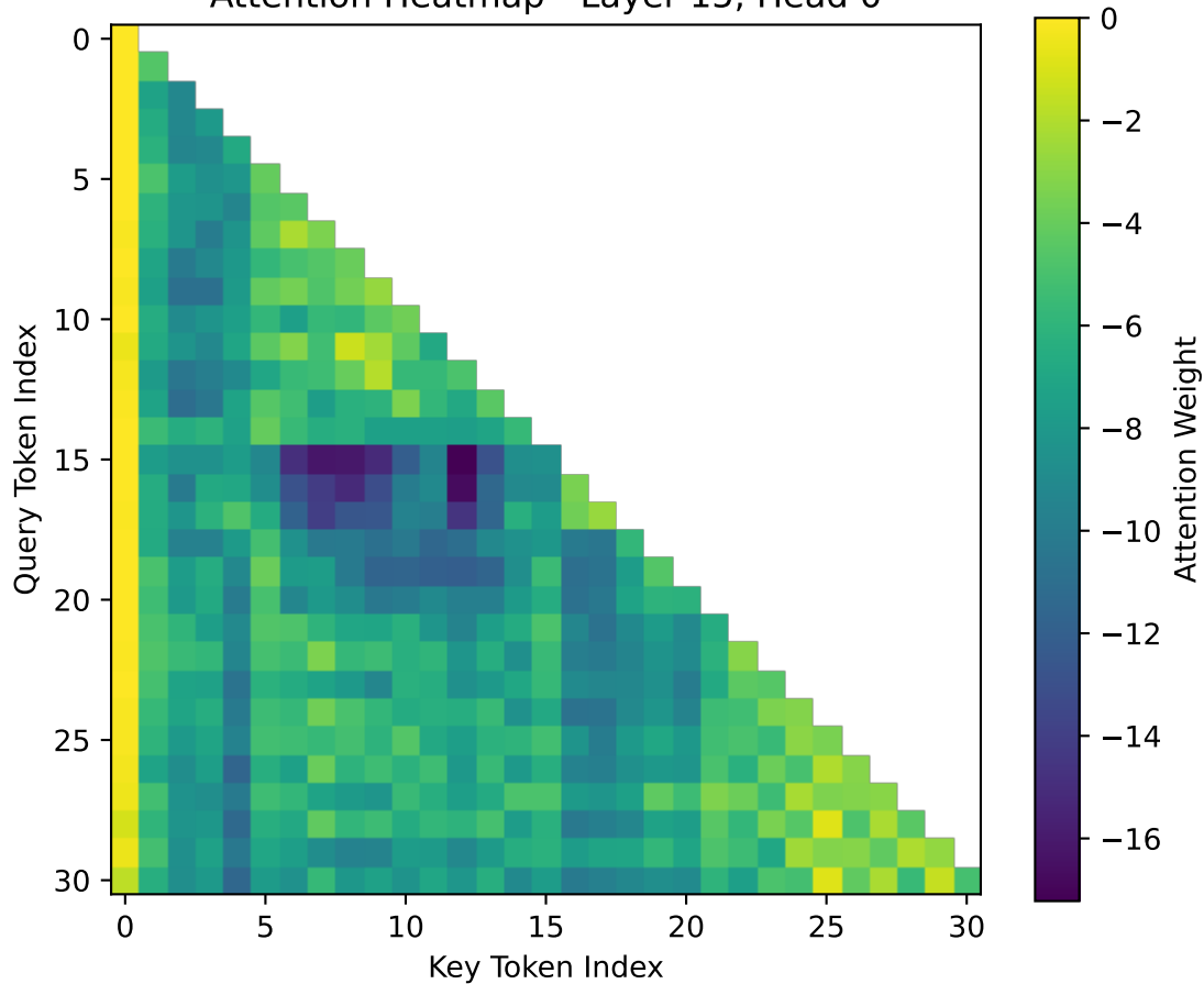
Attention Heatmap - Layer 15, Head 0
