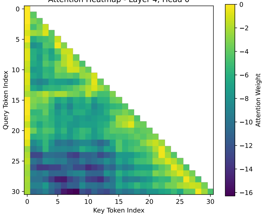
Attention Heatmap - Layer 4, Head 0
