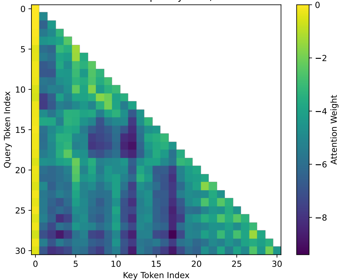
Attention Heatmap - Layer 20, Head 7
