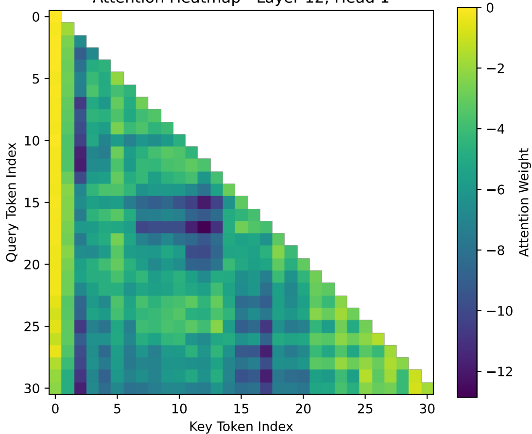
Attention Heatmap - Layer 12, Head 1
