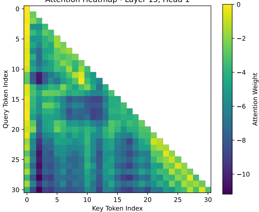
Attention Heatmap - Layer 15, Head 1
