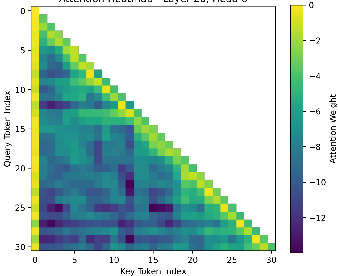
Attention Heatmap - Layer 20, Head 0
