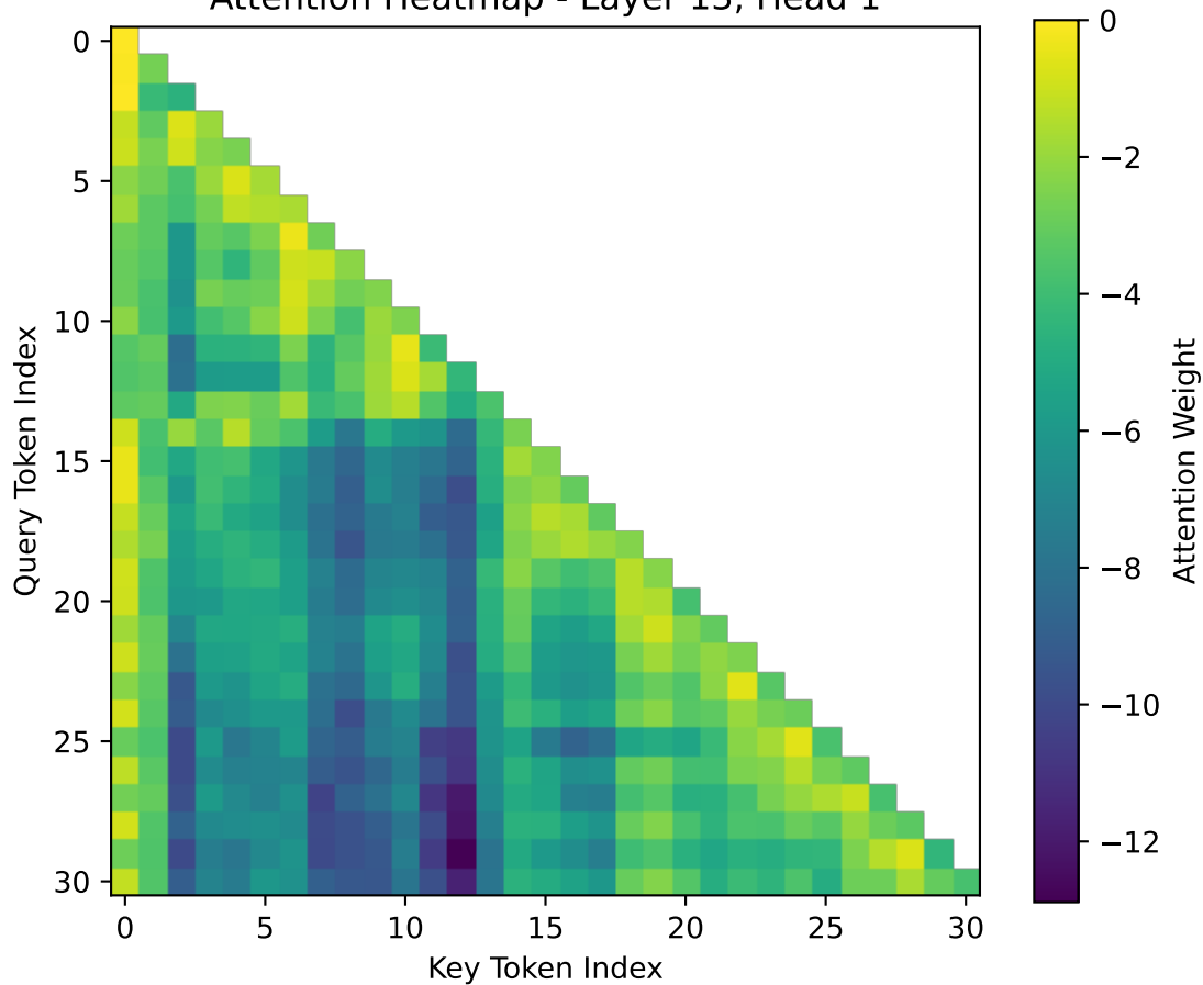
Attention Heatmap - Layer 13, Head 1
