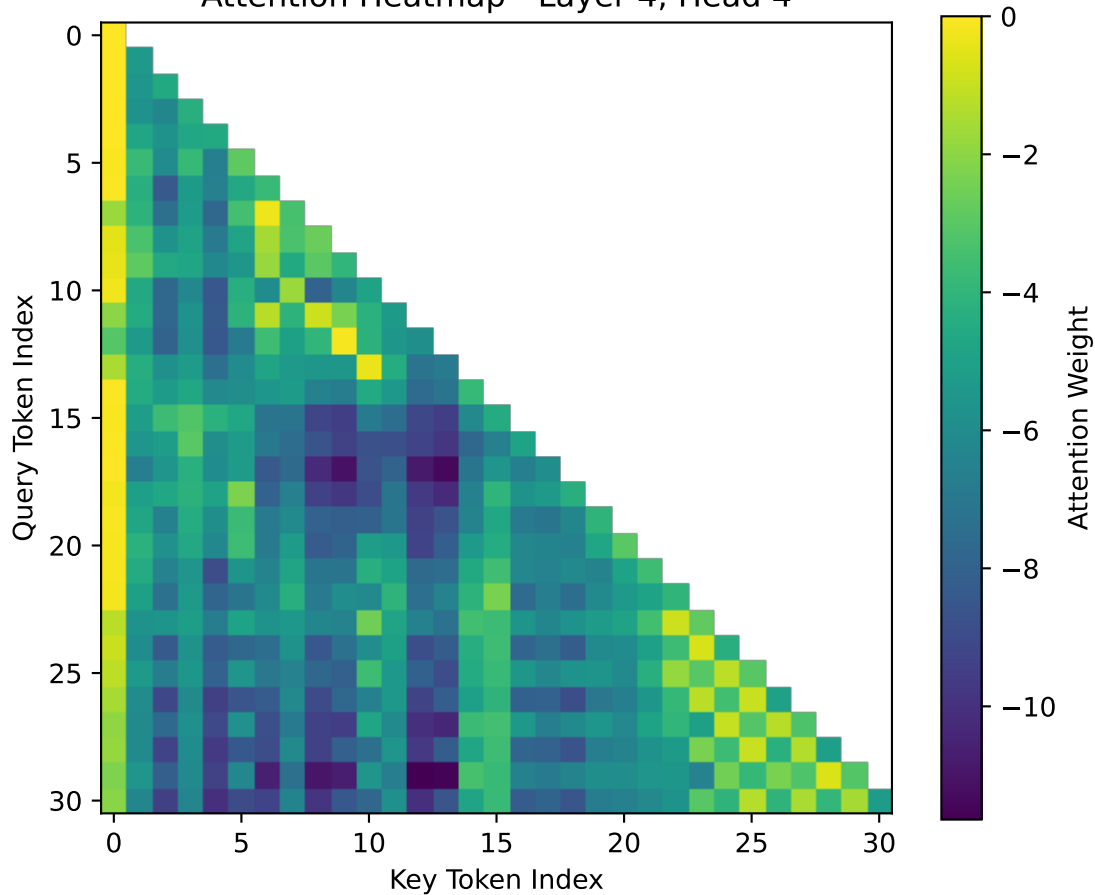
Attention Heatmap - Layer 4, Head 4
