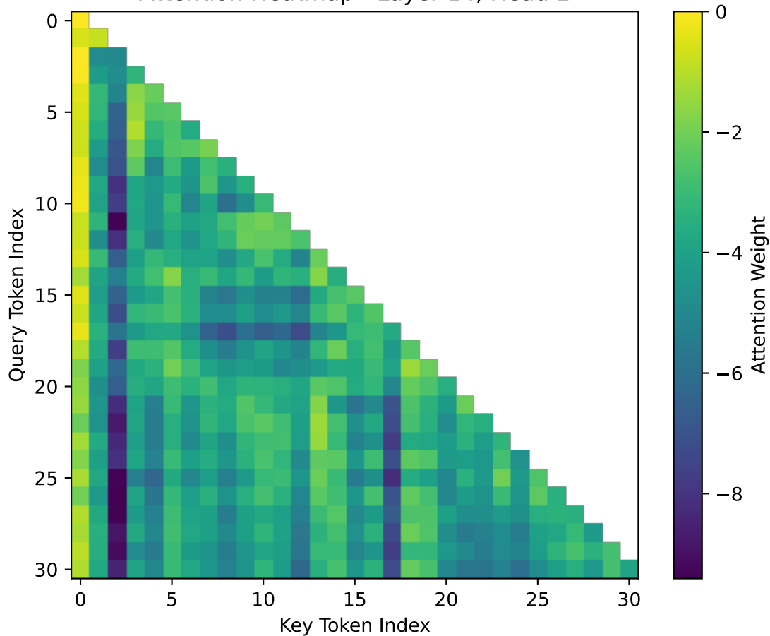
Attention Heatmap - Layer 14, Head 2
