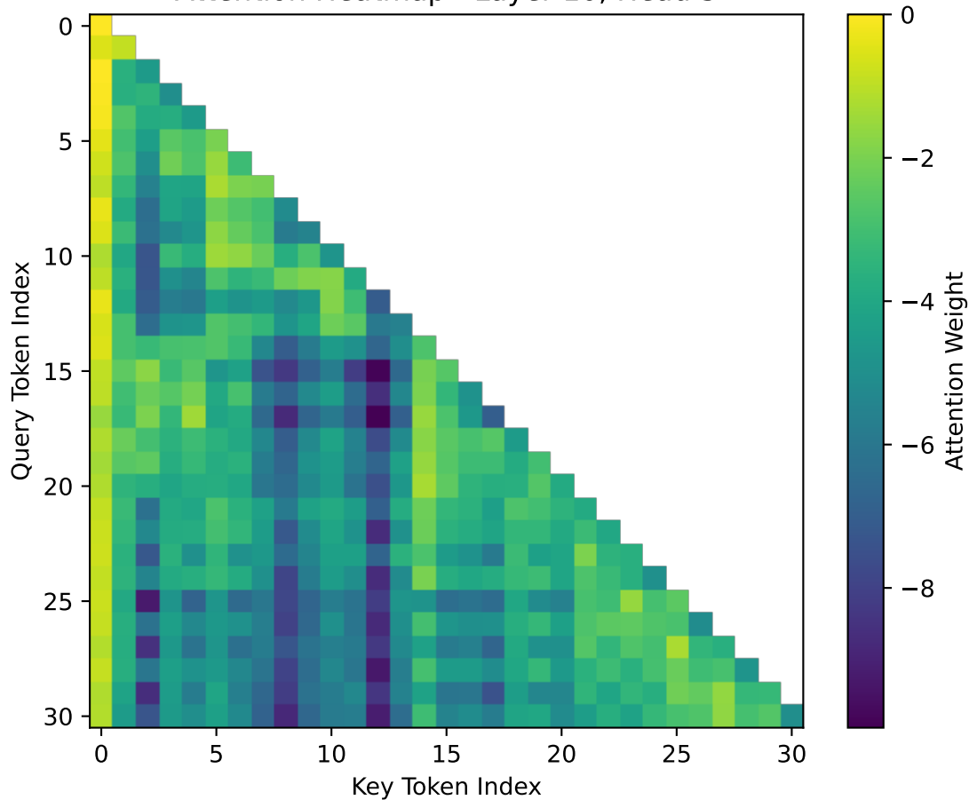
Attention Heatmap - Layer 10, Head 3
