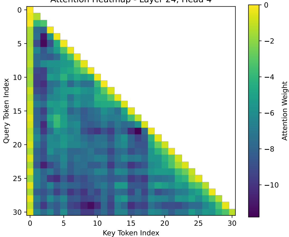
Attention Heatmap - Layer 24, Head 4
