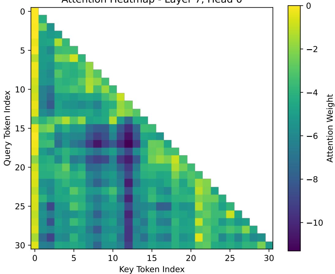
Attention Heatmap - Layer 7, Head 0
