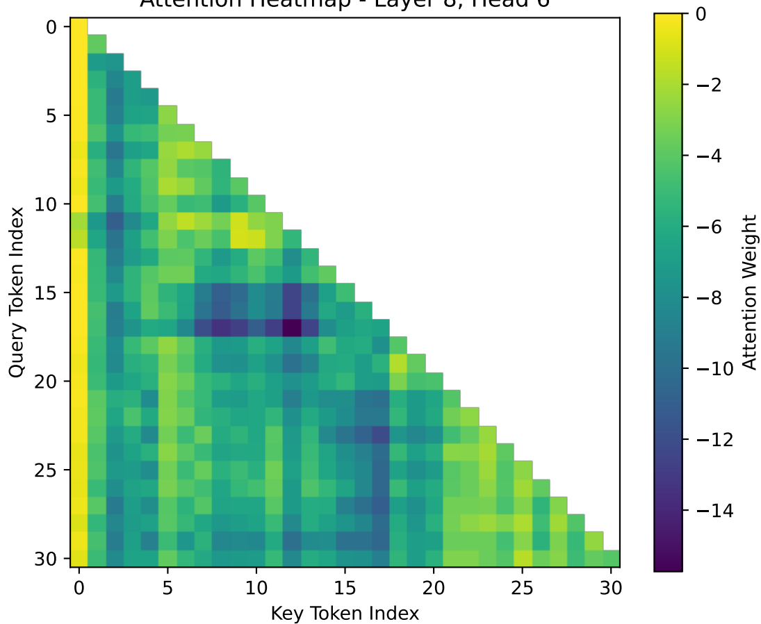
Attention Heatmap - Layer 8, Head 6
