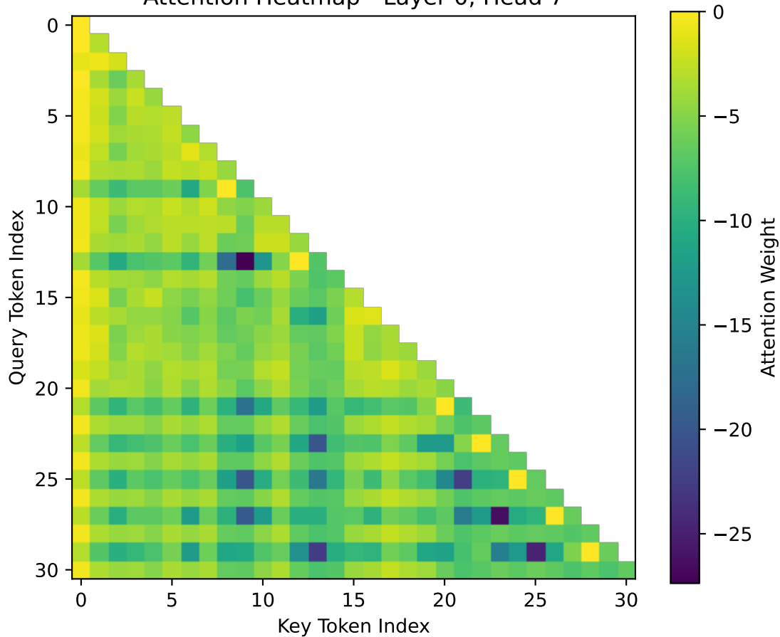
Attention Heatmap - Layer 0, Head 7
