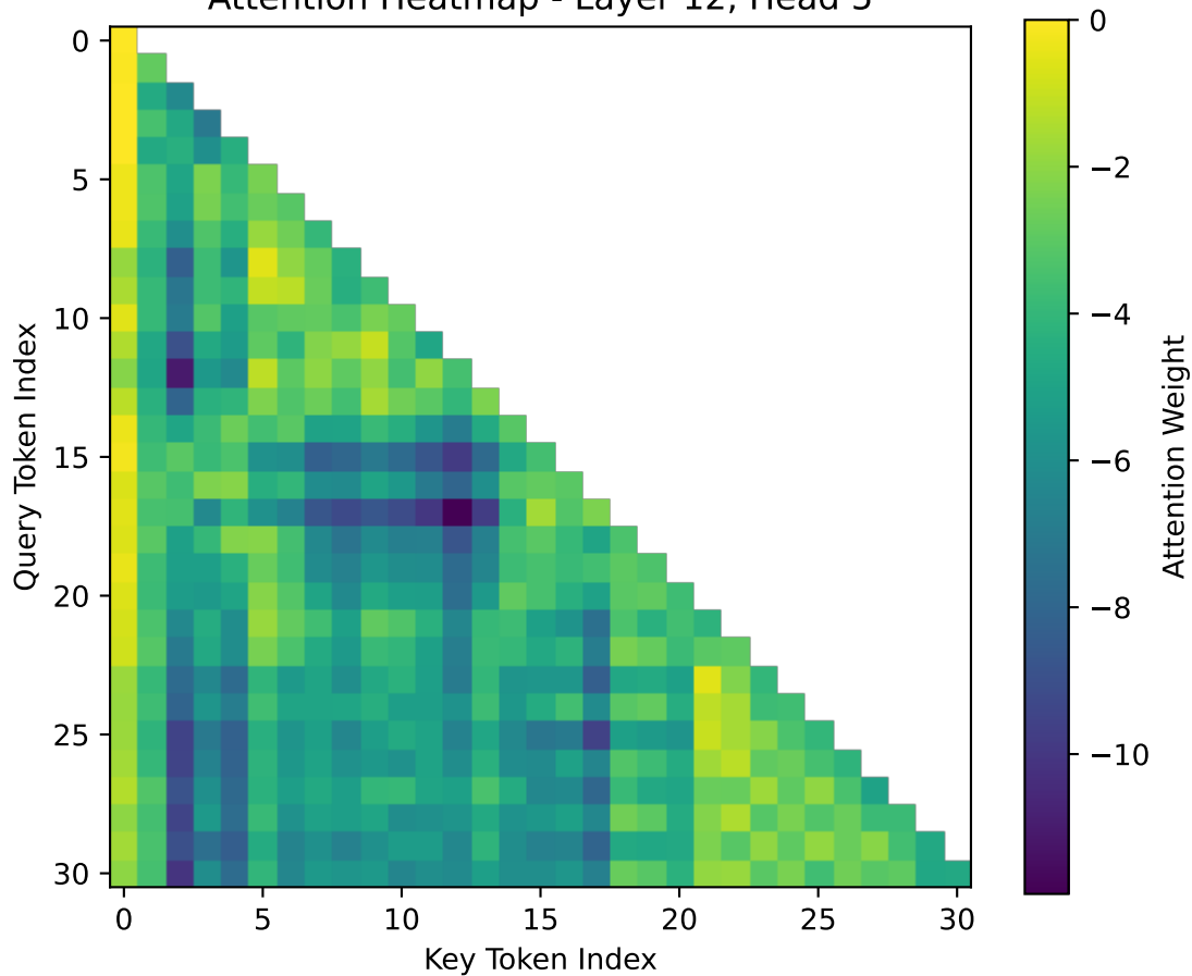
Attention Heatmap - Layer 12, Head 5
