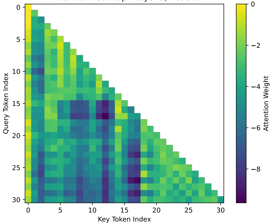
Attention Heatmap - Layer 9, Head 2
