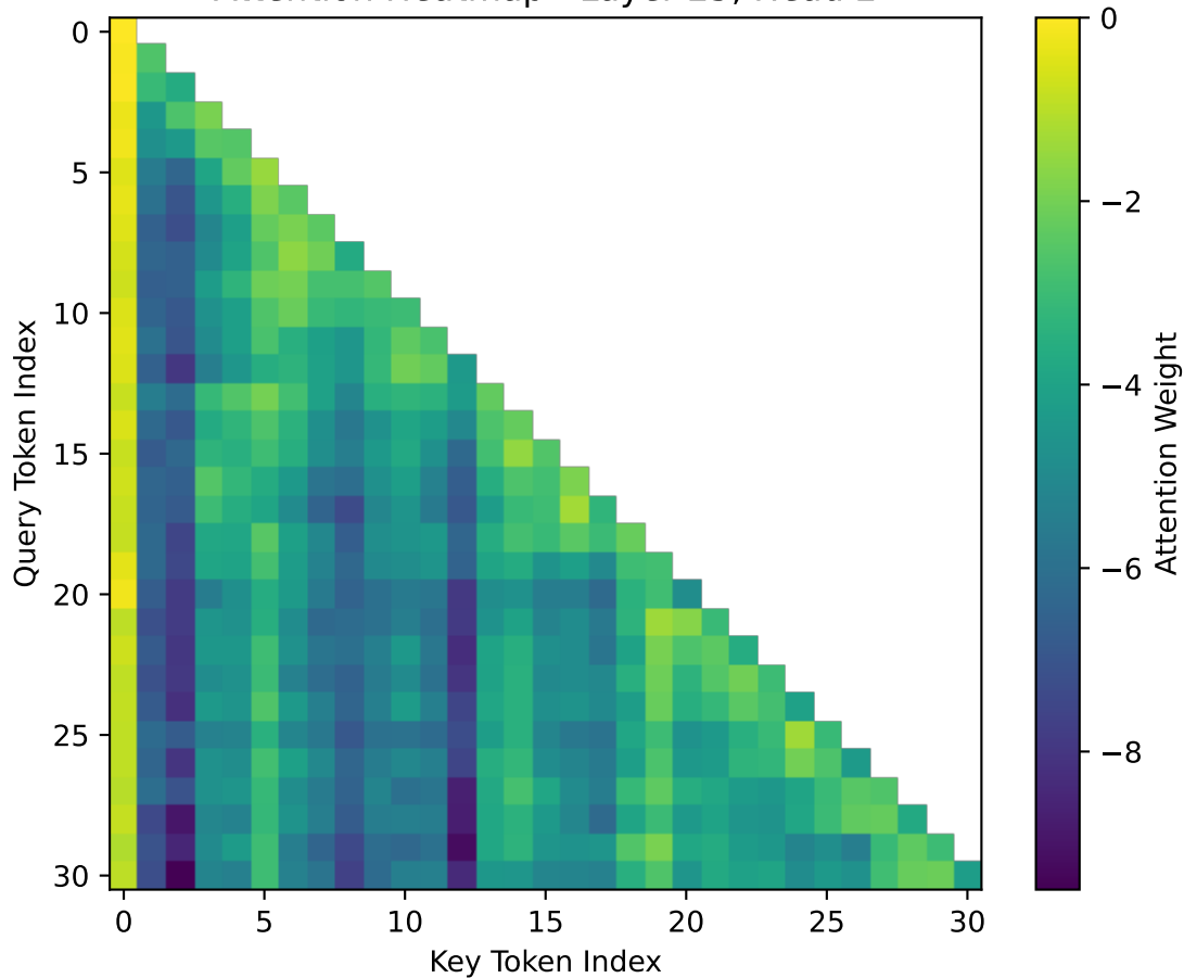
Attention Heatmap - Layer 25, Head 2
