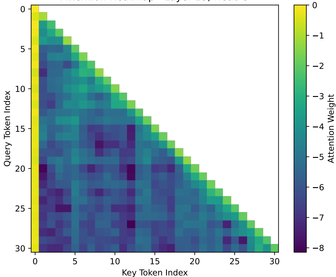
Attention Heatmap - Layer 25, Head 5
