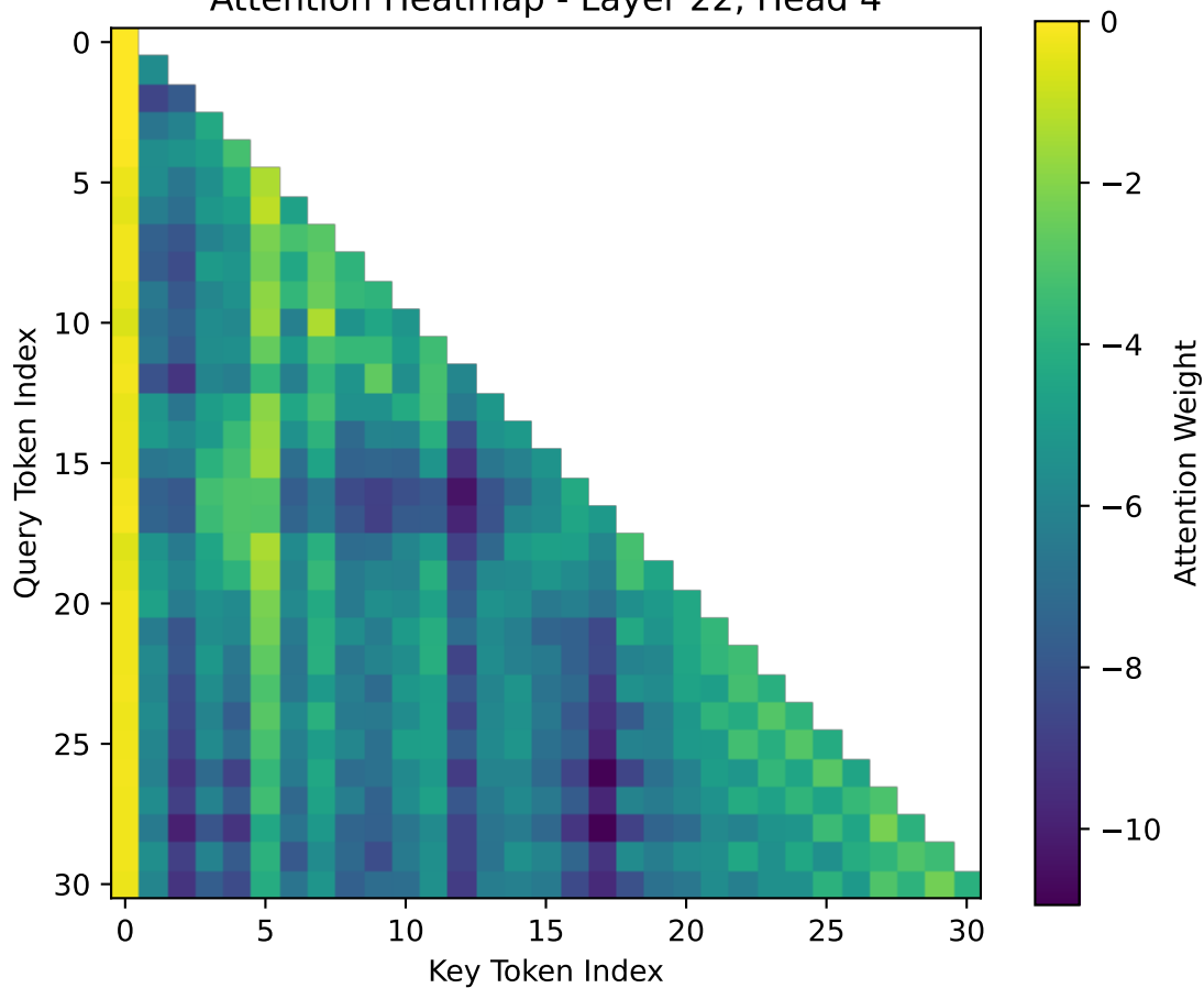
Attention Heatmap - Layer 22, Head 4
