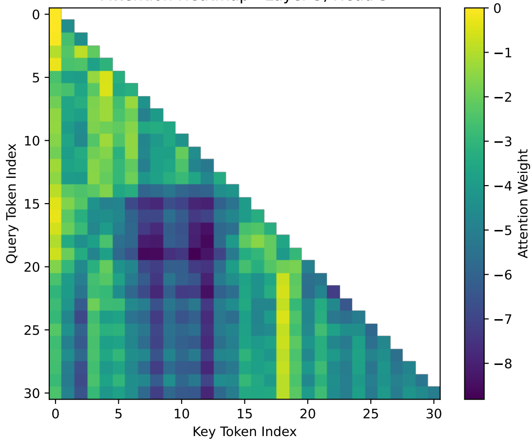
Attention Heatmap - Layer 5, Head 3
