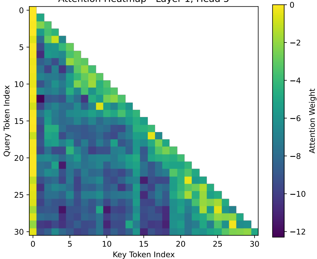
Attention Heatmap - Layer 1, Head 5
