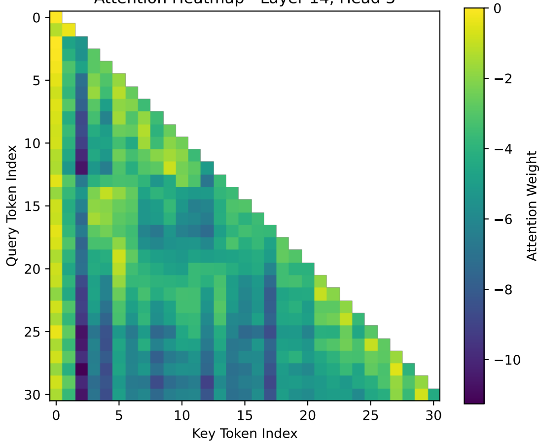
Attention Heatmap - Layer 14, Head 3
