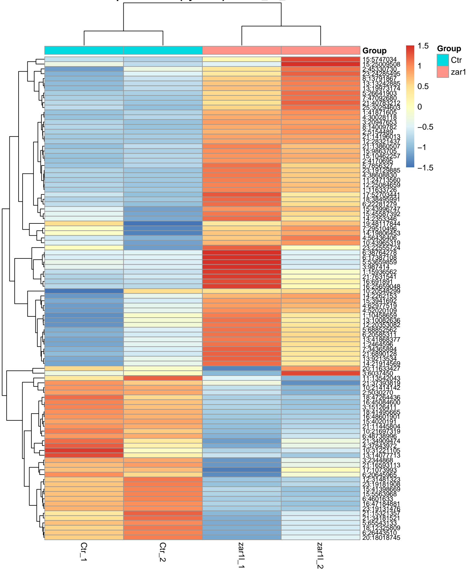
Top 100 DMRs (by delta) - zar1l_vs_Ctr
