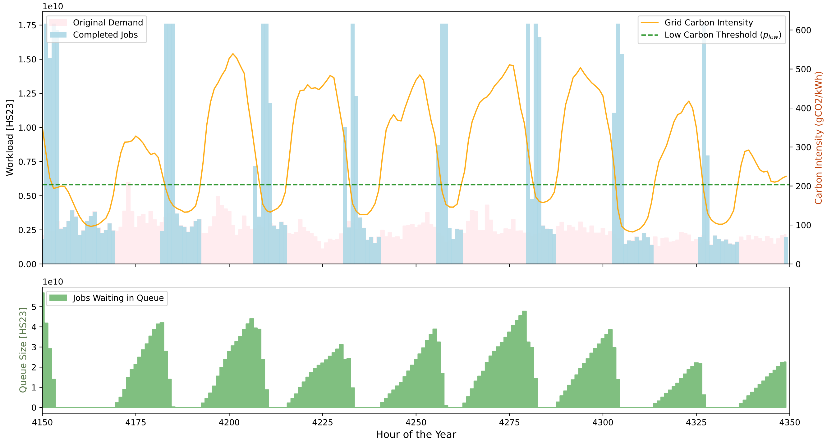
Germany: Execution vs Queue Backlog (Hours 4150-4350)
