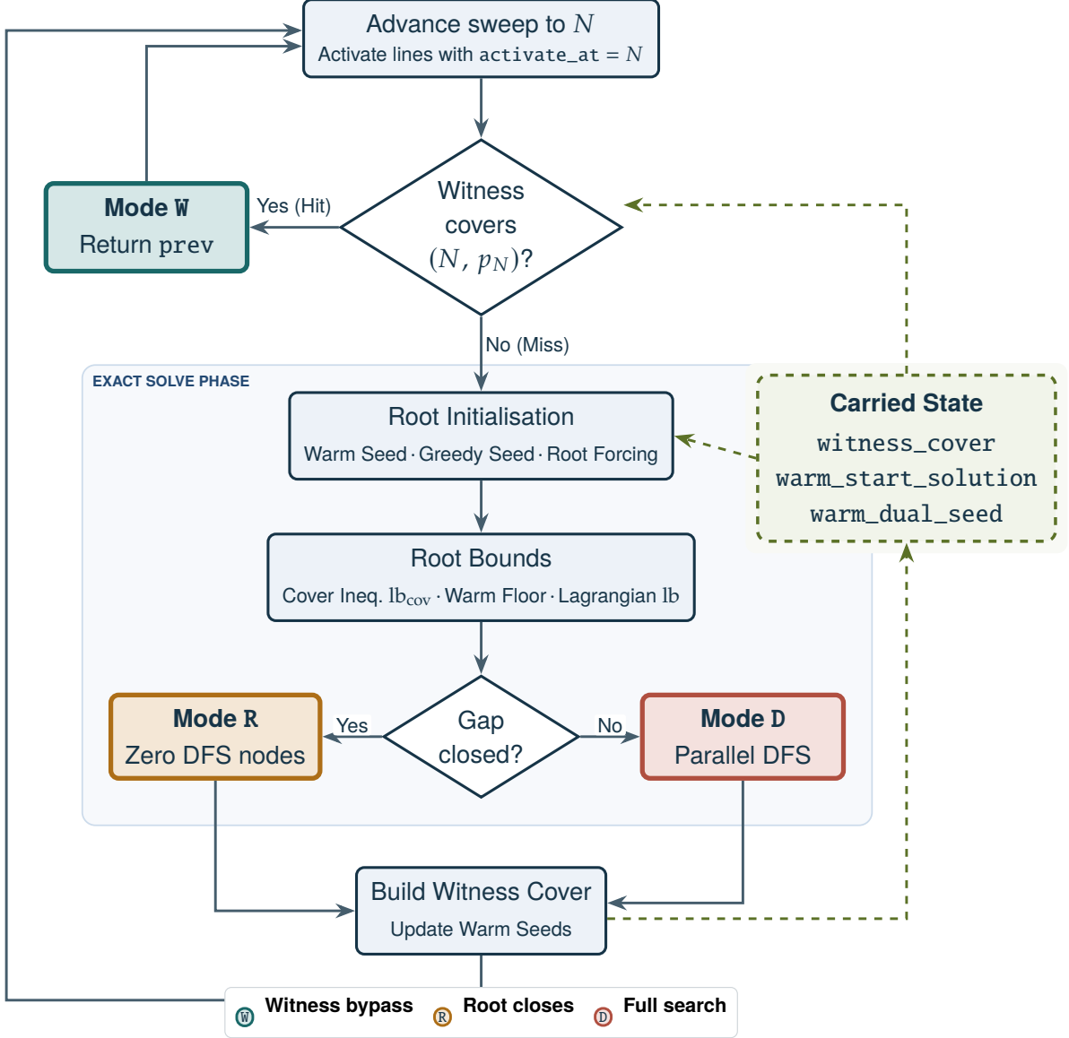
Figure 4: Algorithm architecture and carried-state propagation across the incremental sweep. At each step N the driver appends to active_ids every heavy line whose activate_at equals N , then evaluates the carried witness_cover . A hit ( Mode W ) bypasses the exact solver entirely and returns prev immediately. On a miss the driver calls solve_exact() , which constitutes the exact solve phase : it initialises the root node from the carried warm_start_solution and warm_dual_seed , computes root bounds from the cover inequality, the previous step’s certified cost, and the Lagrangian bound, and then either closes the gap without DFS ( Mode R , zero nodes counted) or launches the parallel frontier and DFS ( Mode D ). Both exact modes conclude by rebuilding the witness cover and writing back updated warm seeds for the next step. Dashed arrows show the three carried-state channels.
