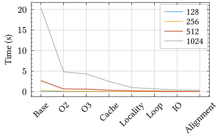
Graph 3: Illustration of all the different sizes through all the taken steps.
