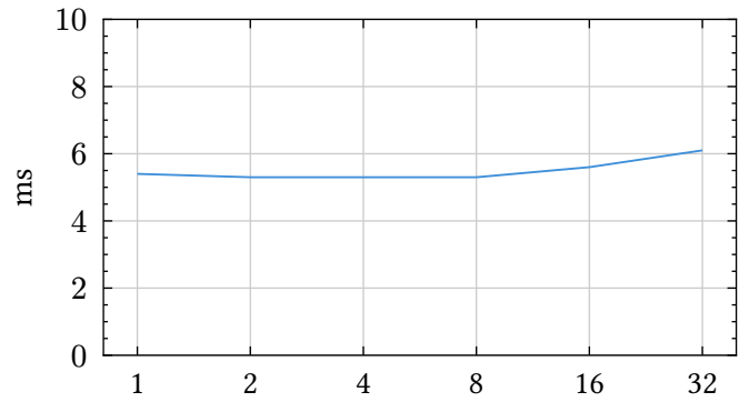
Graph 4: Illustration of time over different thread counts for size 128.
