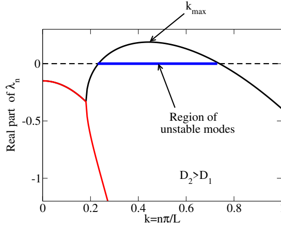
Figure 4.6: Dispersion plot: Real part of the eigenvalues, \lambda_n as a function of k = n\pi/L . D_2 = 10D_1 , I = (1/10)^{3/2} , and \epsilon = 1 .
