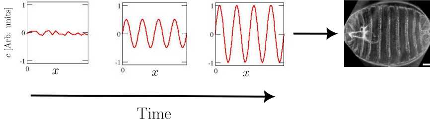
Figure 1.2: Turing structure. From random initial concentration, (a), a concentration gradient emerges spontaneously, (b), and reaches a static situation of varying gradient (structure) (c). The Turing structure can model the biological morphology observed in the embryo of the fruit fly (d).
