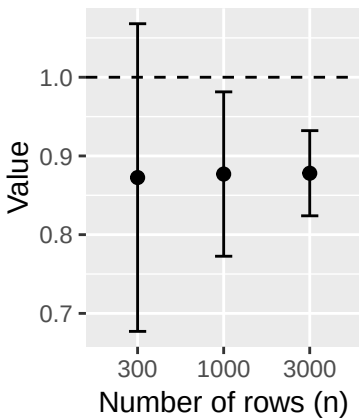
S3 - \hat{\beta}_4
