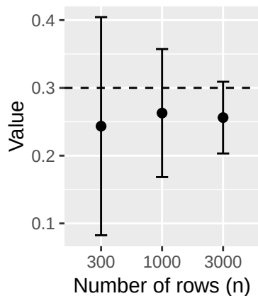
S3 - \hat{\pi}_2
