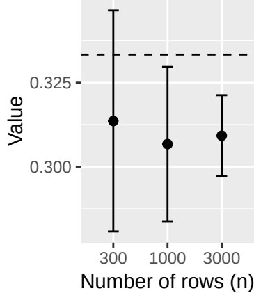
S6 - \hat{\pi}_2
