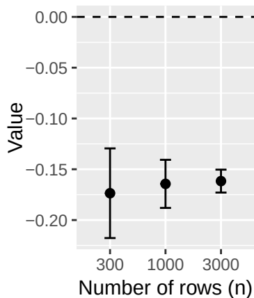
S6 - \hat{\beta}_3
