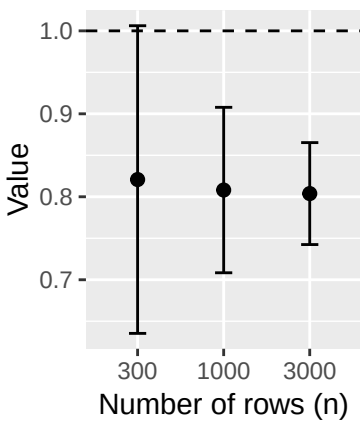
S6 - \hat{\beta}_4
