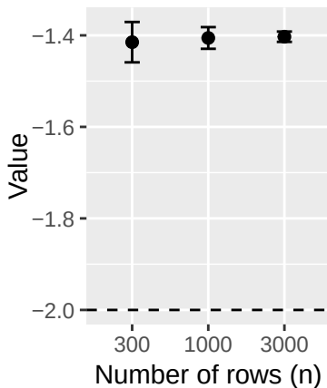
S6 - \hat{\beta}_2
