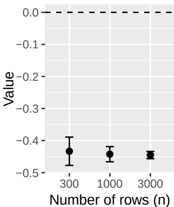
S6 - \hat{\beta}_1
