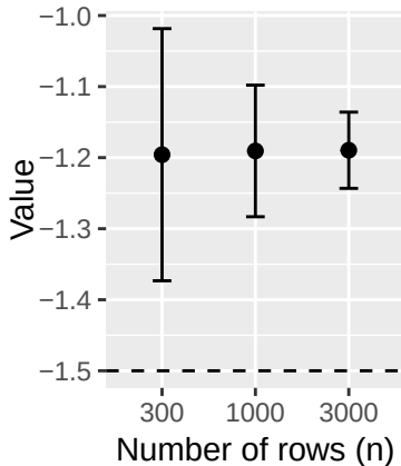
S6 - \hat{\pi}_1
