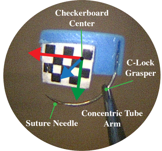
Fig. 3. The needle is rigidly fixed to the checkerboard such that the transform between the centers can be measured, enabling ground truth needle pose measurements, for calibration and accuracy tests.
