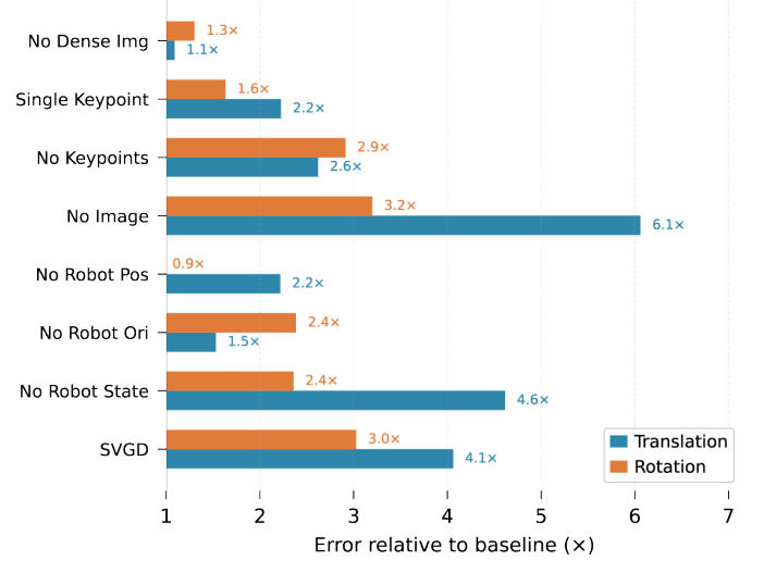
Fig. 5. A bar graph breakdown of the error degradation about the translational and rotational under the given ablation.
