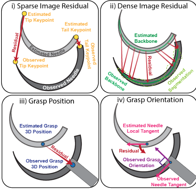
Fig. 2. Sources of information used for monocular needle pose estimation and the geometric reach of their corresponding residuals: (i) image keypoints at the needle tip and tail, (ii) needle backbone segmentation, (iii) the C-Lock rigidly fixes the needle at a known grasp point, and (iv) the C-Lock enforces a perpendicular relationship between the gripper axis and the needle tangent at the grasp location.
