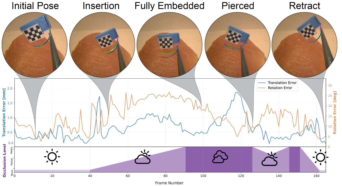
Fig. 7. Graph of translation (blue) and rotation (orange) errors during suturing, with representative images shown at key frames. A graph of the occlusion level is graphed below, with icons illustrating the levels of none, partial, and heavy occlusion. The graph illustrates how occlusion increases during piercing until the tip emerges on the other side of the tissue. Occlusion then decreases as the needle is retracted until it fully exits the tissue.
