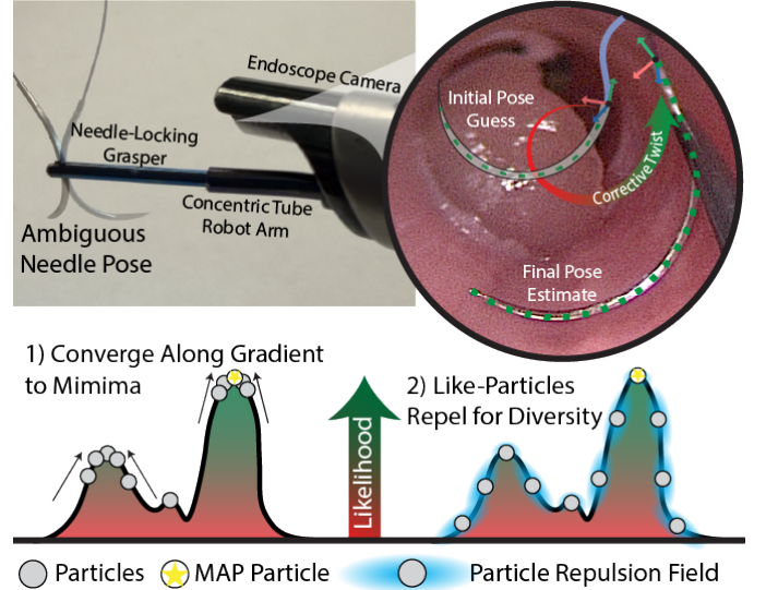
Fig. 1. Conceptual illustration of the proposed monocular needle tracking framework. (Top) Image and robot-based observations define an error over the needle pose estimate, which is iteratively solved for with PinPoint. The isometric robot view highlights the inherent depth ambiguity of monocular needle pose estimation, where multiple 3D configurations can produce similar image projections. (Bottom) PinPoint uses Stein Variational Inference, which represents the posterior over needle poses using a set of interacting particles. Particles are deterministically transported toward high-probability regions of the posterior while repulsive interactions prevent collapse and preserve multimodal hypotheses. The maximum a posteriori (MAP) particle corresponds to the most likely needle pose estimate.
