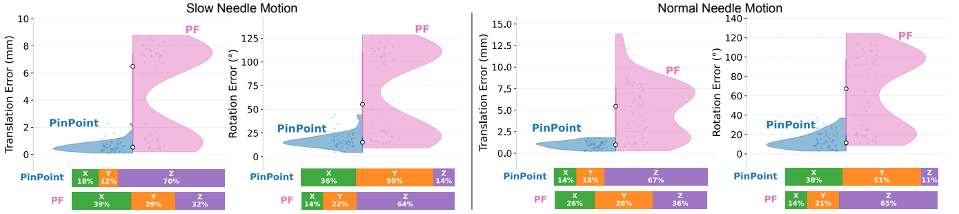
Fig. 4. Distribution of translational and rotational pose estimation errors for PF and PinPoint across motion speeds. Each panel shows a half-violin with overlaid scatter for PF (pink, right) and PinPoint (blue, left), with white circles indicating the median. Stacked bars below each panel show the fractional contribution of each component axis (X: green, Y: orange, Z: purple) to total error. In both (Left) slow-speed trials and (Right) normal-speed trials, we show the rotational and translational errors.
