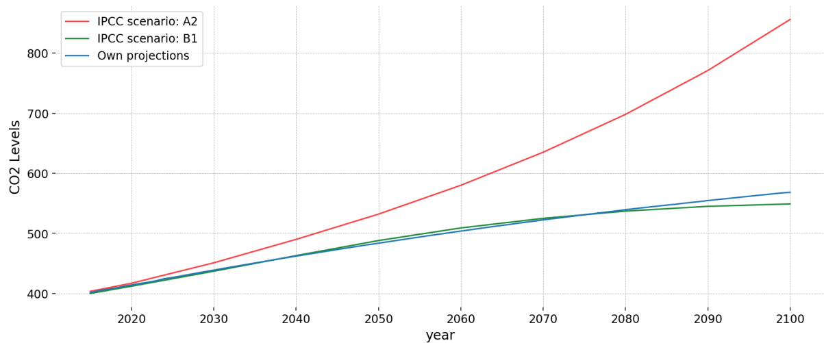
Figure 20: IPCC and own projections of atmospheric CO 2
