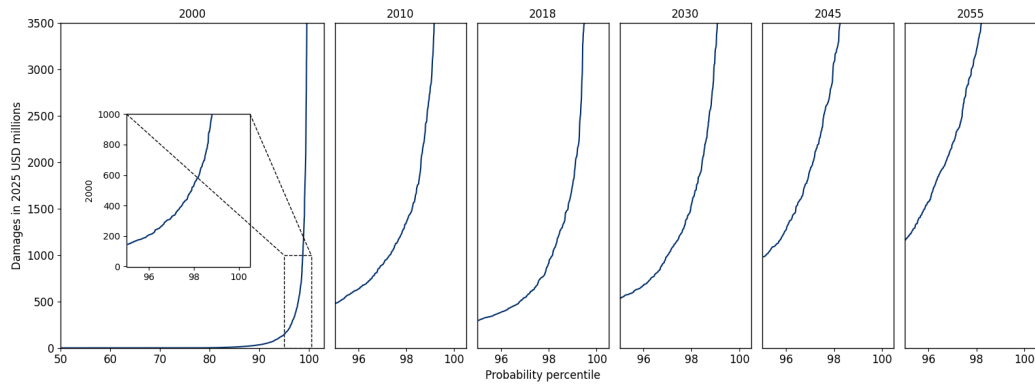
Figure 31: CR damage curves
