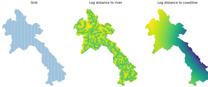
Figure 17: Laos grid with distance to rivers and coastlines
