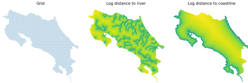
Figure 16: Costa Rica grid with distance to rivers and coastlines
