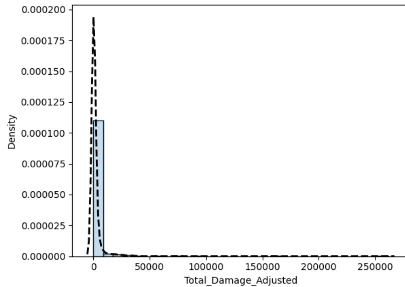
Figure 7: Kernel density for yearly damages of hydrometeorological disasters
