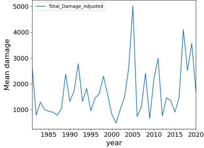
Figure 8: Historical trend of yearly damages of hydrometeorological disasters
