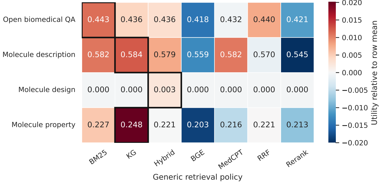
Mol-Instructions
