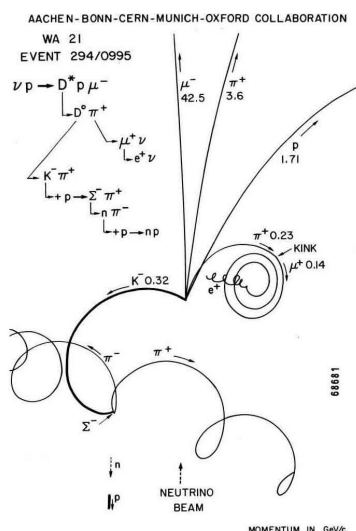
(b) D-meson bubble chamber tracks
