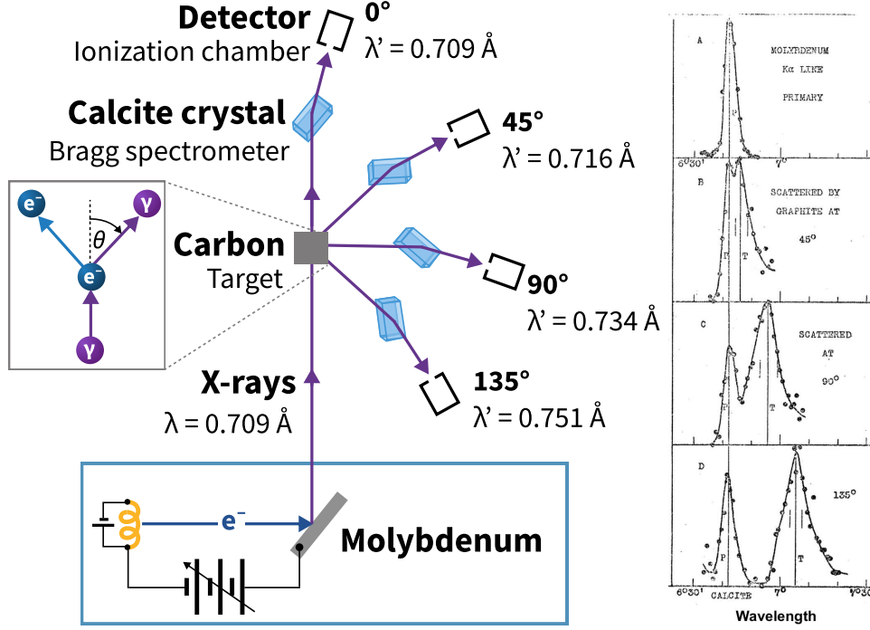
Figure 6: Compton scattering: a cathode-ray tube generates the “K- \alpha ” line of 0.709 \text{ \AA} X-rays from molybdenum, which strike a carbon graphite target and scatter into a calcite crystal spectrometer. Dots show the measured data at various scattering angles, where the classical Thomson (quantum Compton) prediction is marked P (T) [12].
