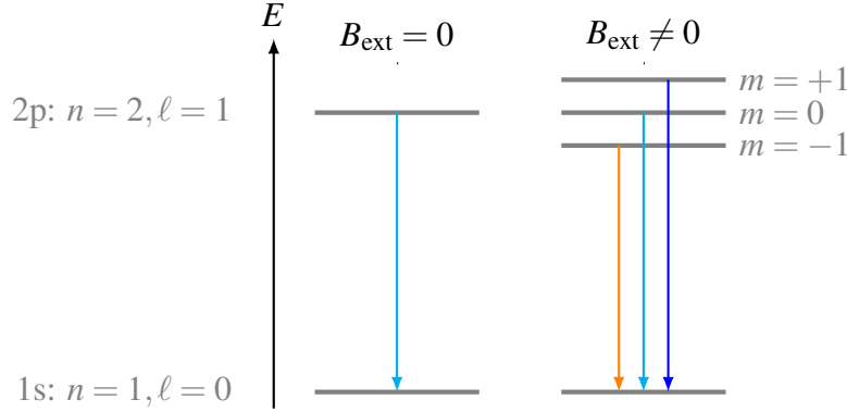
Figure 39: Schematic energy diagram of normal Zeeman splitting for B_{\text{ext}} on and off.
