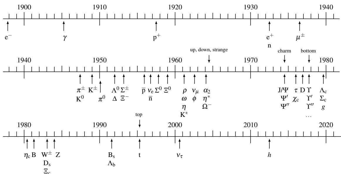
Figure 45: Timeline of particle discoveries. Displayed are various fundamental SM particles and composite hadrons. Figure: adapted from Ref. [58]
