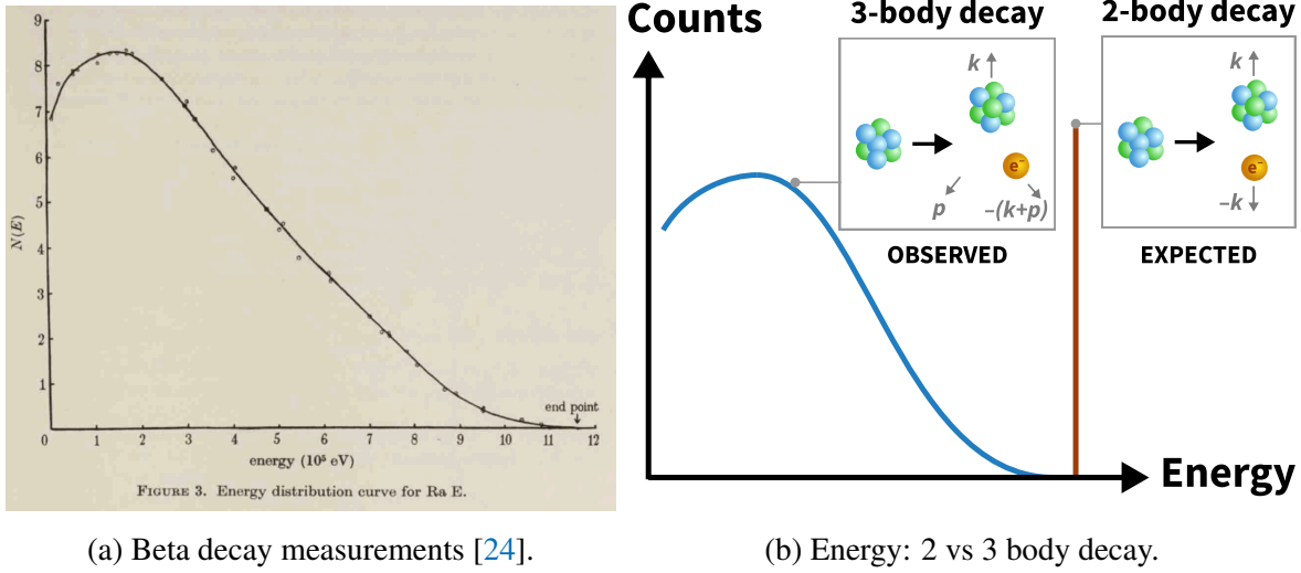
Figure 13: Beta decay spectrum. The early expectation of a two-body decay sees the child nucleus and electron having equal and opposite momentum, resulting in a sharp peak in energy from equation (2.7). The observed three-body decay features an additional anti-neutrino with momentum \mathbf{p} smearing out the observed spectrum into a continuum.
