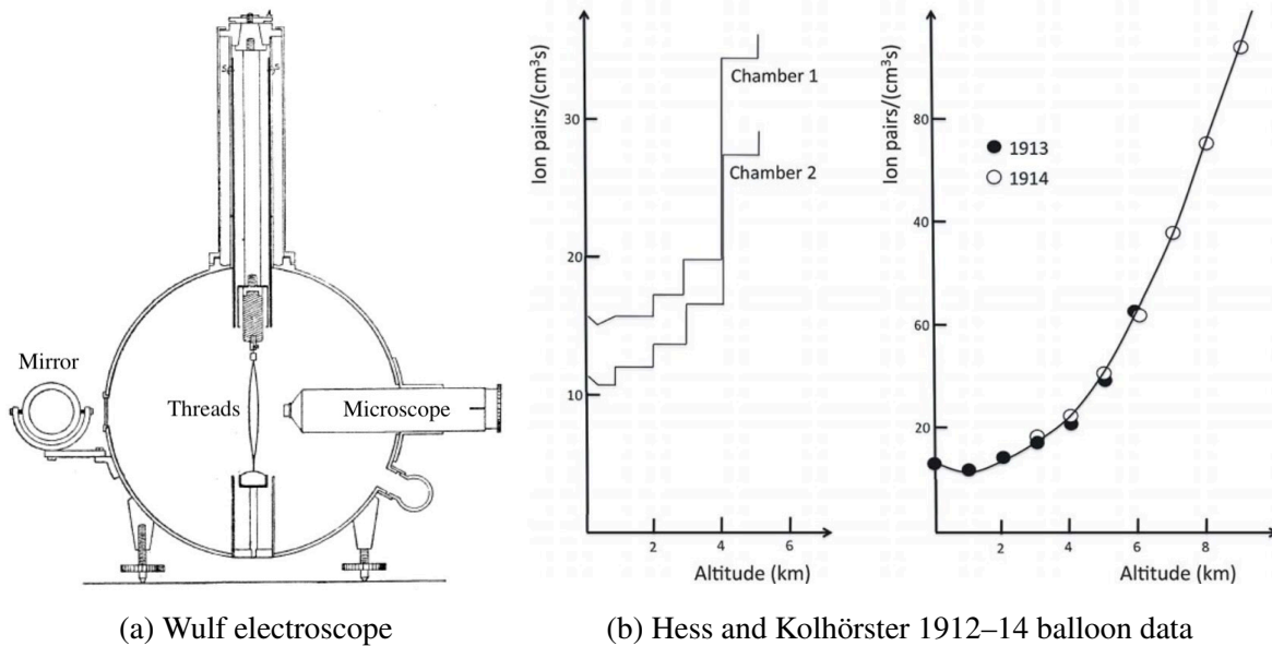
Figure 16: Historical measurements of cosmic-ray flux. Electroscopes measure ionisation by observing metallic threads under tension during electrostatic discharge. This enabled balloon-borne measurements by Hess (1912) and Kolhörster (1913), illustrating the increase in flux with altitude. Images: Wulf, Phys. Zeit. 1 (1909) 152 , Ref. [30].
