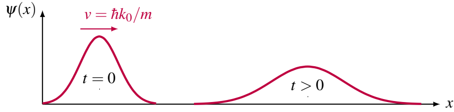
Figure 22: Sketch of Gaussian wavepacket moving in free space with speed v = \hbar k_0 / m , whose dispersion (width) and amplitude (height) broadens with time.
