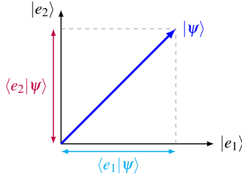
Figure 27: A state vector |\psi\rangle projected onto basis vectors \{|e_1\rangle, |e_2\rangle\} of a Hilbert space.
