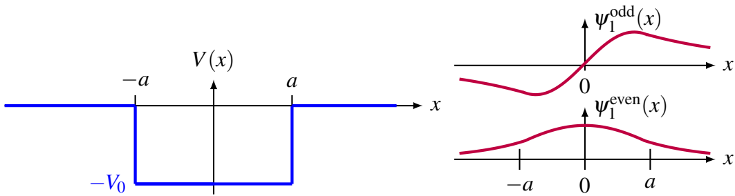
Figure 18: Left: finite-well potential. Right: sketch of first odd/even wavefunctions, which ‘leak’ outside the well |x| > a in striking difference from classical particles in a box.
