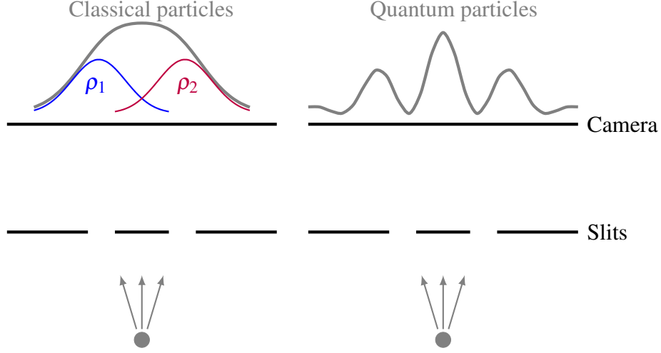
Figure 13: Sketch of double-slit experiment for particles thrown at a barrier with two slits. The classical particle distribution \rho_{1+2} = \rho_1 + \rho_2 is the sum of those for the individual slits \rho_1, \rho_2 . Quantum particle distribution exhibits a wave-like interference pattern.
