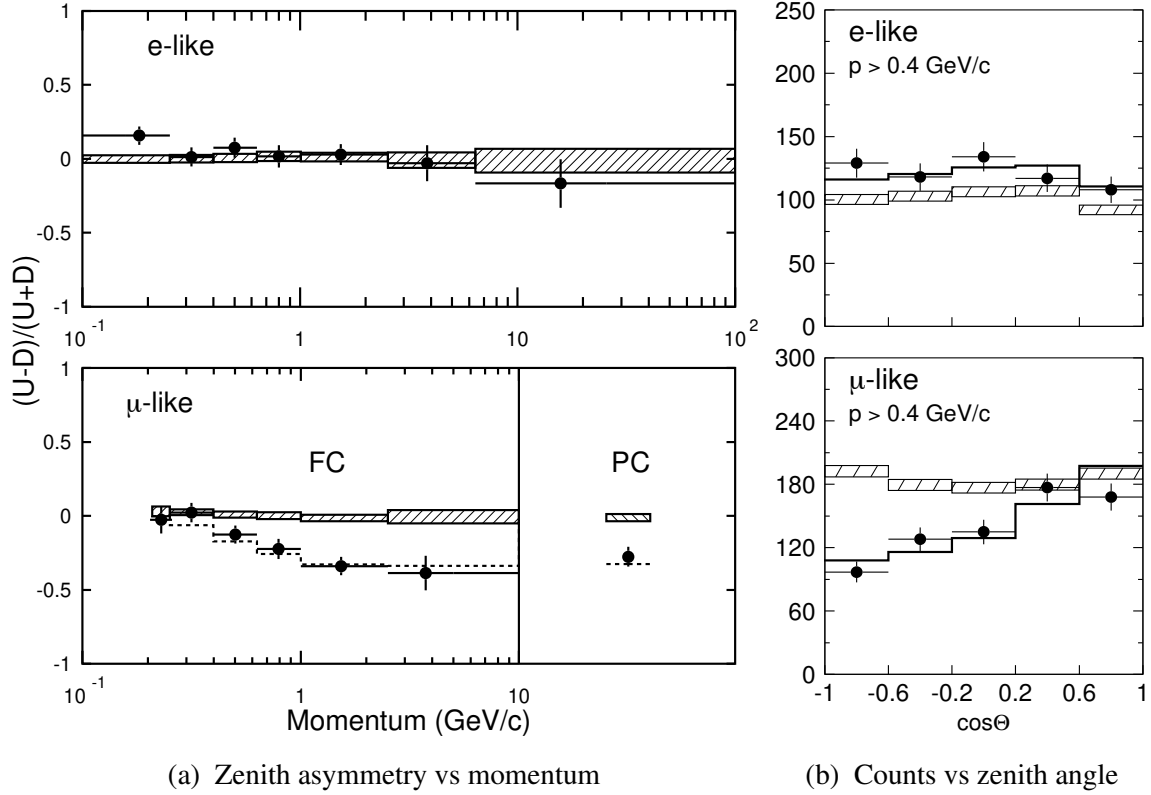
Figure 117: Atmospheric neutrino measurements from the 1998 Super-Kamiokande paper [109]. Hatched boxes show the simulated prediction from the no-oscillation model; lines (dotted on left, solid on right) show the best-fit to a \nu_\mu \rightarrow \nu_\tau oscillation model. Upper (lower) panels show electron-like (muon-like) candidates. A zenith angle of \cos \Theta_Z corresponds to directly overhead, \cos \Theta_Z < 0 is up-going and \cos \Theta_Z > 0 is down-going.
