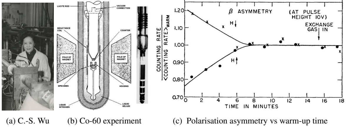
Figure 79: Wu et al. Cobalt-60 experiment. The plot shows the beta asymmetry from the discovery paper [84], which illustrates the magnetic field polarisation up H \uparrow and down H \downarrow vs warm-up time of six minutes. Images: Smithsonian Institute Archives , National Institute of Standards and Technology , Ref. [84].
