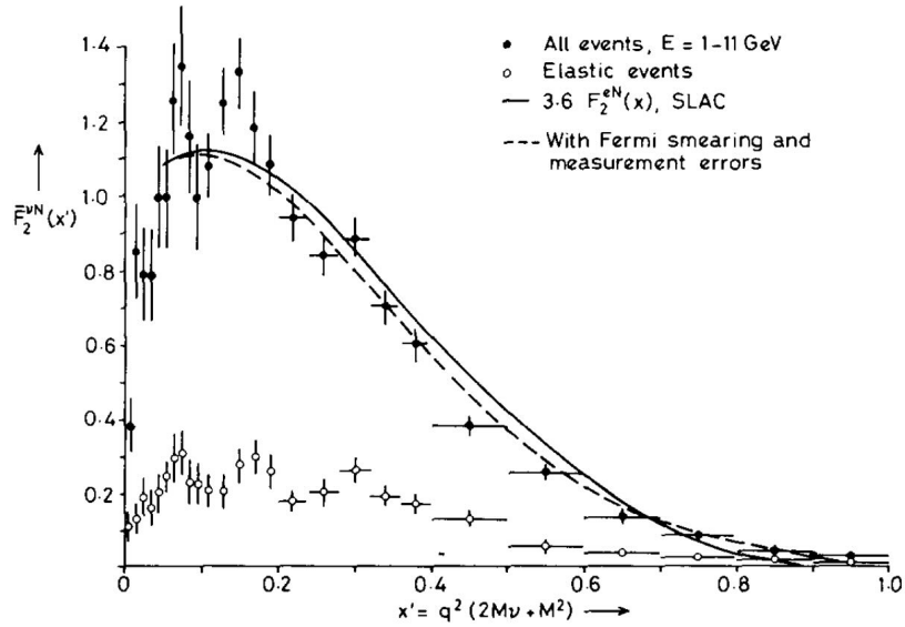
Figure 68: Combined SLAC–Gargamelle data [72] supporting the fractional charges of quarks. The black points are the neutrino-quark data, compared to the lines based on the electron-quark data scaled by 2/(Q_u^2 + Q_d^2) = 18/5 = 3.6 .
