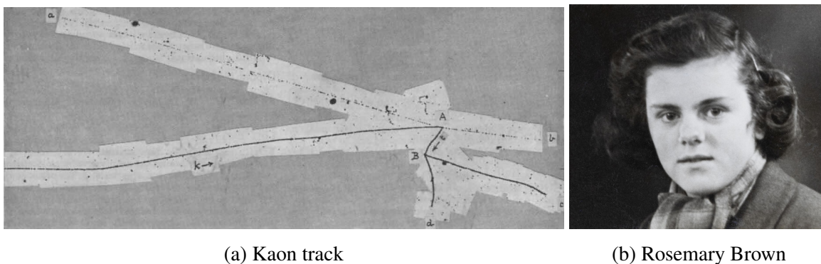
Figure 49: Bristol kaon discovery photo. Kaon track found by W. J. van der Merwe in a photographic plate: V shaped tracks in cosmic ray from Ref. [62]. Photo showing Rosemary Brown who analysed such events.
