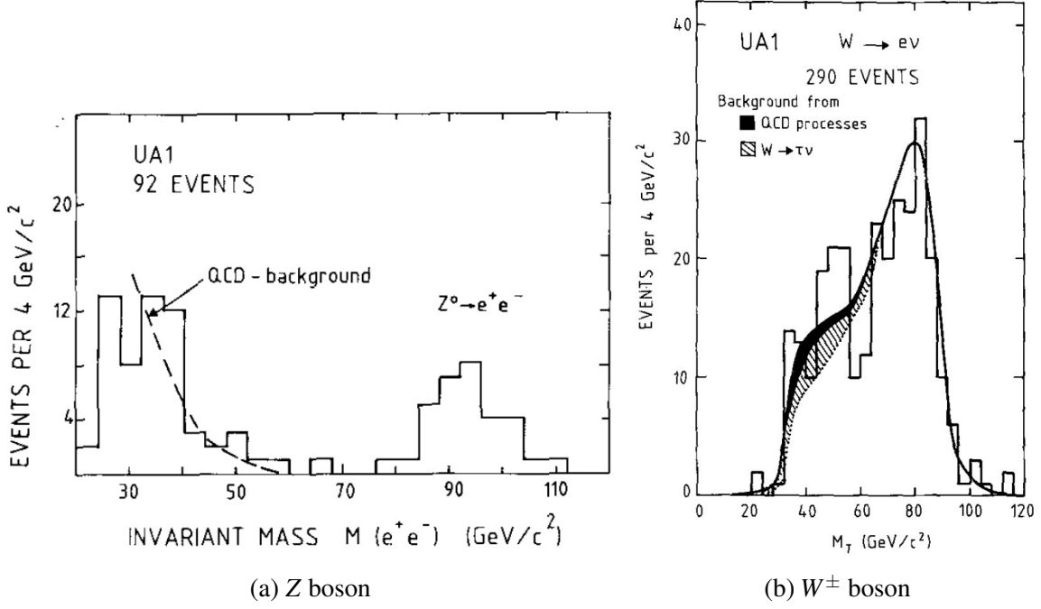
Figure 101: Mass peaks of the W^\pm and Z bosons from larger statistics samples from the UA1 Collaboration [98].
