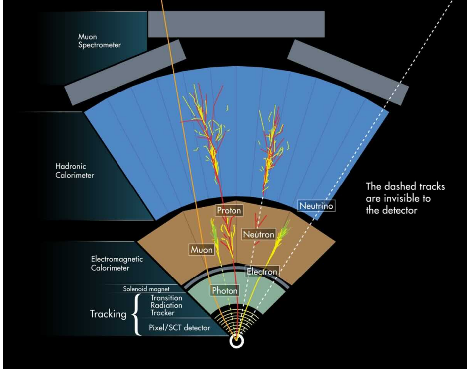
Figure 91: Particles traversing through the various subsystems of the ATLAS detector [94].
