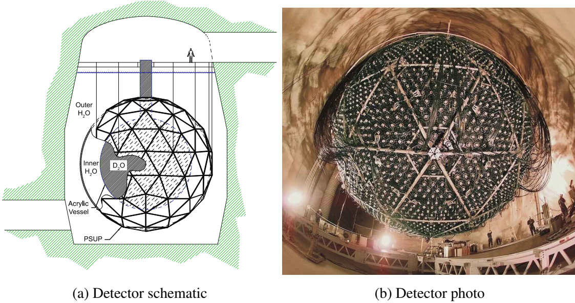
Figure 119: Sudbury Neutrino Observatory situated at Sudbury, Ontario, Canada. Images: Ref. [112], LBNL/R. Kaltschmidt
