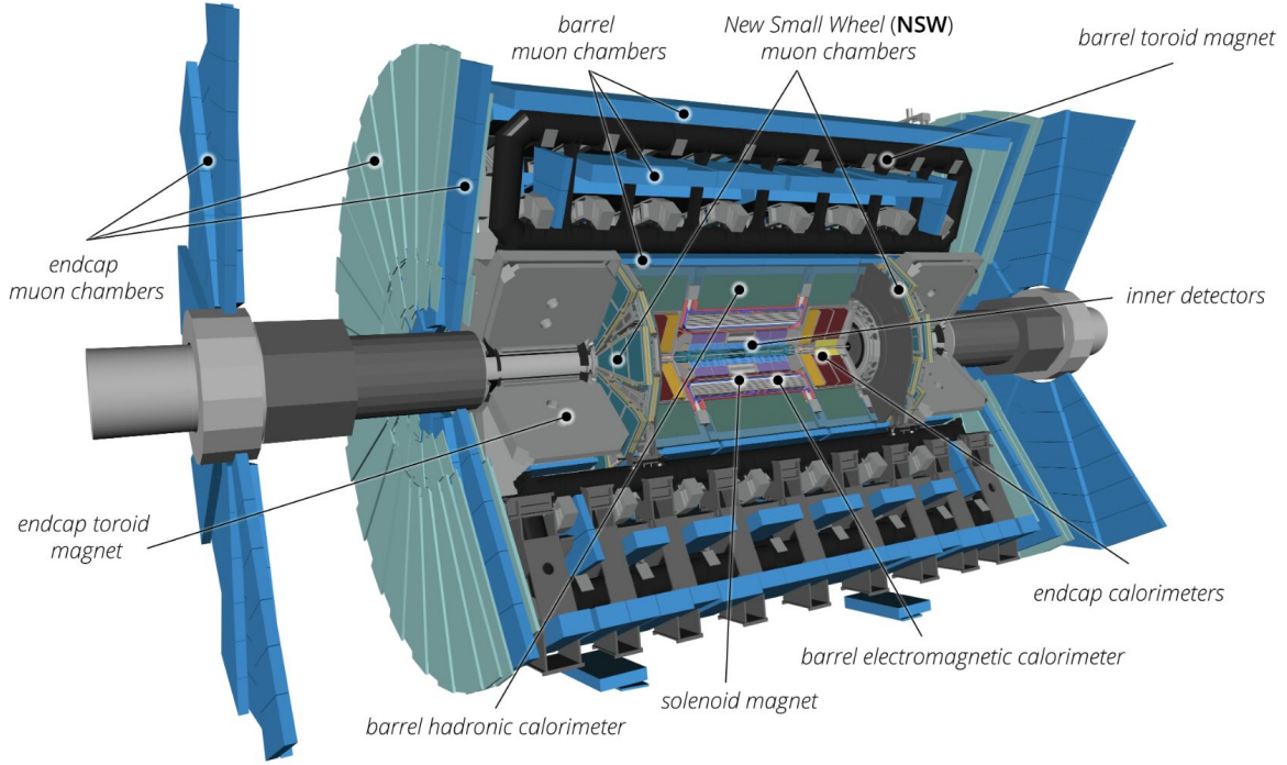
Figure 90: ATLAS Experiment layout. The components exemplifies a modern collider detector from Ref. [93].
