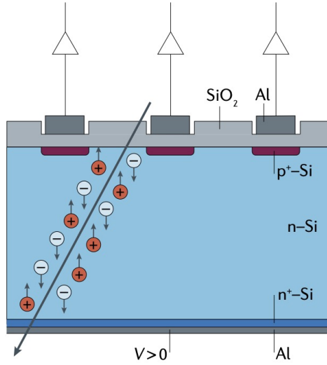
Figure 89: Silicon sensor schematic. This showing the principle of detection from Ref. [92].
