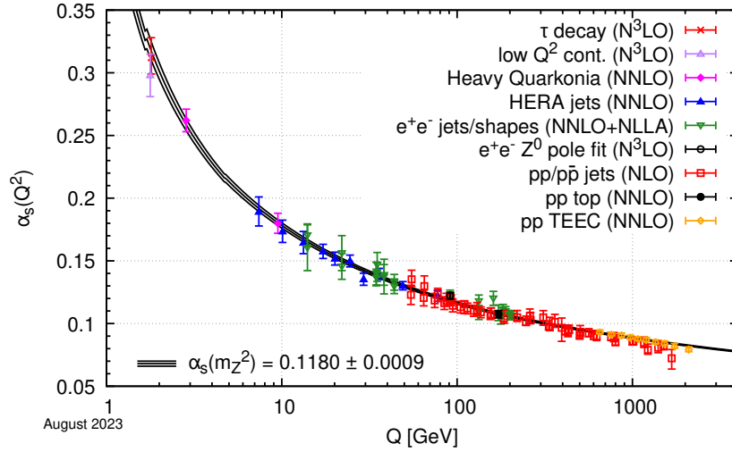
Figure 77: Running of strong coupling. Displayed is the strong coupling \alpha_s(Q^2) as a function of momentum transfer Q^2 from Ref. [76]. The measurements are performed using various probes, and the line shows the five-loop running taking \alpha_s(m_Z^2) = 0.1180 \pm 0.0009 as input.
