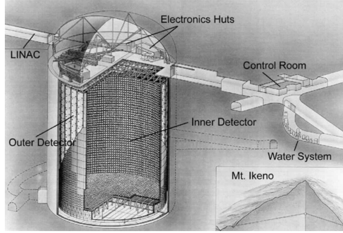
Figure 116: Super-Kamiokande detector situated in Mount Ikenoyama, Japan. Image: Ref. [108]
