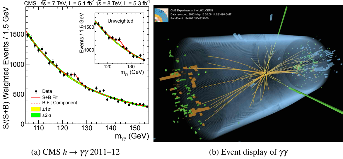
Figure 109: CMS Higgs boson discovery: diphoton channel. The original diphoton discovery data observed at the CMS Experiment using 2011–12 LHC data. Images: Ref. [101], CMS-PHO-EVENTS-2013-003.
