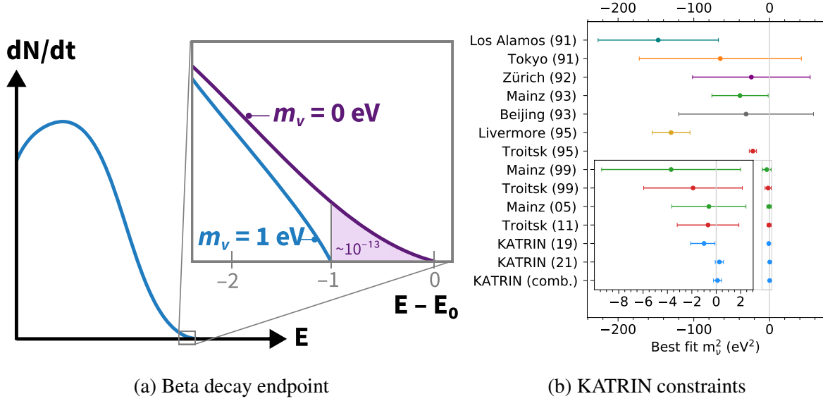
Figure 120: Beta decay spectrum for massless vs massive neutrinos. Only around 2 \times 10^{-13} of all decays reside in the last 1 eV. Right image: Ref. [113].
