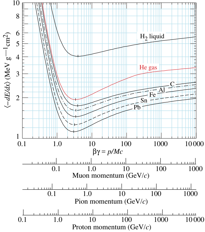
Figure 86: Particle stopping power by material. Stopping power dE/dx for muon and by material from Ref. [76].
