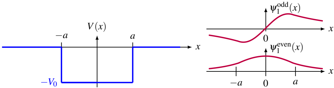
Figure 18: Left: finite-well potential. Right: sketch of first odd/even wavefunctions, which ‘leak’ outside the well |x| > a in striking difference from classical particles in a box.
