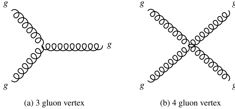
Figure 74: Gluon self-interaction vertices due to the non-Abelian structure of quantum chromodynamics.
