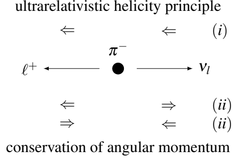
(b) Helicity of pion decay
