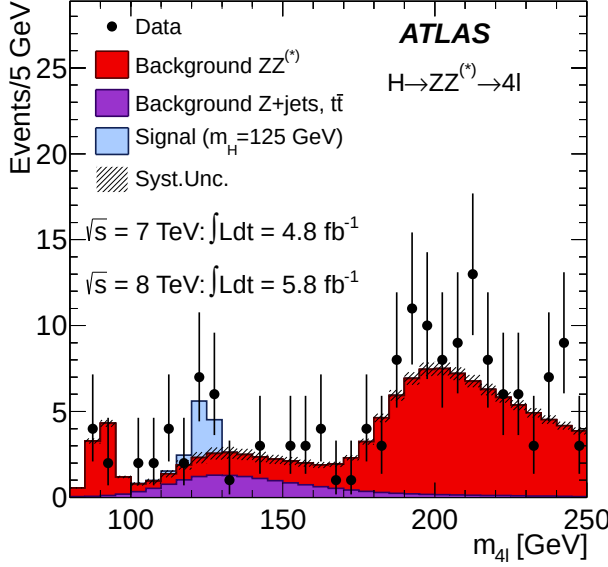
(a) ATLAS h \rightarrow 4\ell 2011–12
