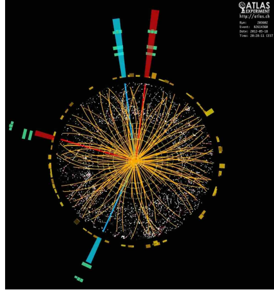
(b) Event display of 2e2\mu
