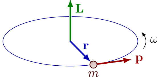
Figure 29: Visualization of orbital angular momentum \mathbf{L} . Figure: Izaak Neutelings .
