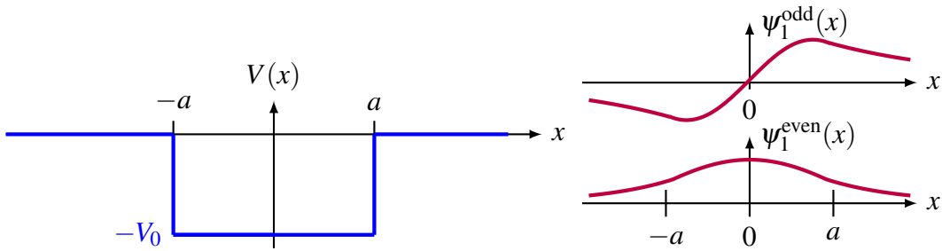
Figure 18: Finite-well potential (left) and sketch of first odd/even wavefunctions (right).
