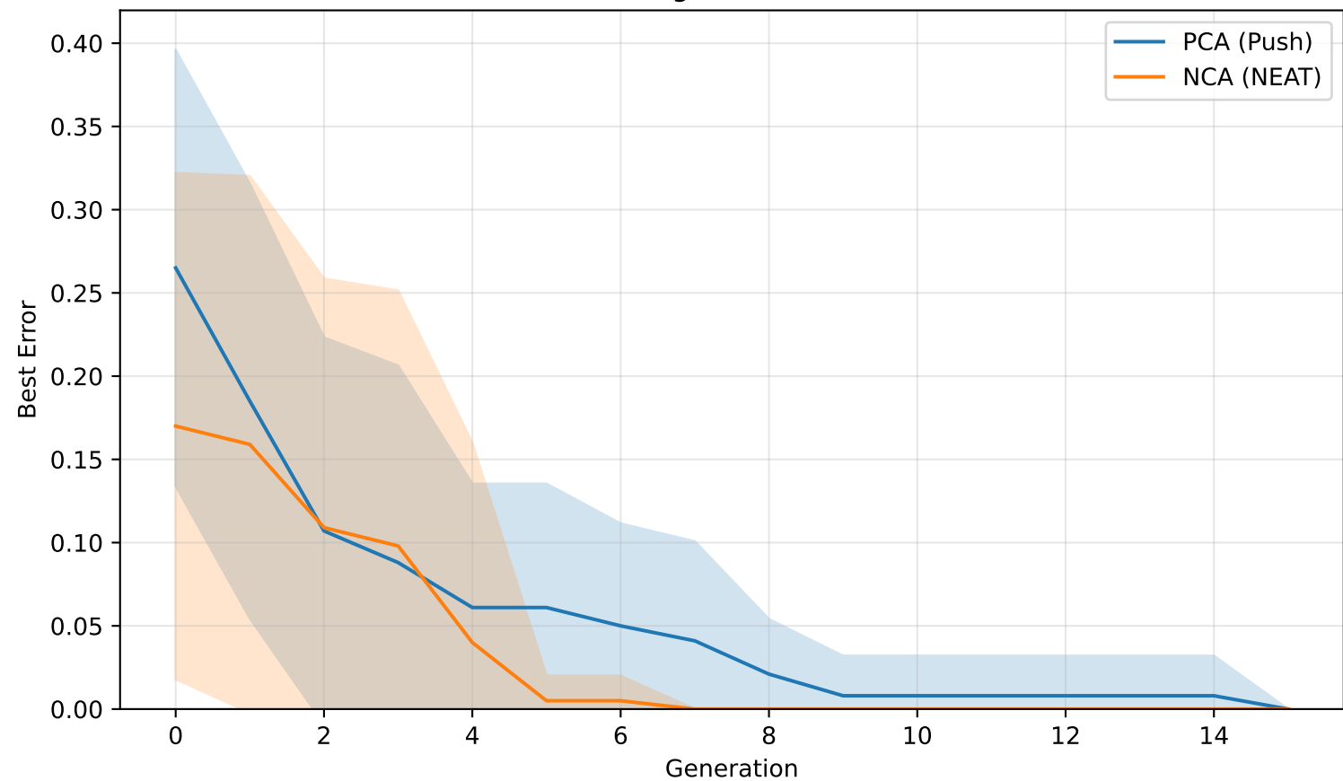
Error Convergence: checkerboard
