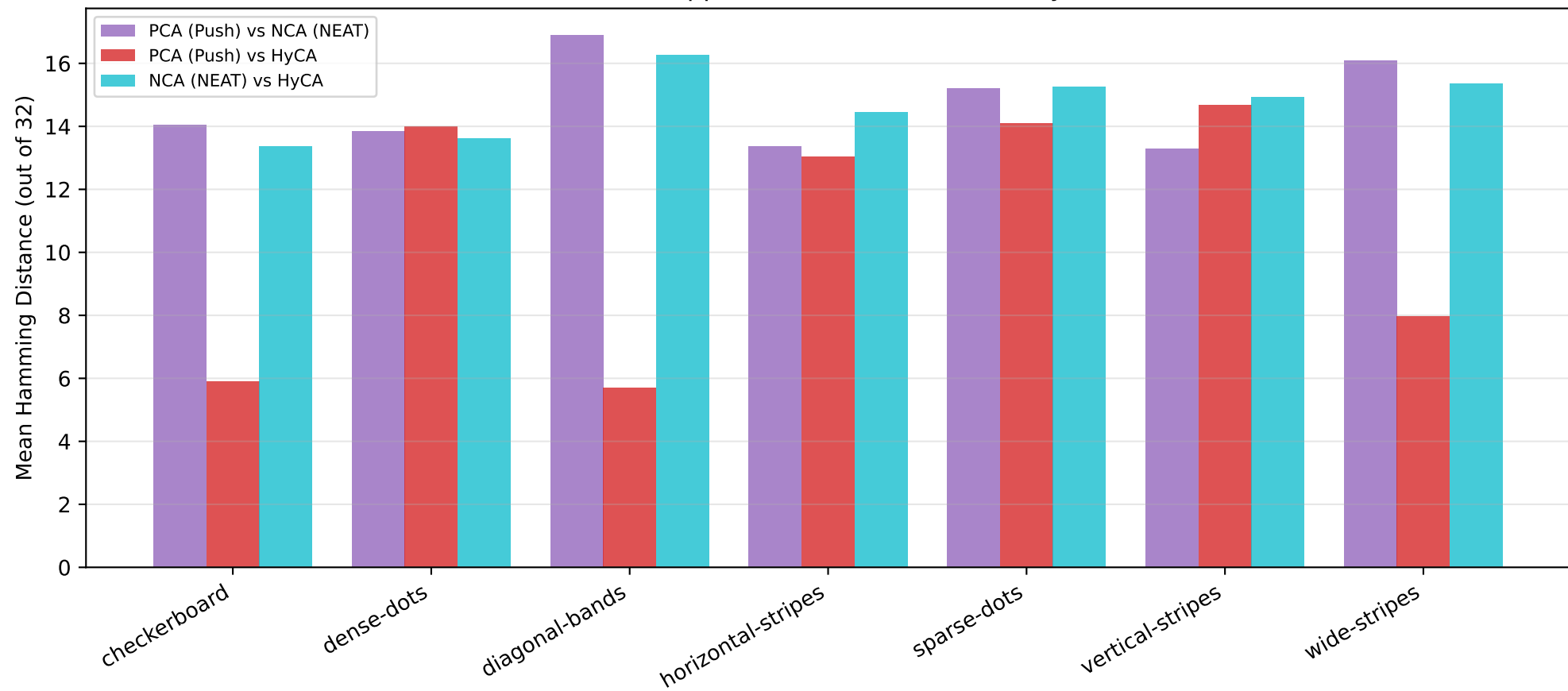
Cross-Approach Truth Table Similarity
