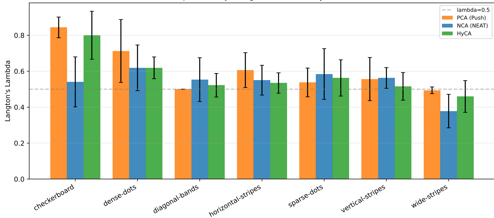
Output Density (Langton's Lambda) by Pattern
