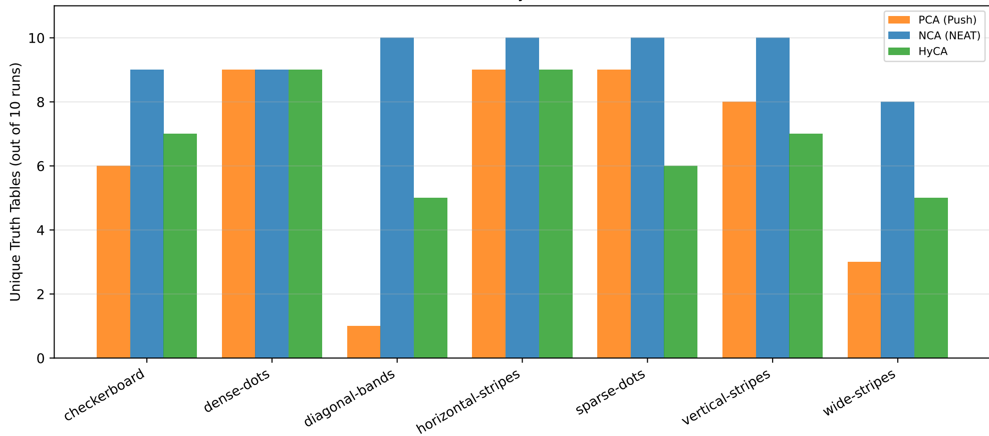
Rule Diversity Across Runs
