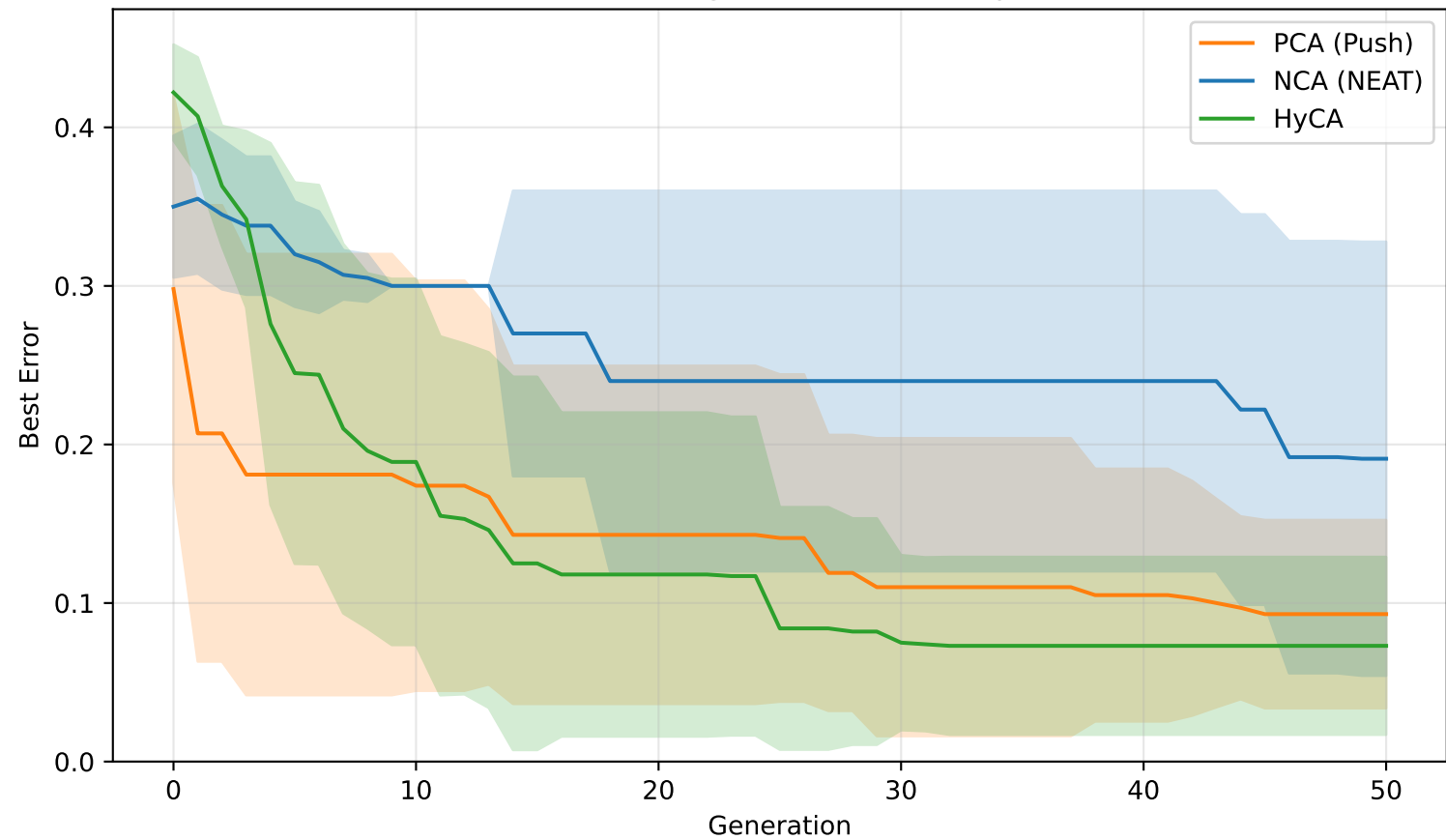
Error Convergence: vertical-stripes
