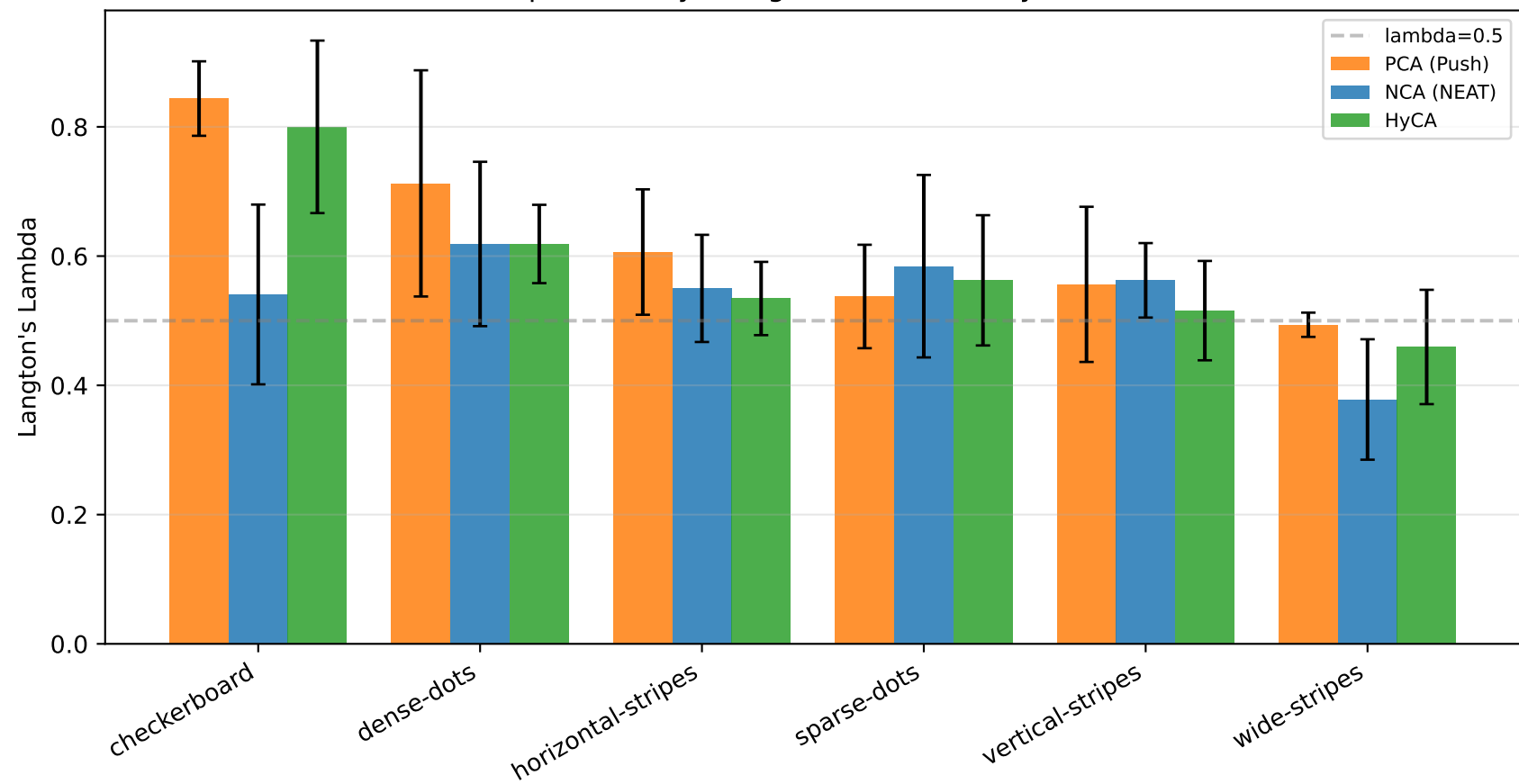
Output Density (Langton's Lambda) by Pattern
