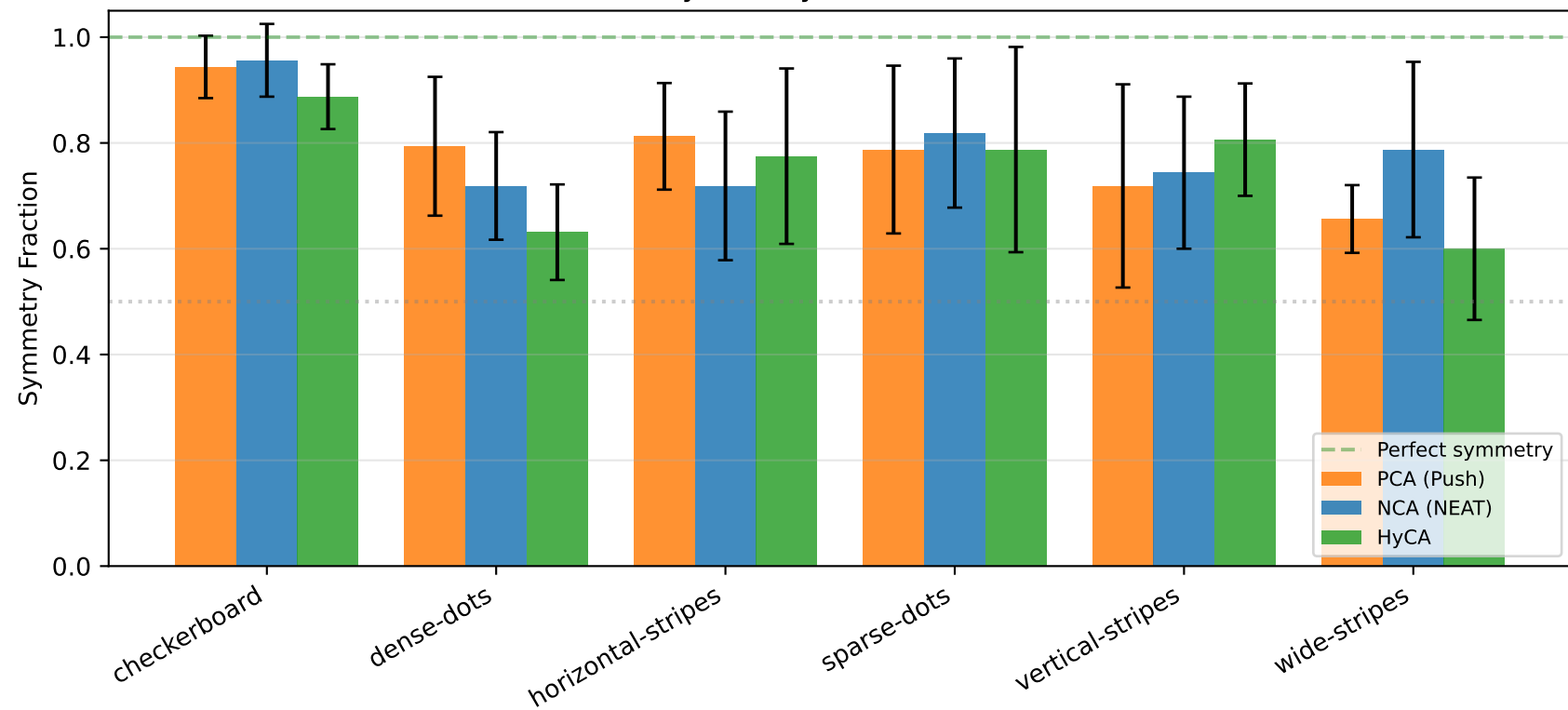
Reflection Symmetry: North-South ( N2 \leftrightarrow N4 )
