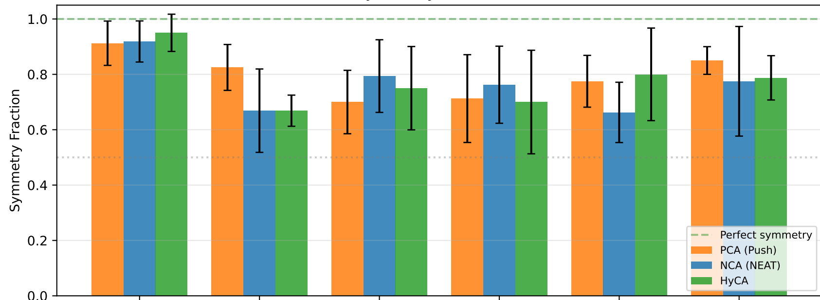
Reflection Symmetry: East-West ( N1 \leftrightarrow N3 )
