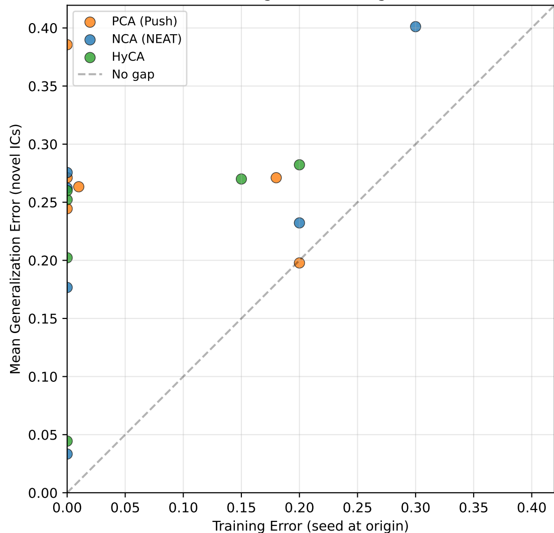
Best-Generalizing Rule: Training vs Test Error
