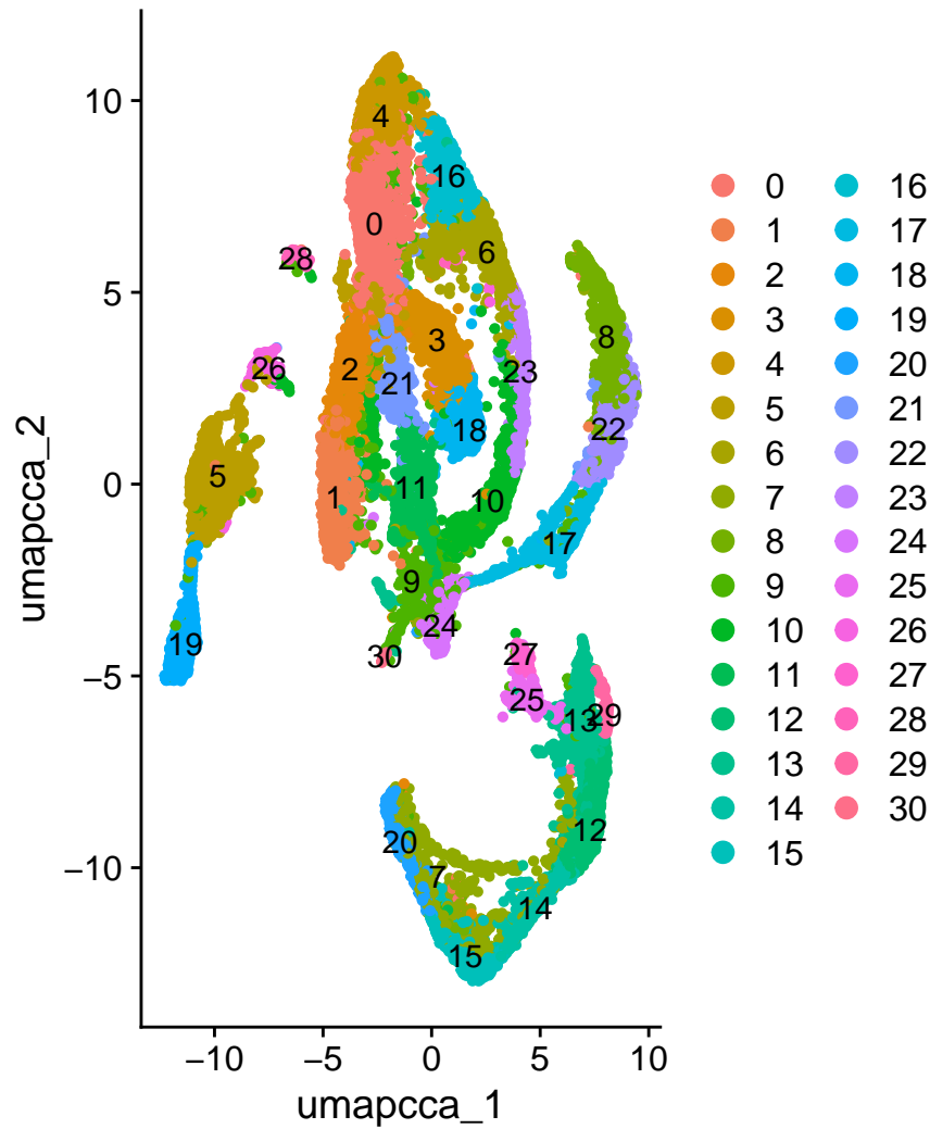
cca_clusters
