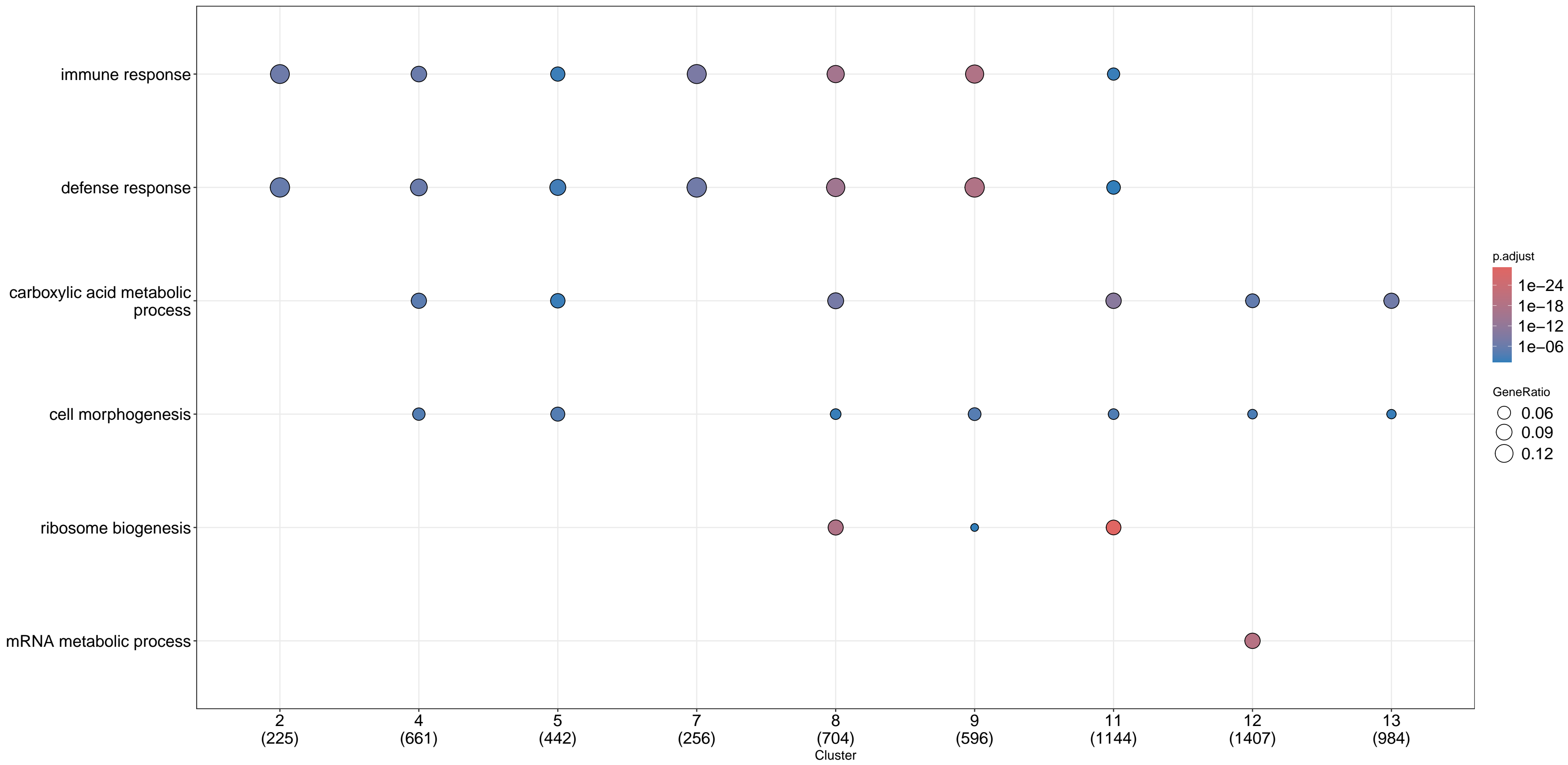
GO Enrichment (Biological Process)
