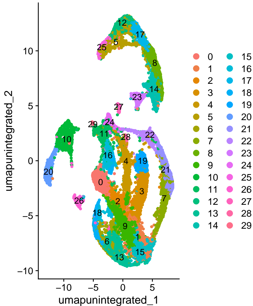
unintegrated_clusters
