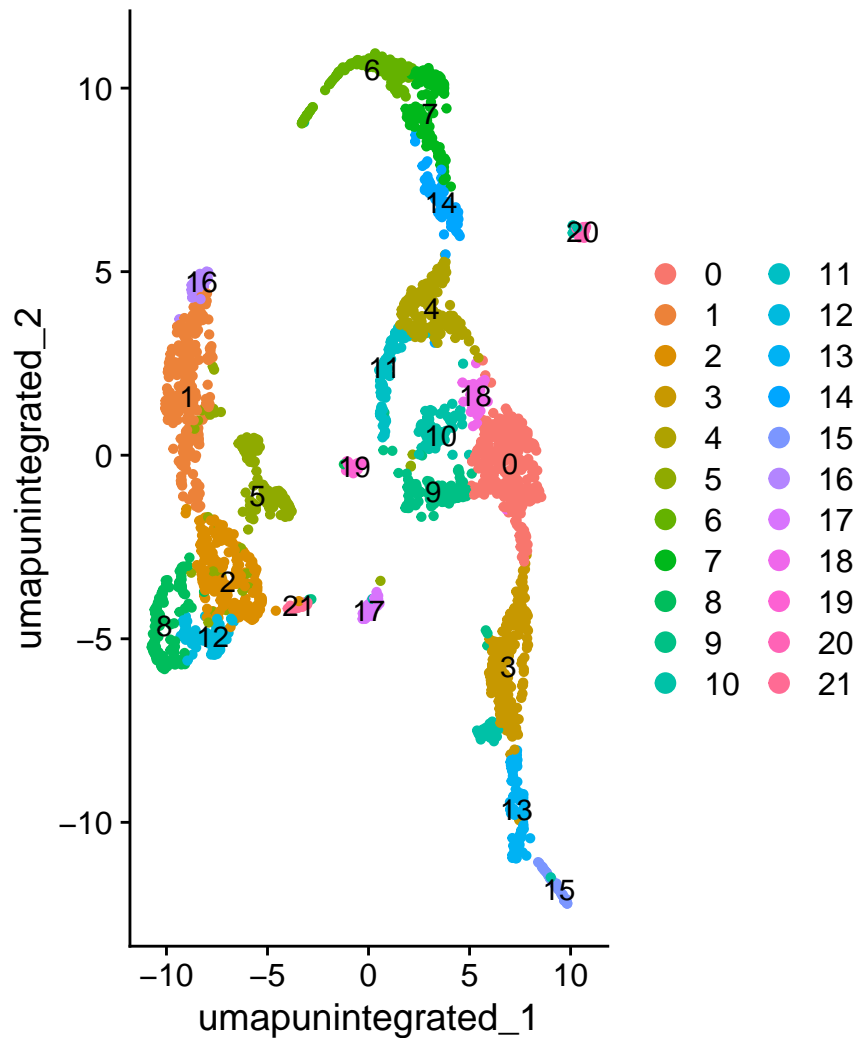
unintegrated_clusters
