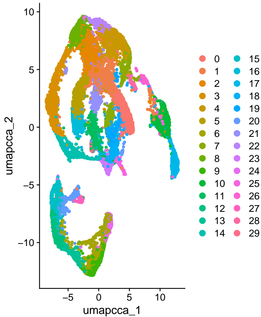
cca_clusters
