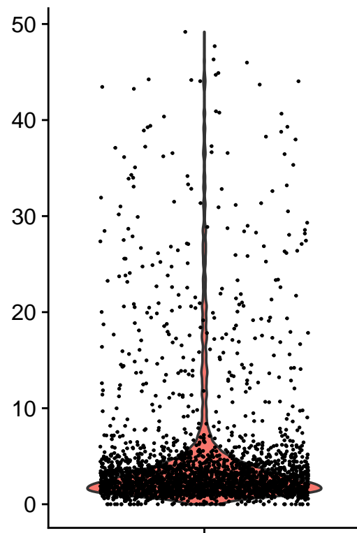
percent.mt
