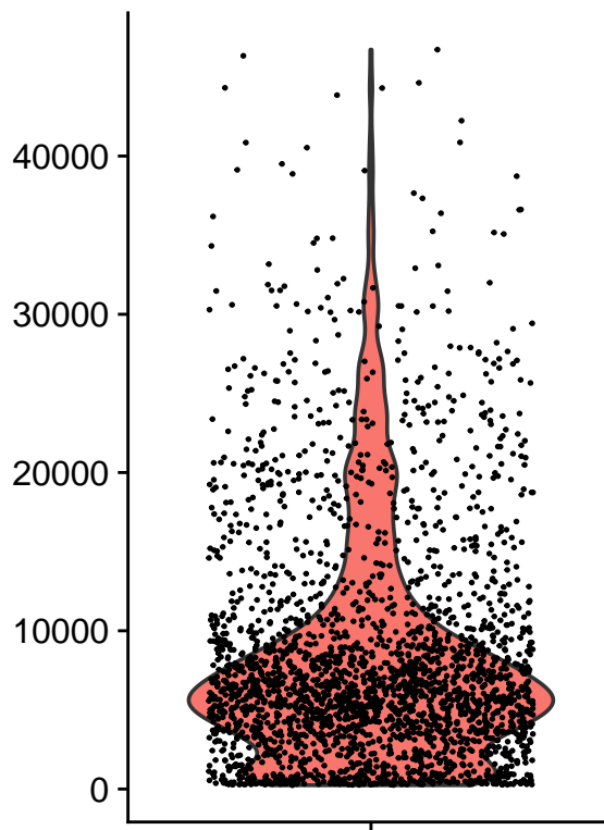
nCount_RNA
