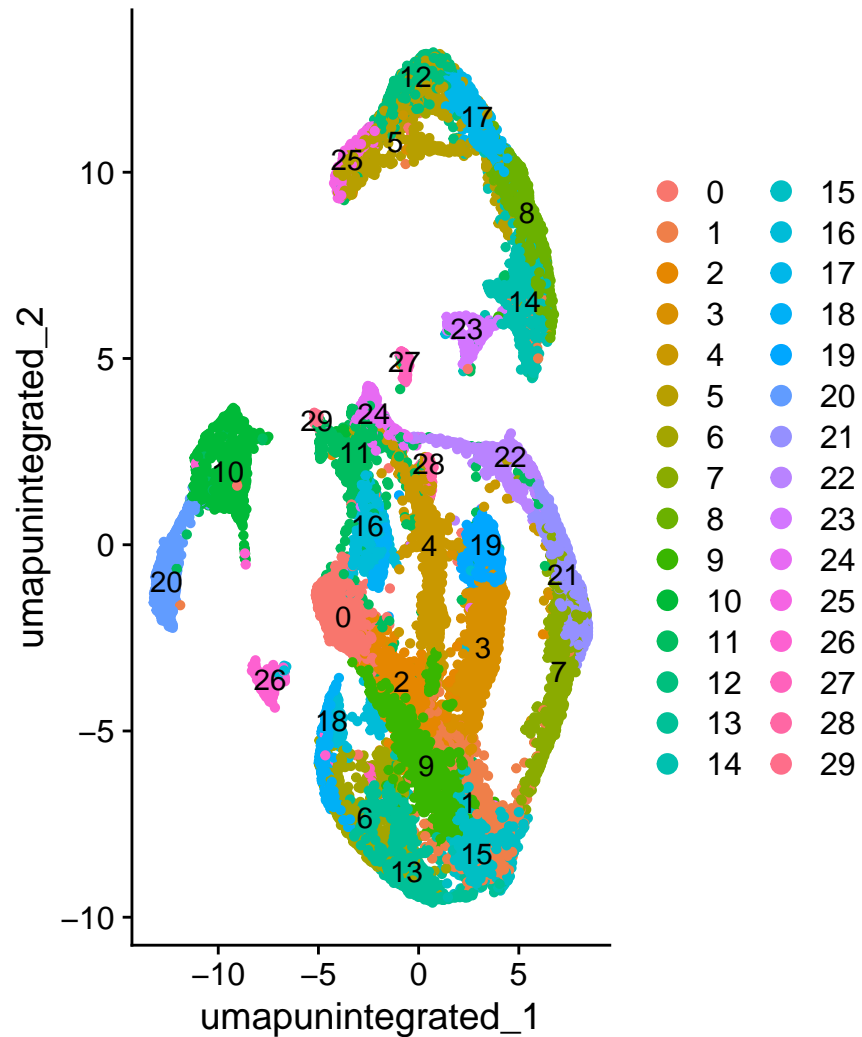
unintegrated_clusters
