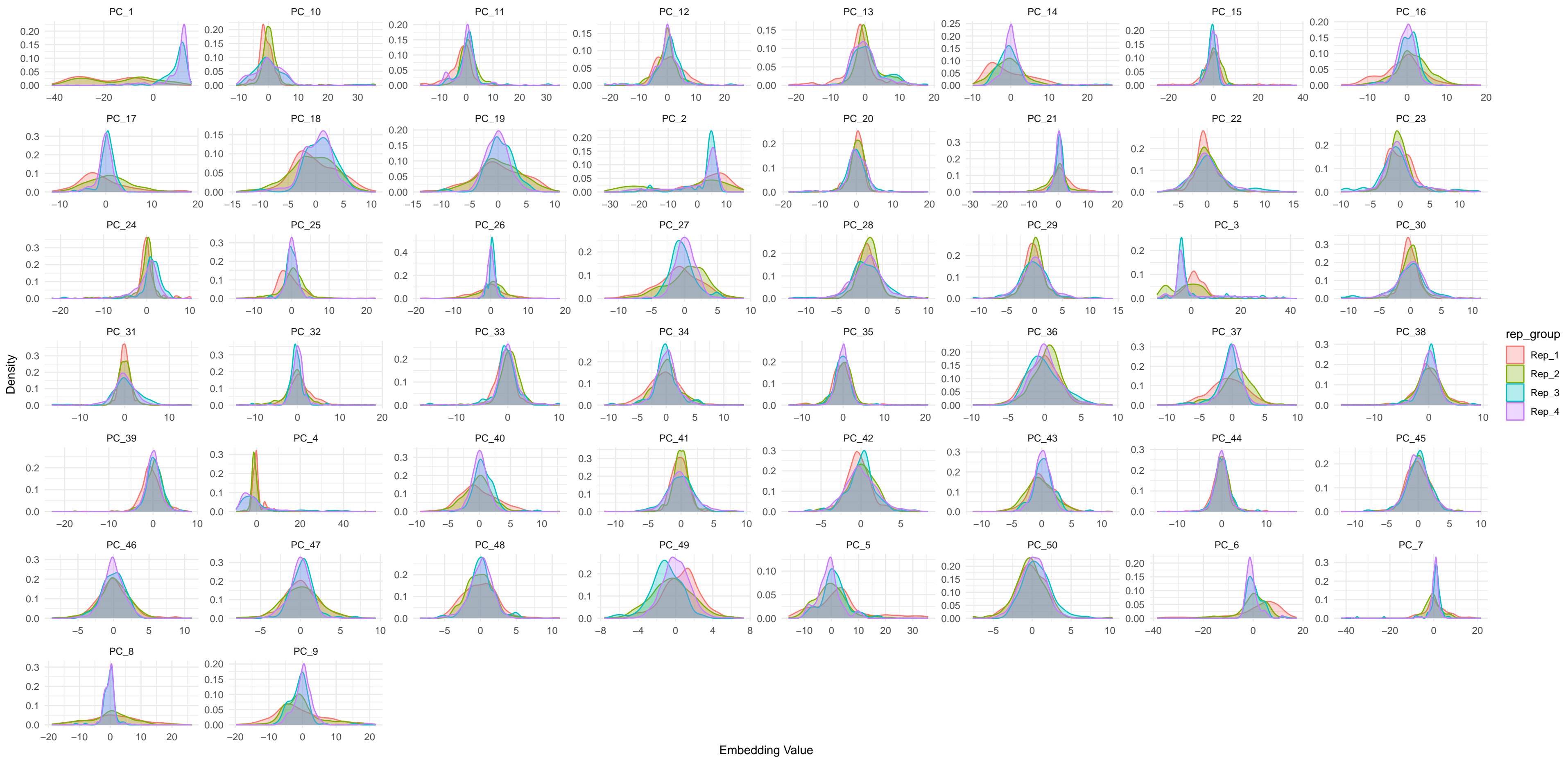
Density of Harmony components by replicate group
