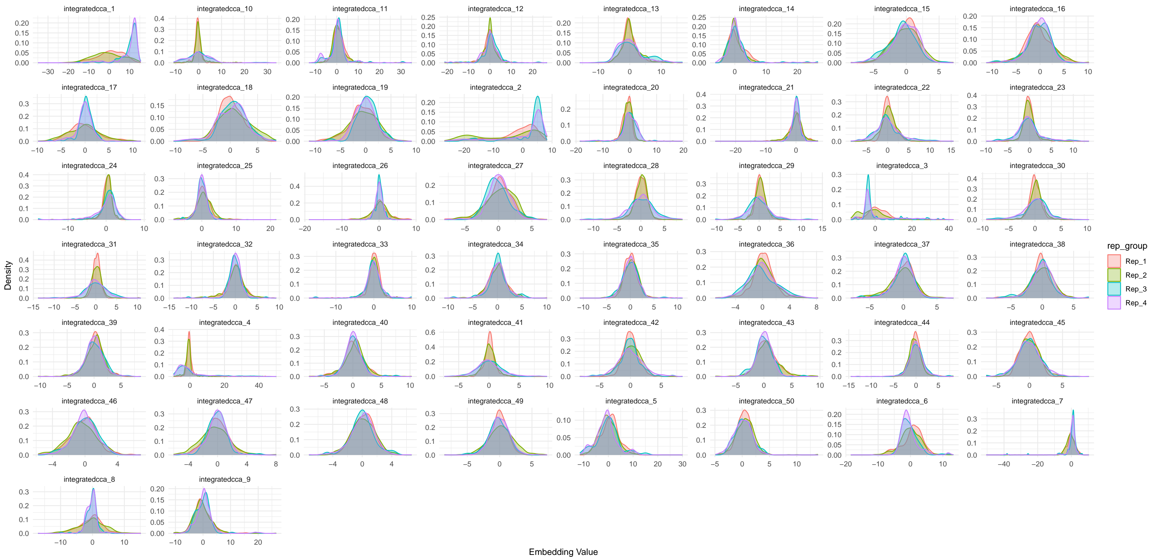
Density of CCA components by replicate group
