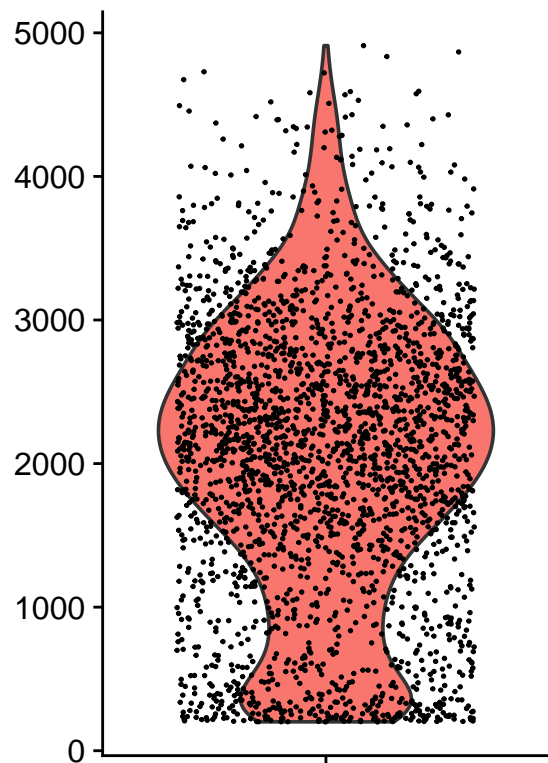
nFeature_RNA
