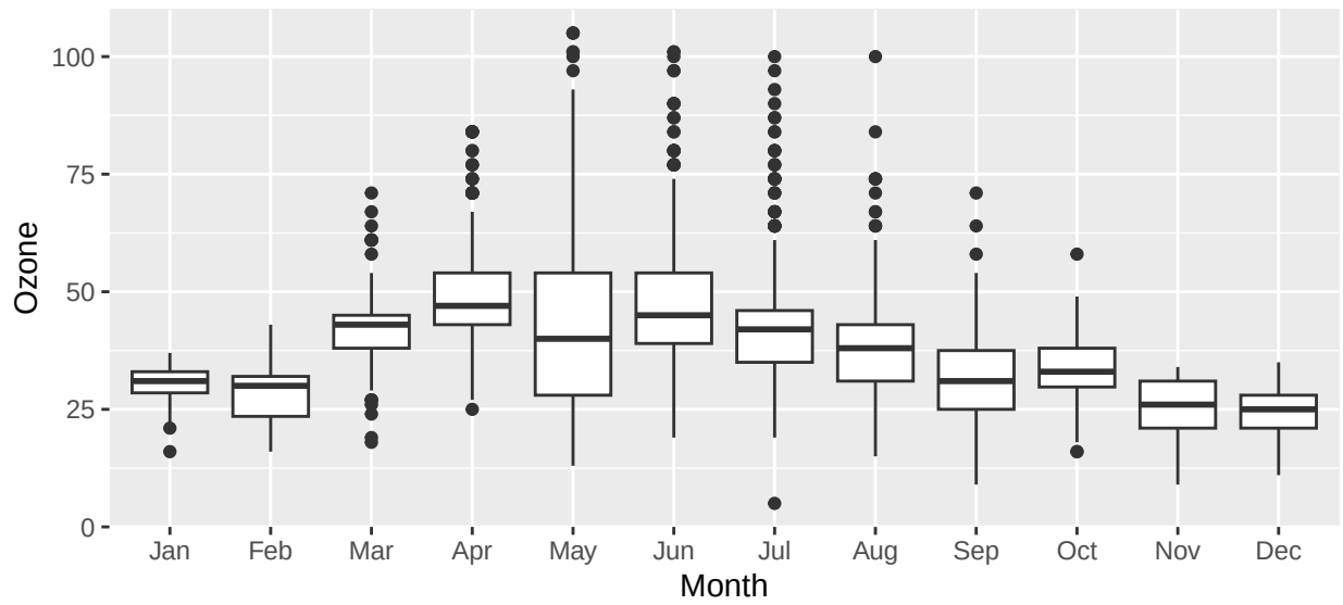
Figure 1: Ozone distribution by month (2018).
