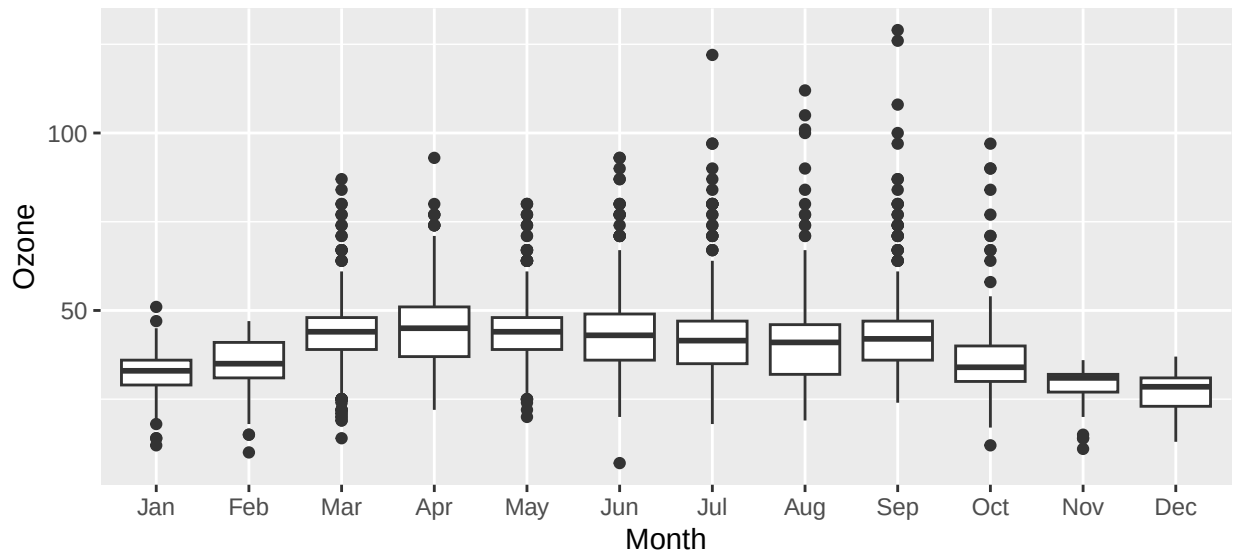
Figure 2: Ozone distribution by month (2019).
