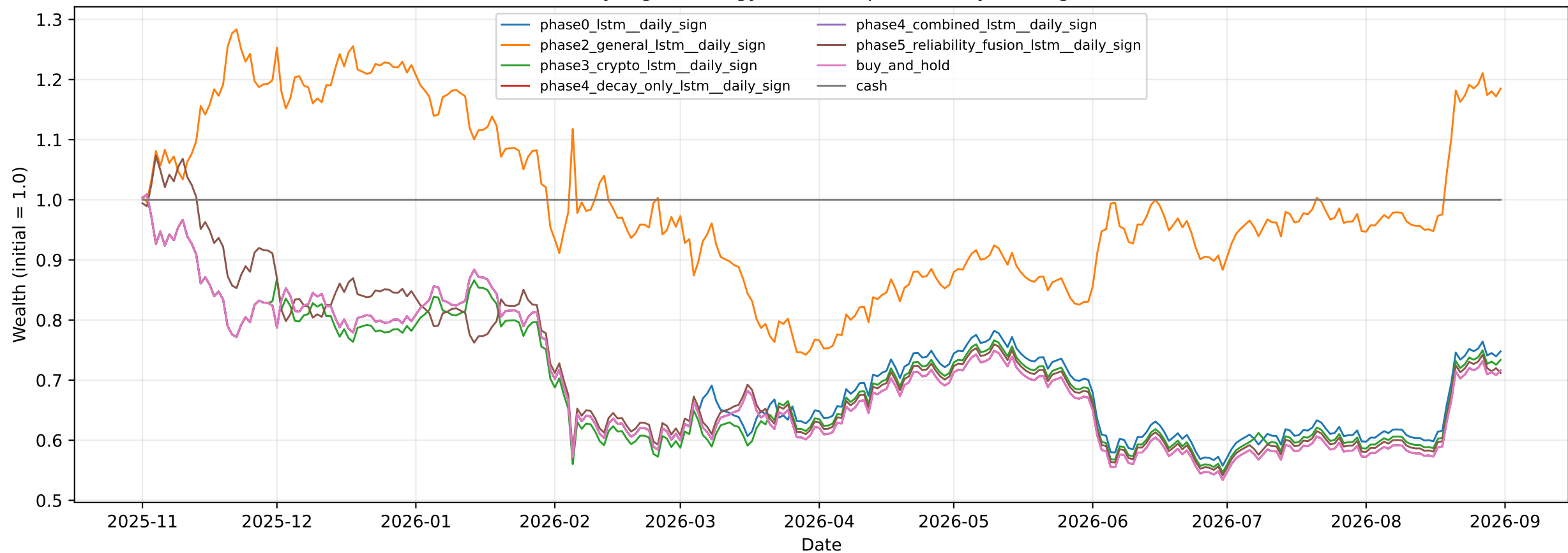
BTC: Daily-Sign Strategy after 10 bps One-Way Trading Costs
