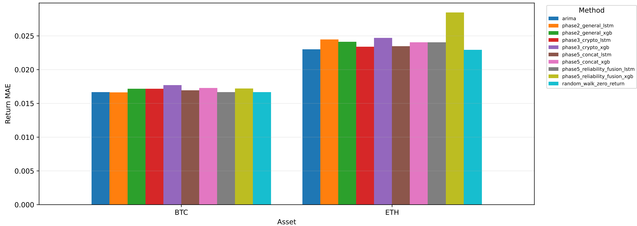
Held-Out Test Return MAE
