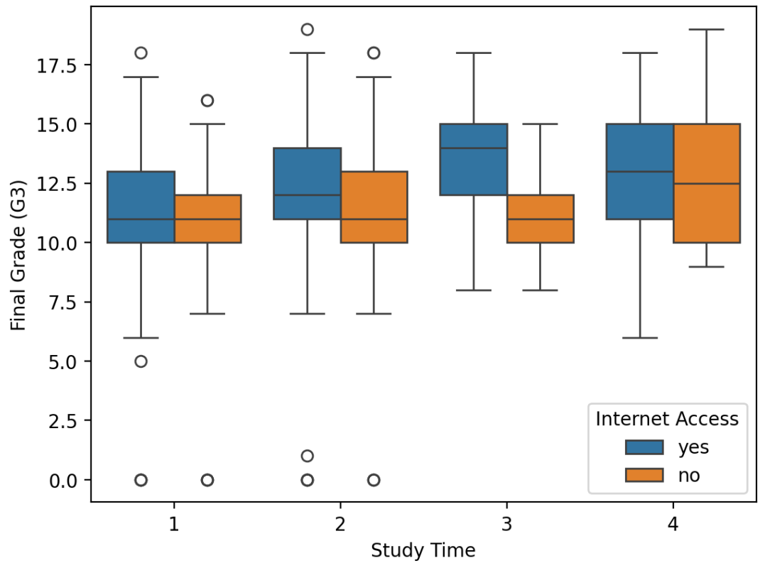
Grade Distribution for Sex = M
